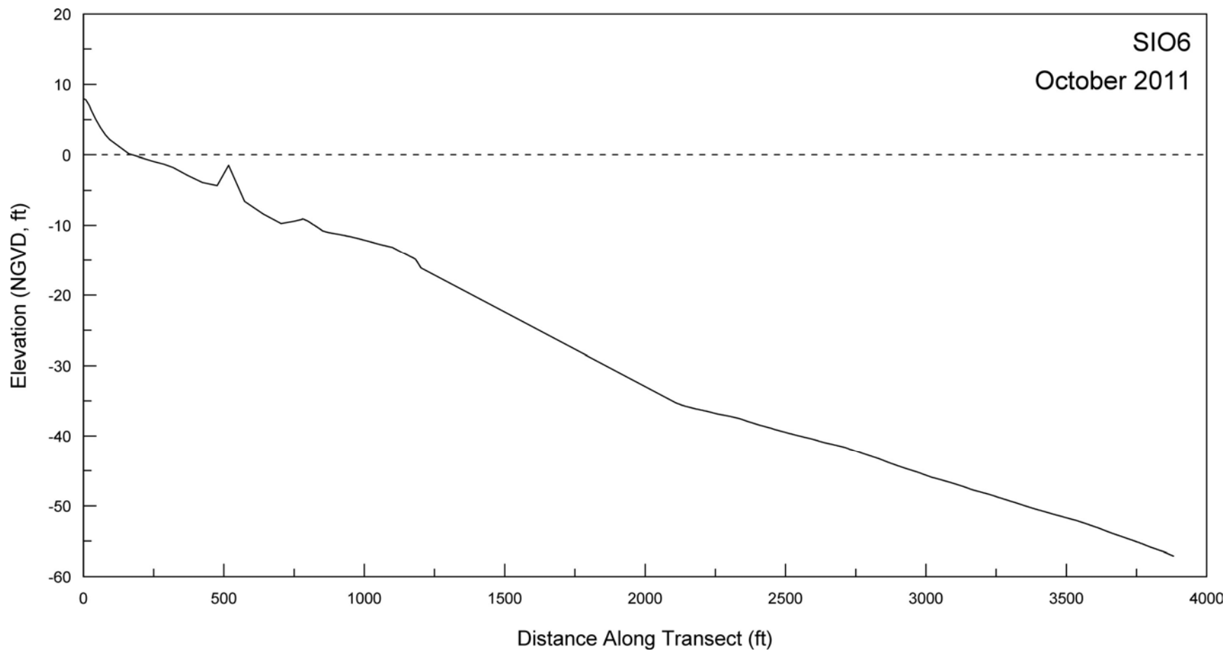
Figure A-4. Beach profile for SIO6 surveyed on 4 October 2011.
