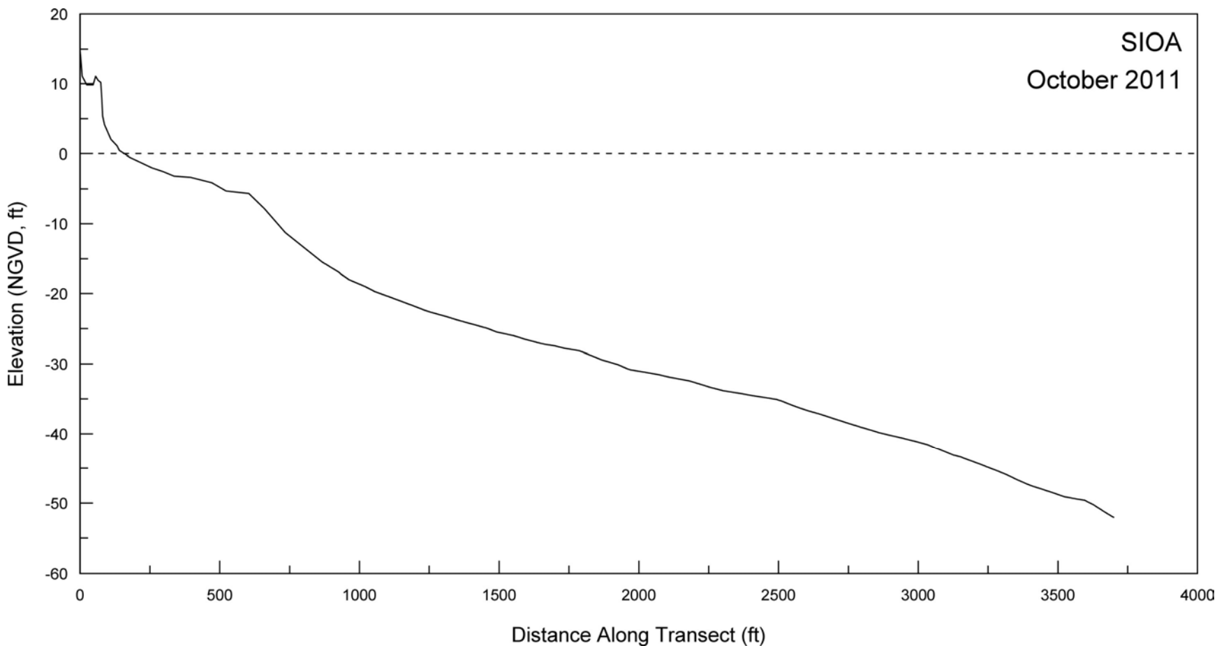
Figure A-5. Beach profile for SIOA surveyed on 4 October 2011.
