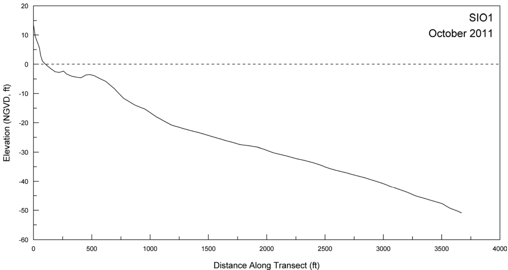
Figure A-1. Beach profile for SIO1 surveyed on 4 October 2011.
