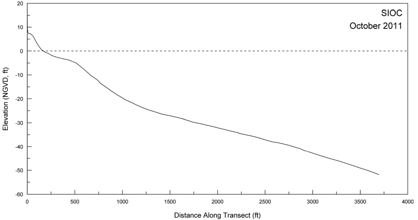
Figure A-7. Beach profile for SIOC surveyed on 4 October 2011.
