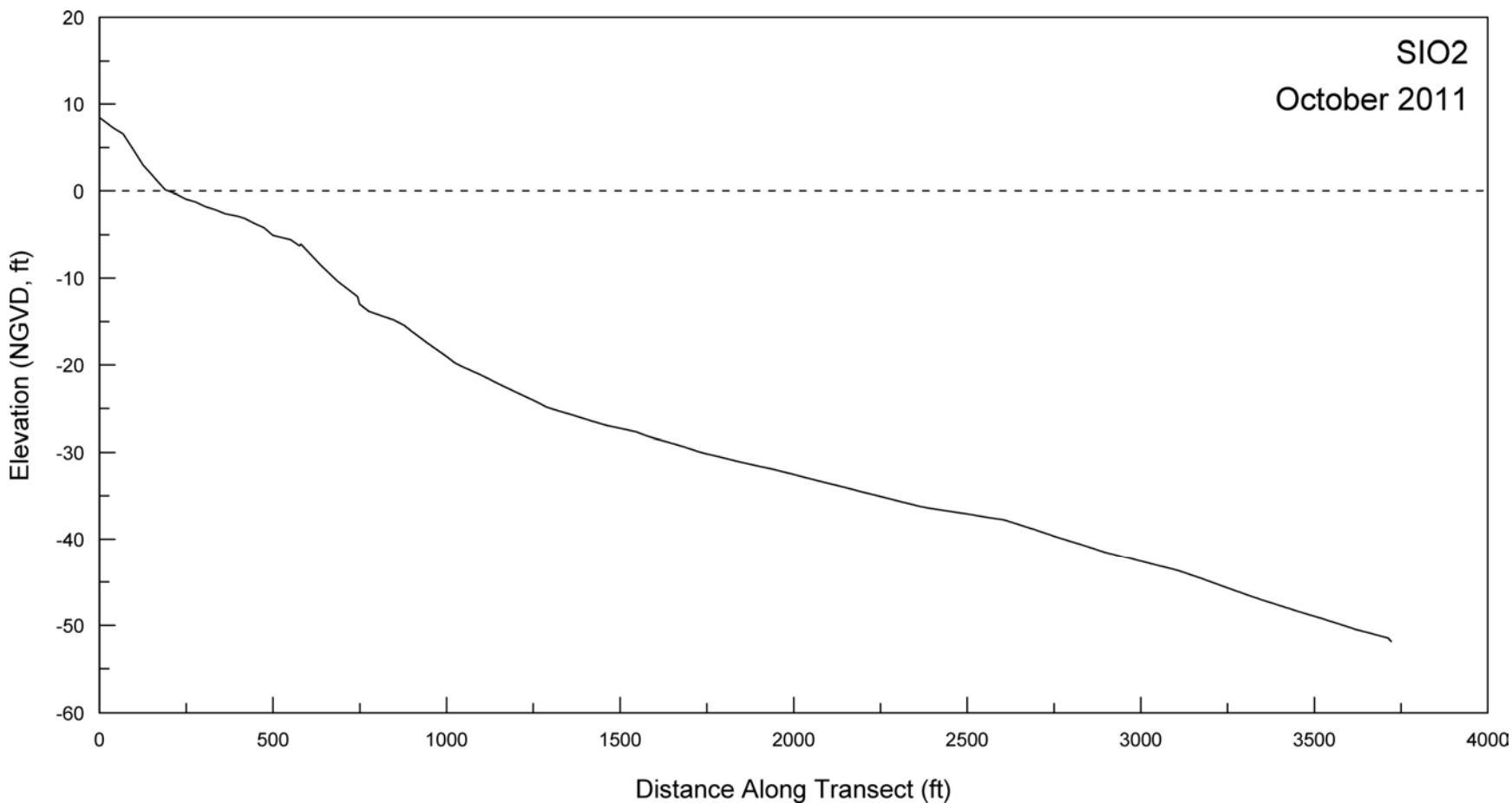
Figure A-2. Beach profile for SIO2 surveyed on 4 October 2011.
