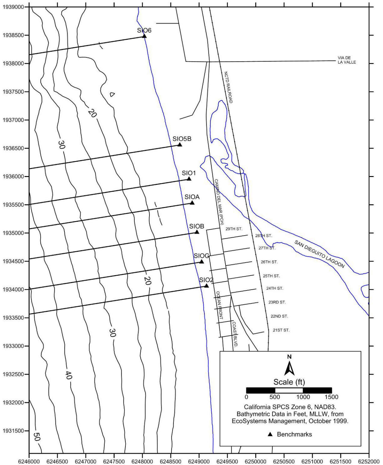
Figure 2. Beach profiles surveyed on 4 October 2011.
