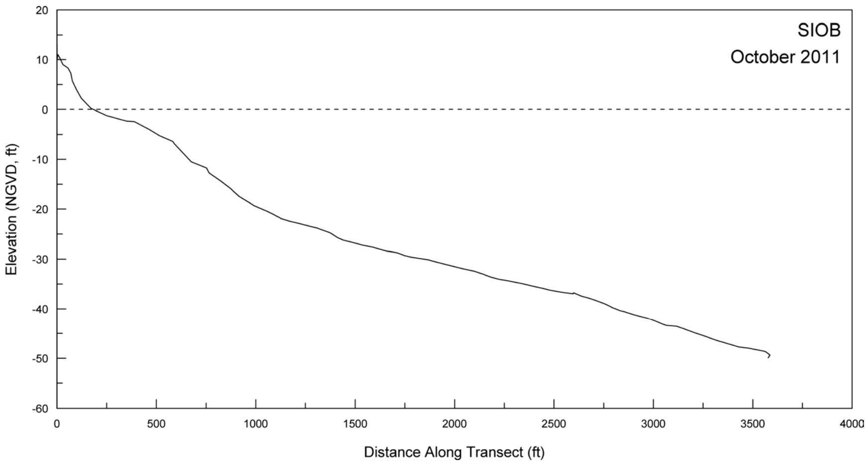
Figure A-6. Beach profile for SIOB surveyed on 4 October 2011.
