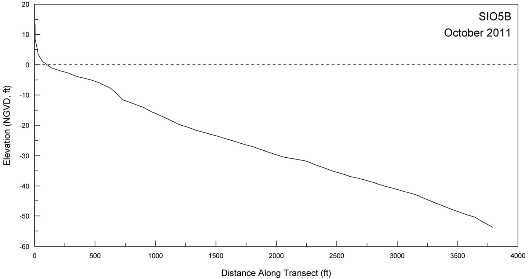
Figure A-3. Beach profile for SIO5B surveyed on 4 October 2011.
