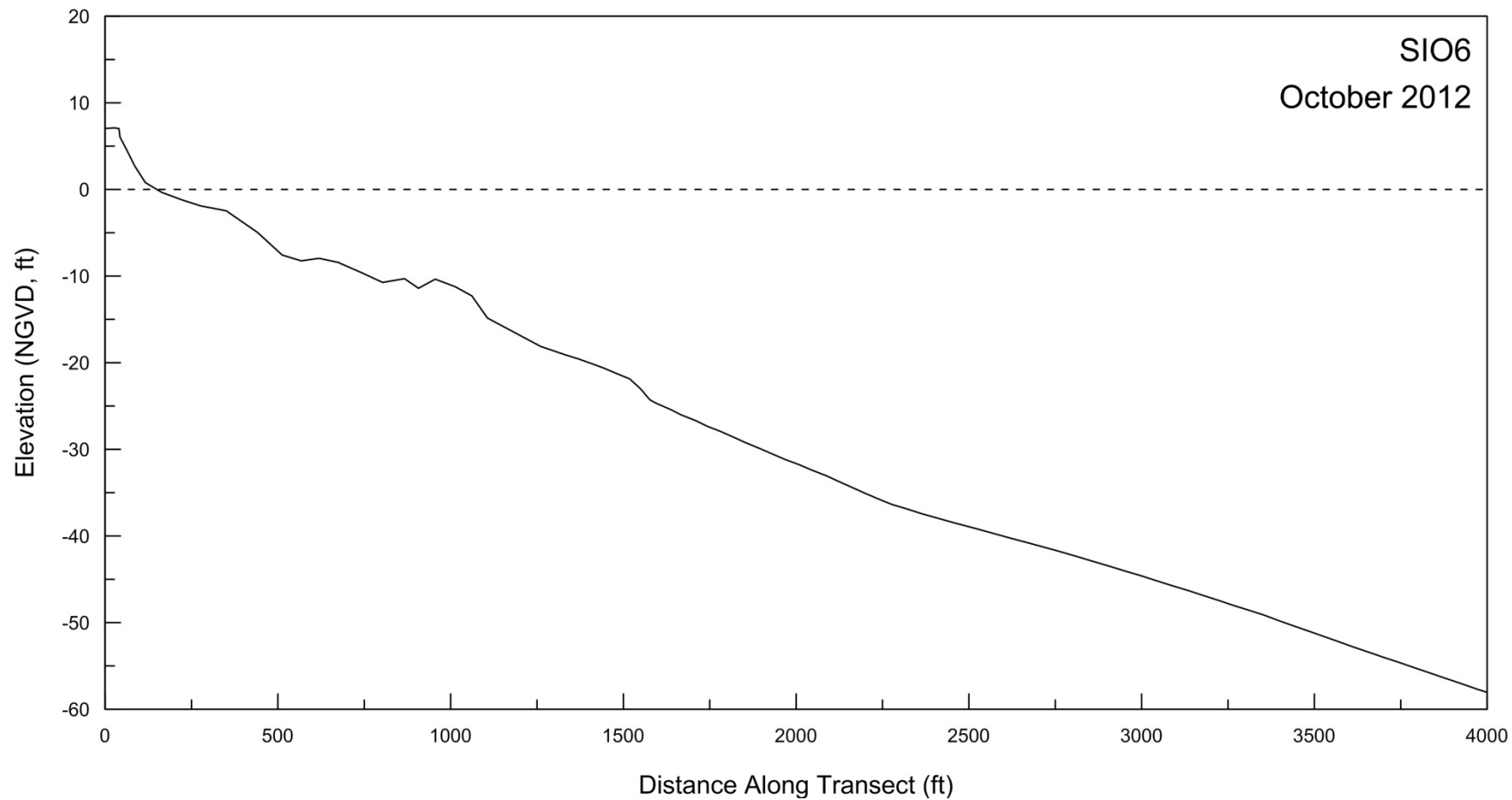
Figure A-4. Beach profile for SIO6 surveyed on 9 October 2012.
