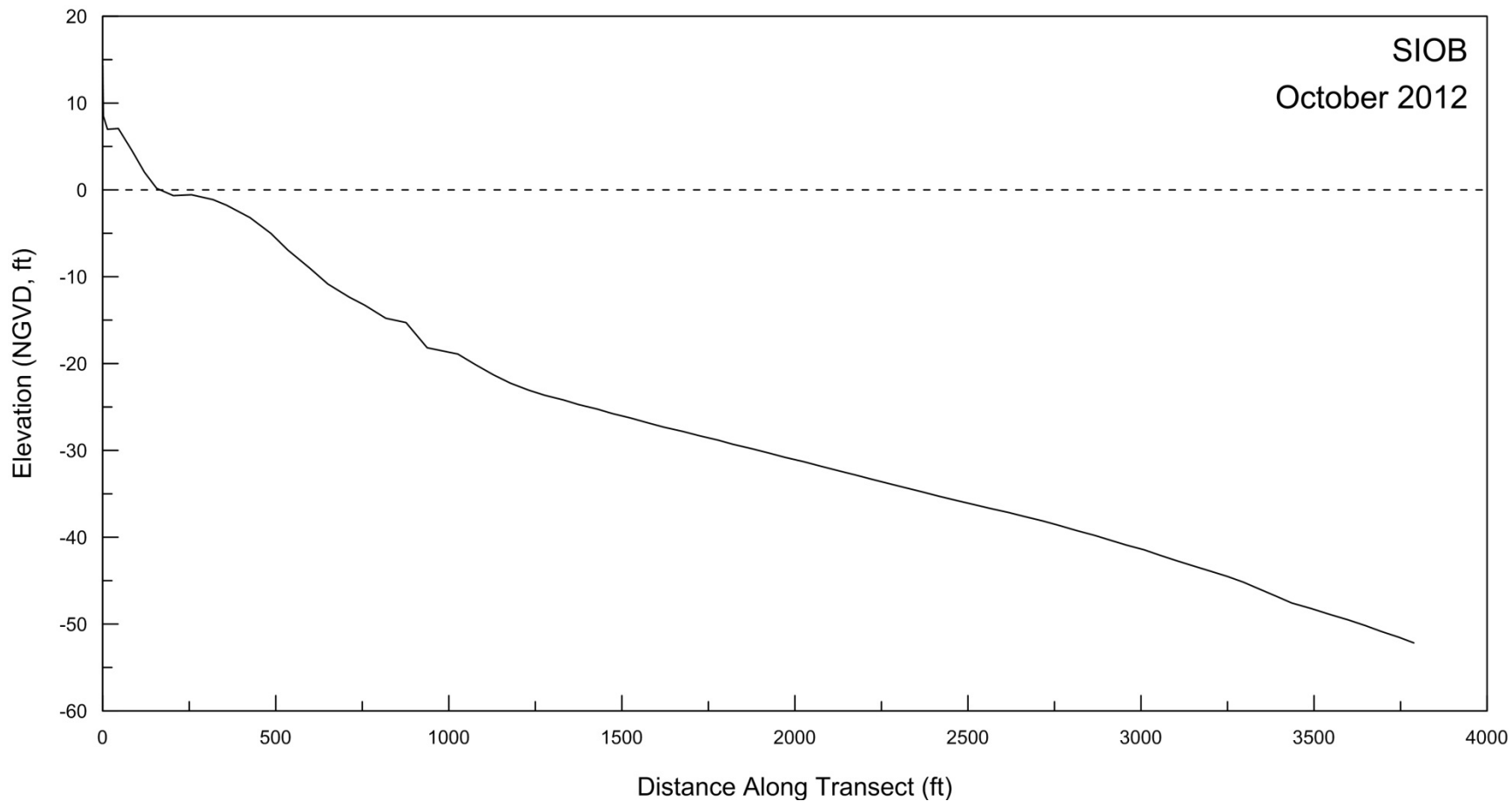
Figure A-6. Beach profile for SIOB surveyed on 9 October 2012.
