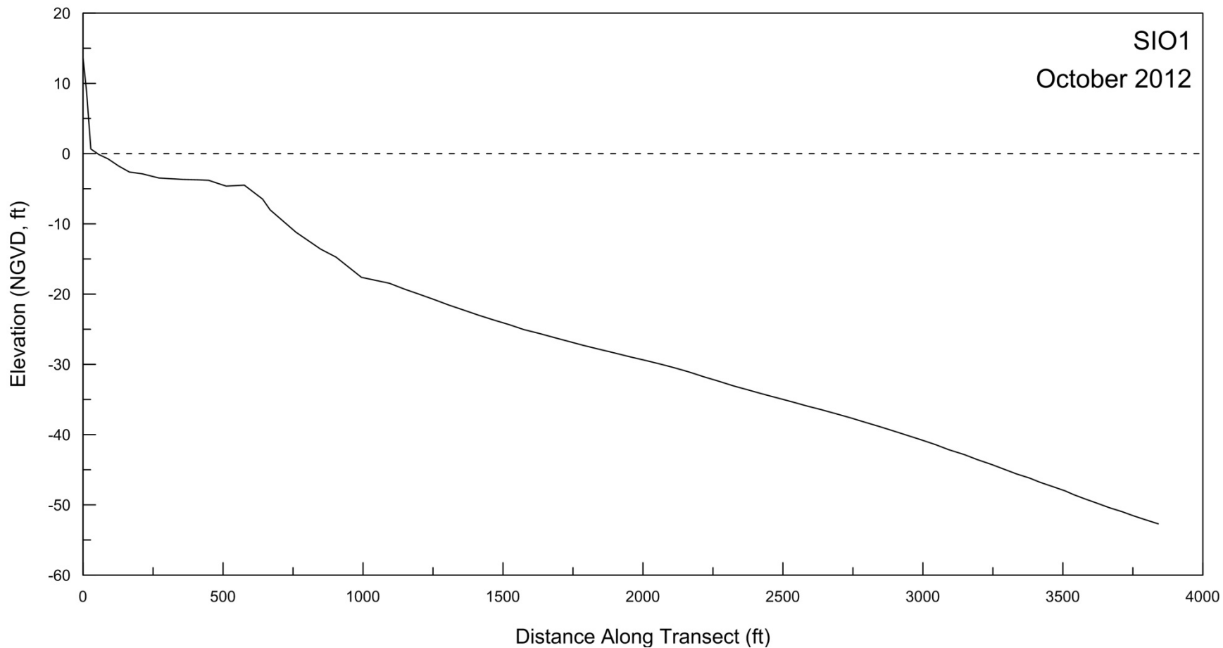
Figure A-1. Beach profile for SIO1 surveyed on 9 October 2012.
