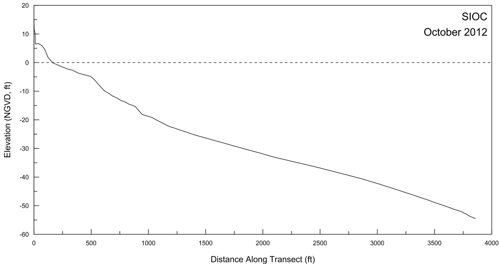
Figure A-7. Beach profile for SIOC surveyed on 9 October 2012.
