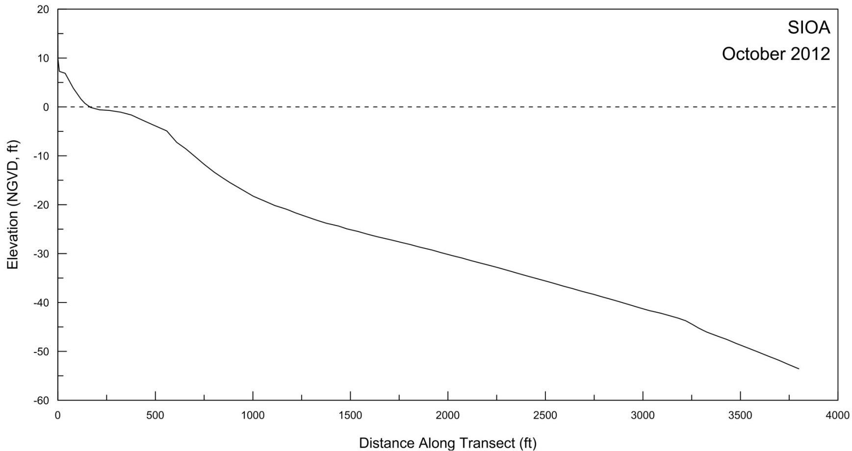
Figure A-5. Beach profile for SIOA surveyed on 9 October 2012.
