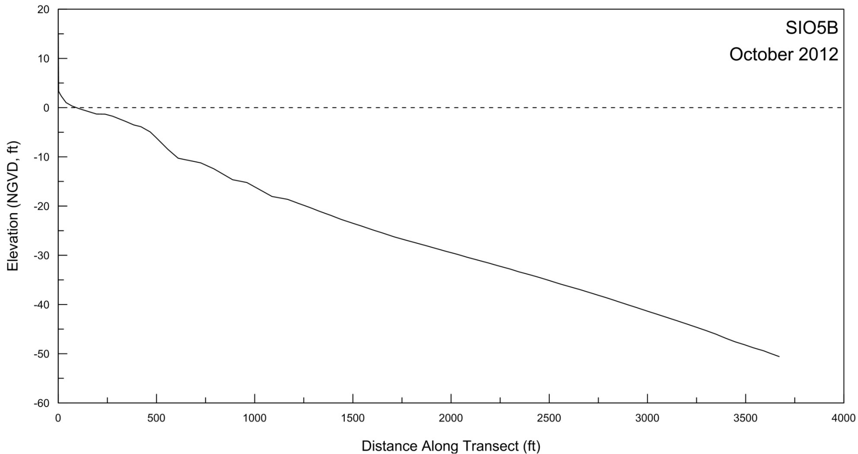
Figure A-3. Beach profile for SIO5B surveyed on 9 October 2012.
