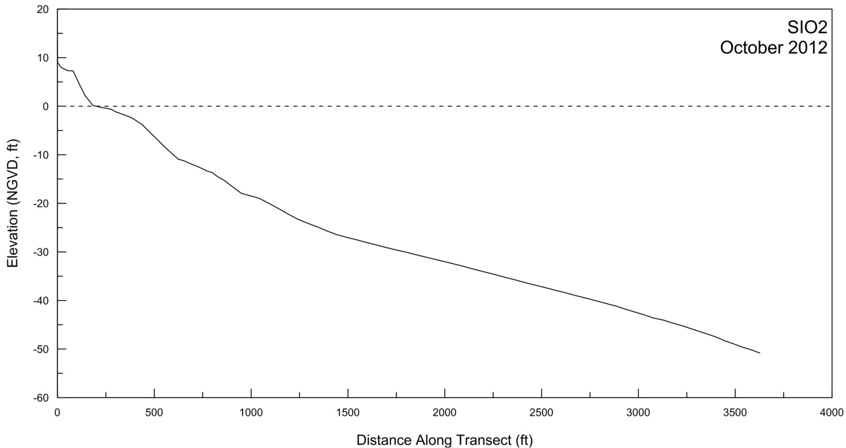
Figure A-2. Beach profile for SIO2 surveyed on 9 October 2012.
