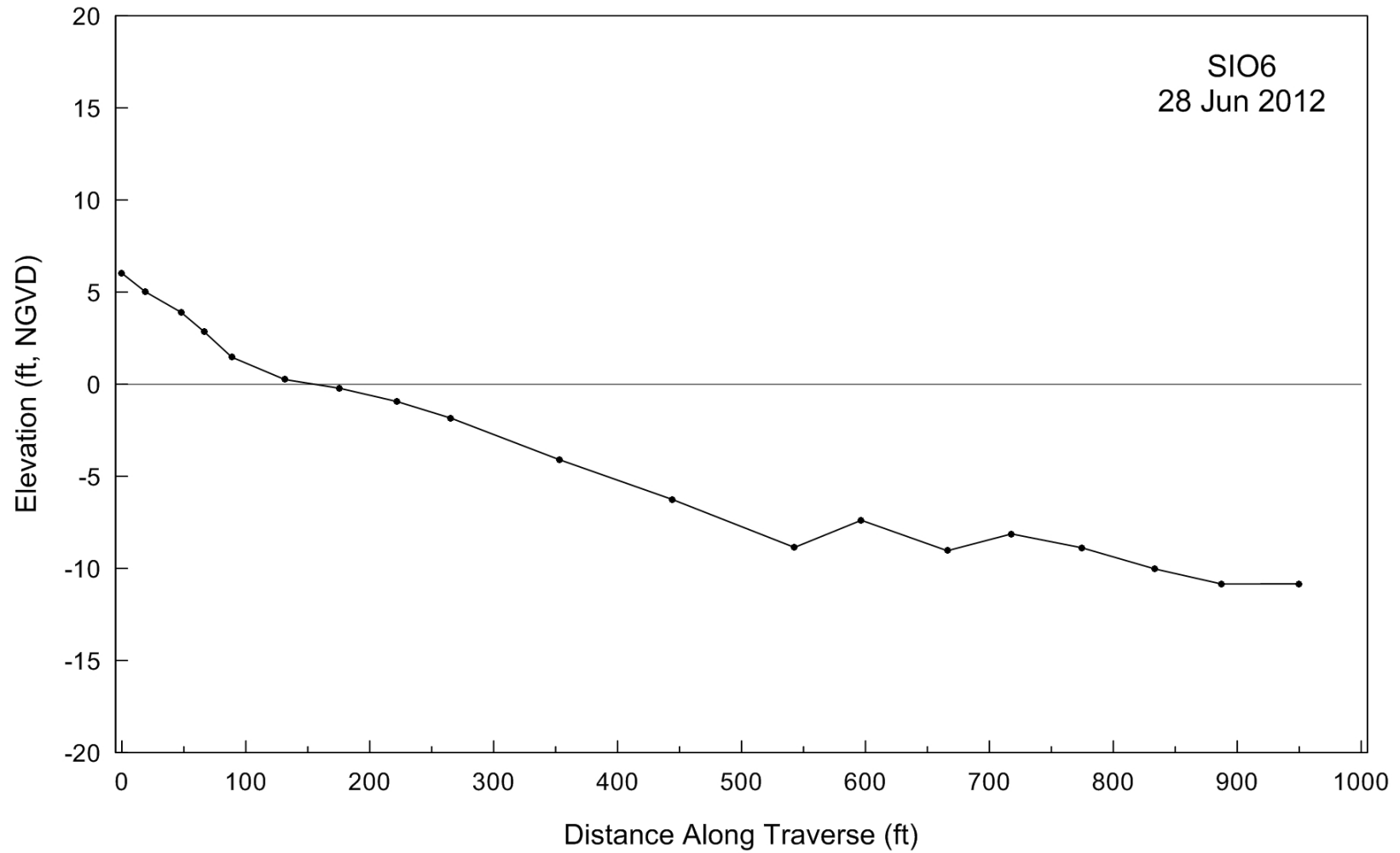
Figure A-4. Beach profile for SIO6 taken on 28 June 2012.
