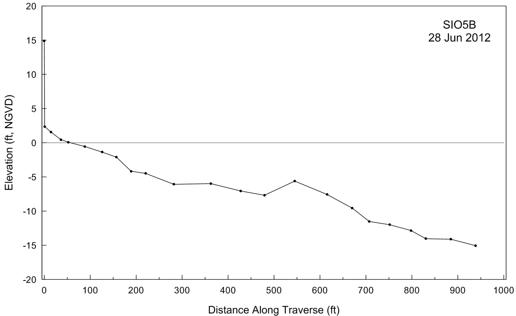
Figure A-3. Beach profile for SIO5B taken on 28 June 2012.
