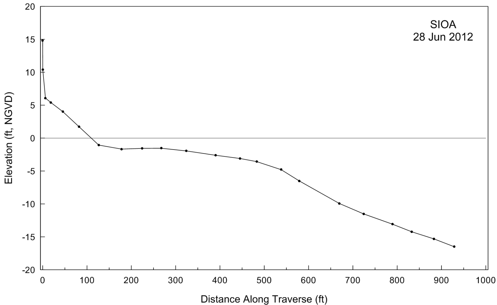
Figure A-5. Beach profile for SIOA taken on 28 June 2012.
