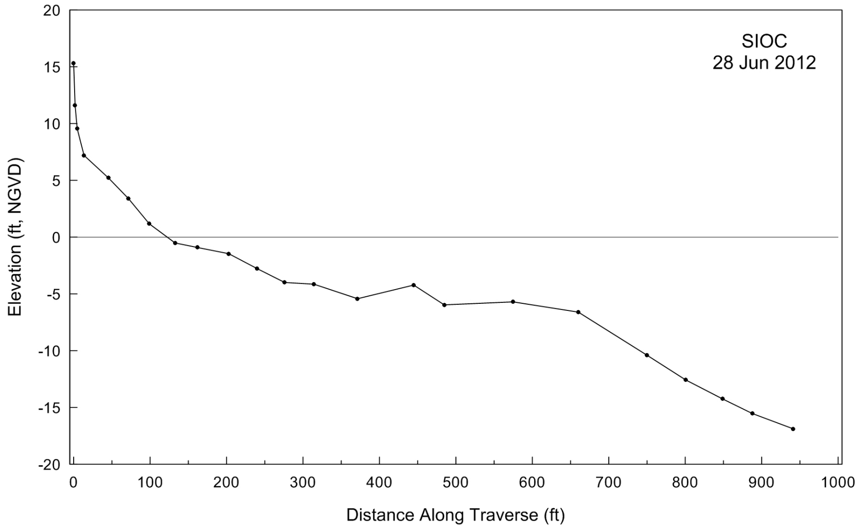
Figure A-7. Beach profile for SIOC taken on 28 June 2012.
