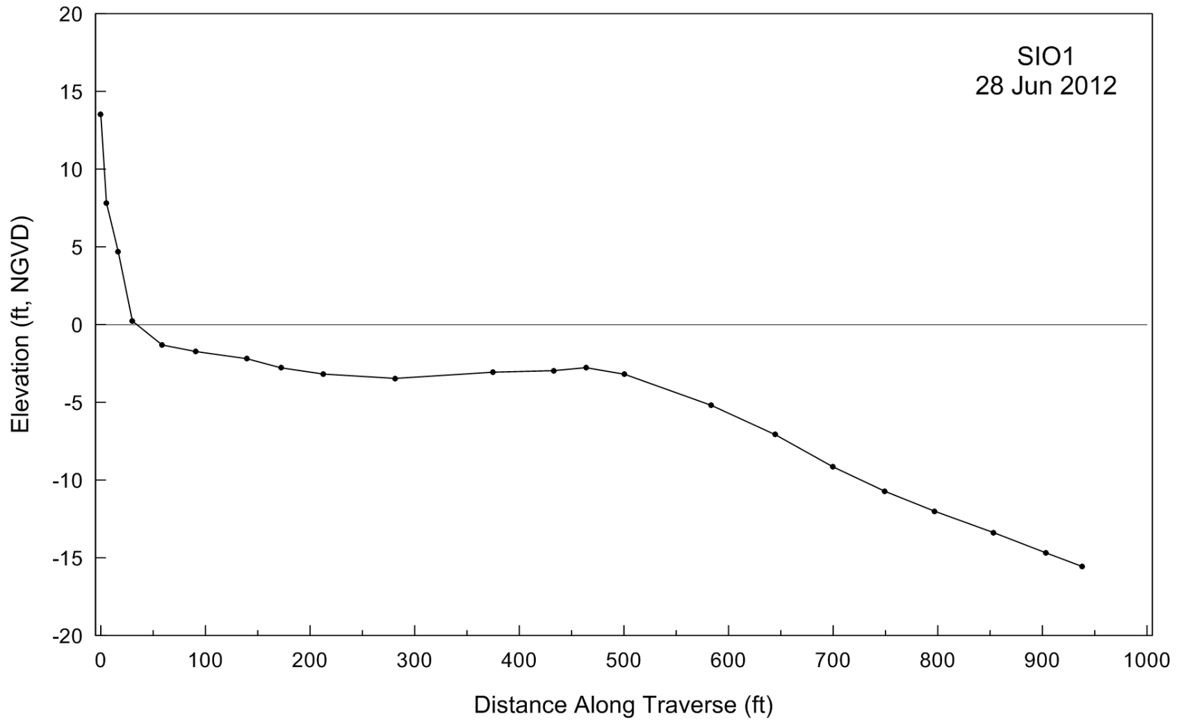
Figure A-1. Beach profile for SIO1 taken on 28 June 2012.
