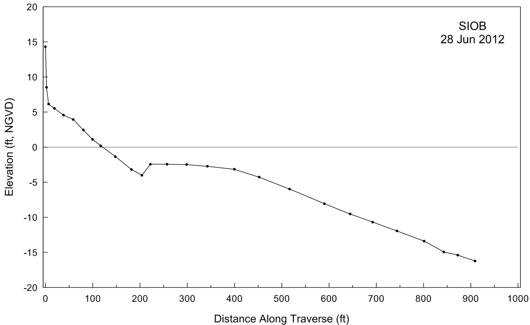
Figure A-6. Beach profile for SIOB taken on 28 June 2012.
