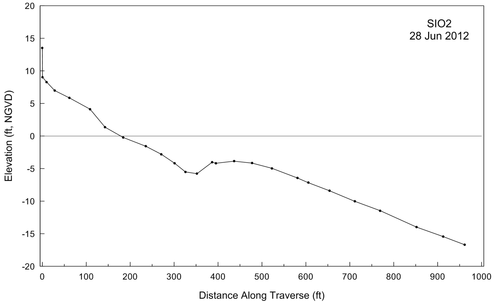
Figure A-2. Beach profile for SIO2 taken on 28 June 2012.
