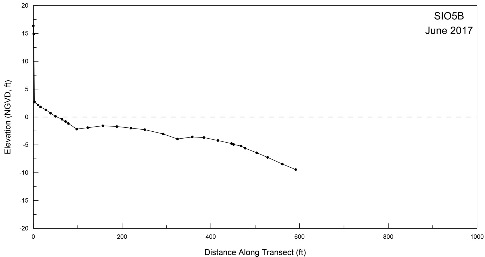
Figure A-3. Beach profile for SIO5B surveyed on 20 June 2017.
