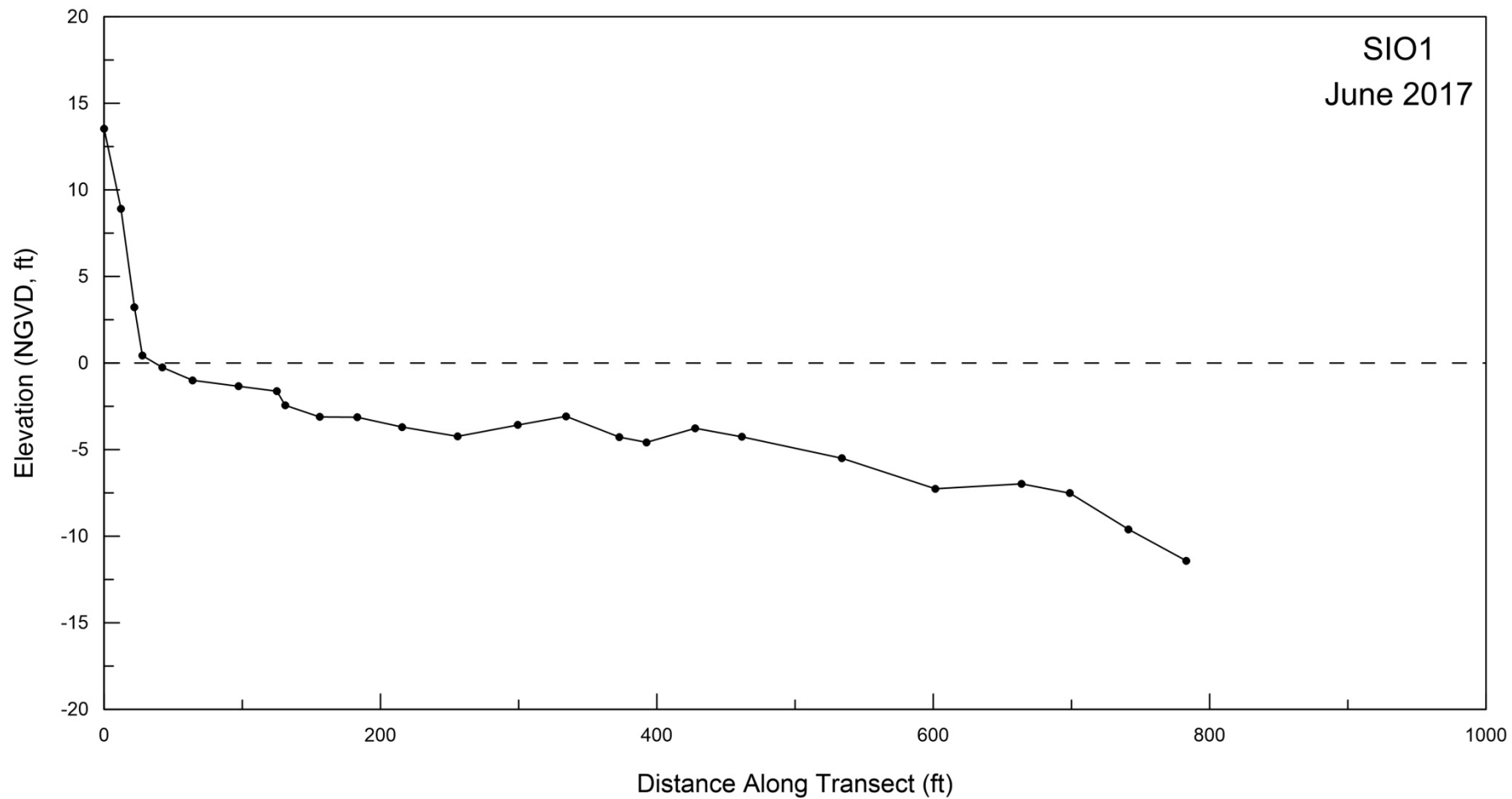
Figure A-1. Beach profile for SIO1 surveyed on 20 June 2017.
