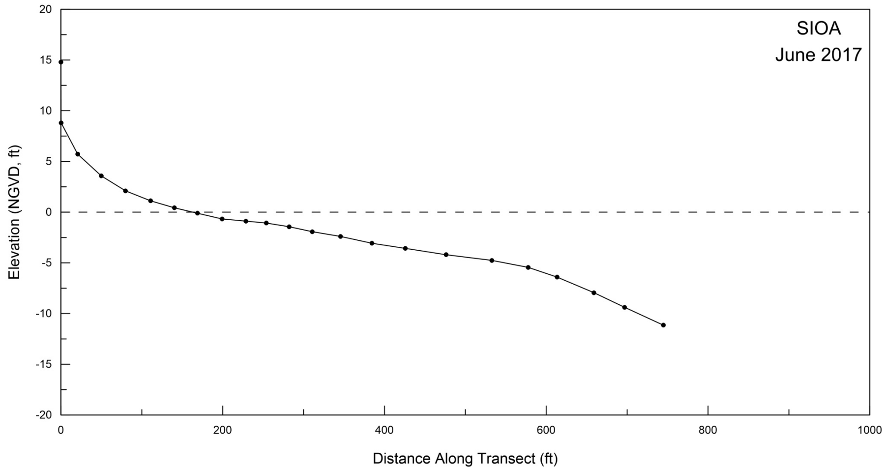
Figure A-5. Beach profile for SIOA surveyed on 20 June 2017.
