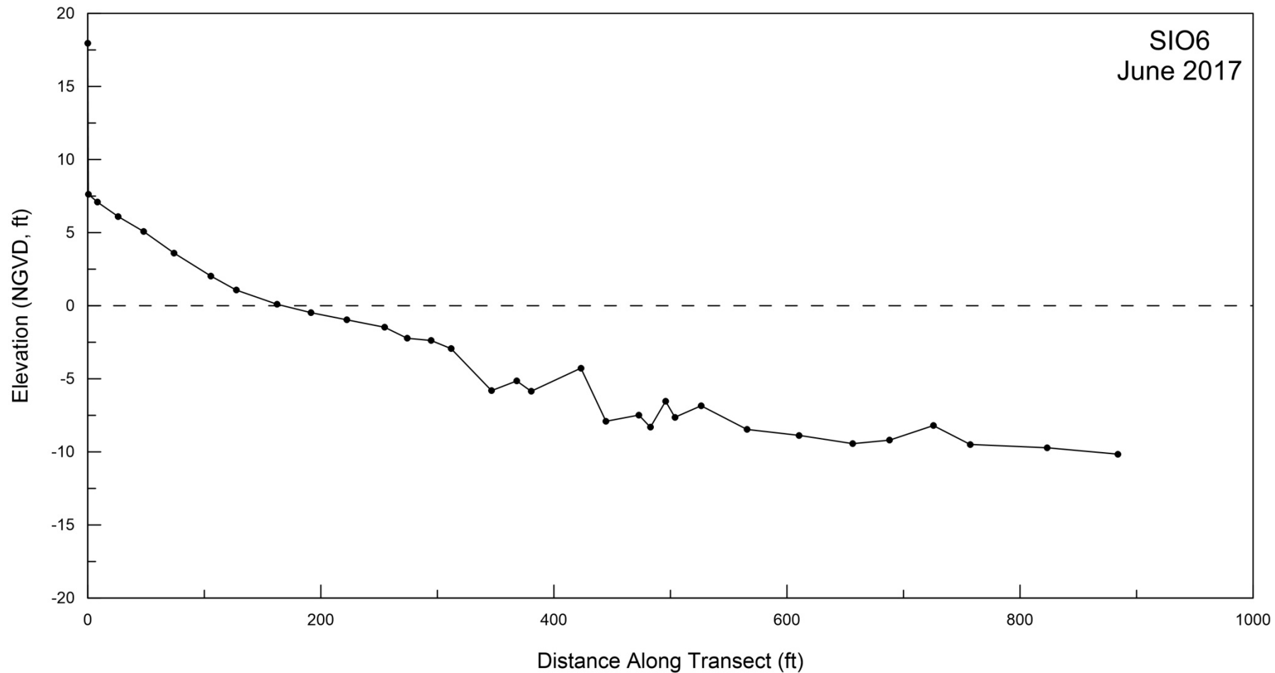
Figure A-4. Beach profile for SIO6 surveyed on 20 June 2017.
