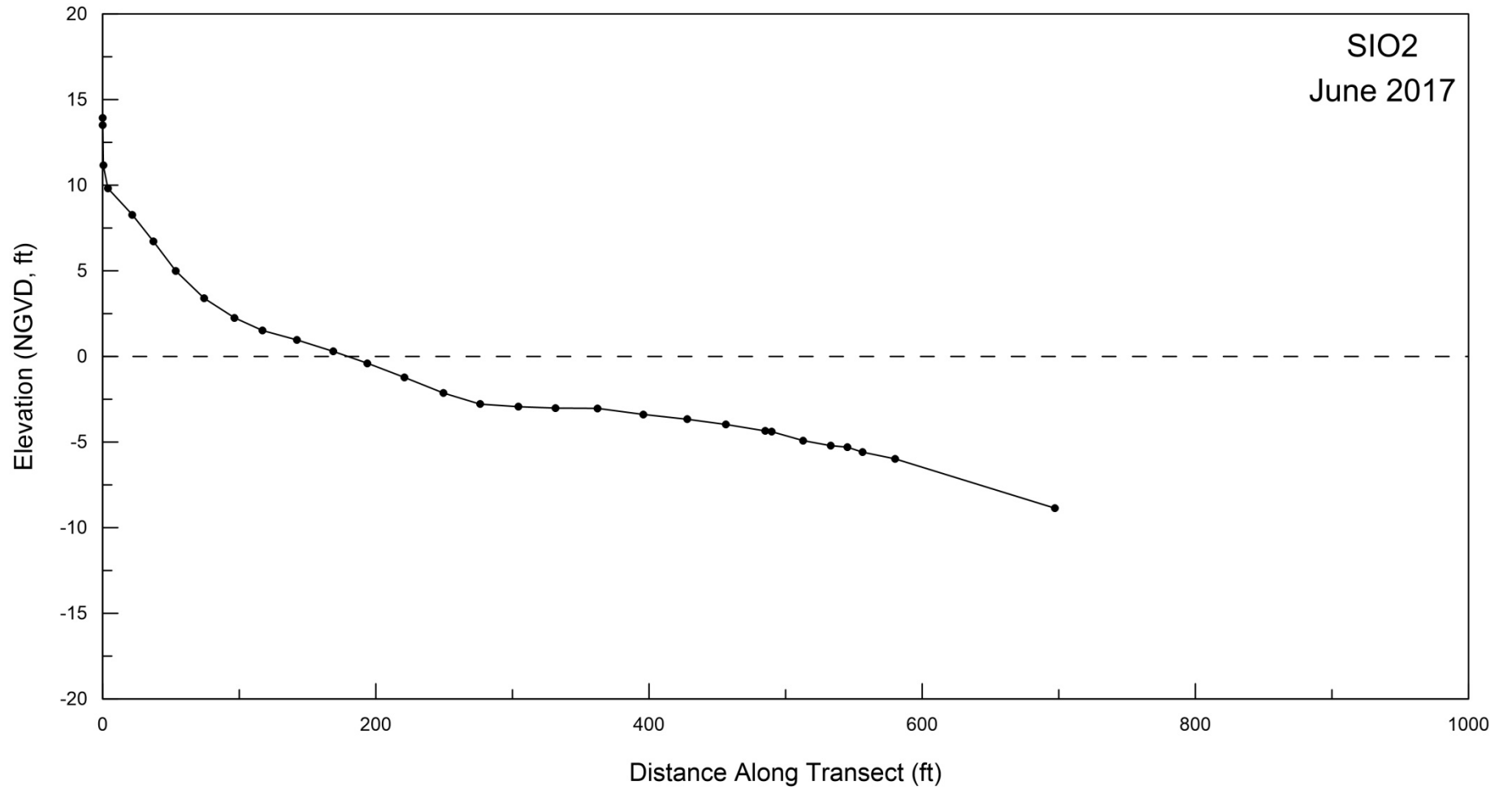
Figure A-2. Beach profile for SIO2 surveyed on 20 June 2017.
