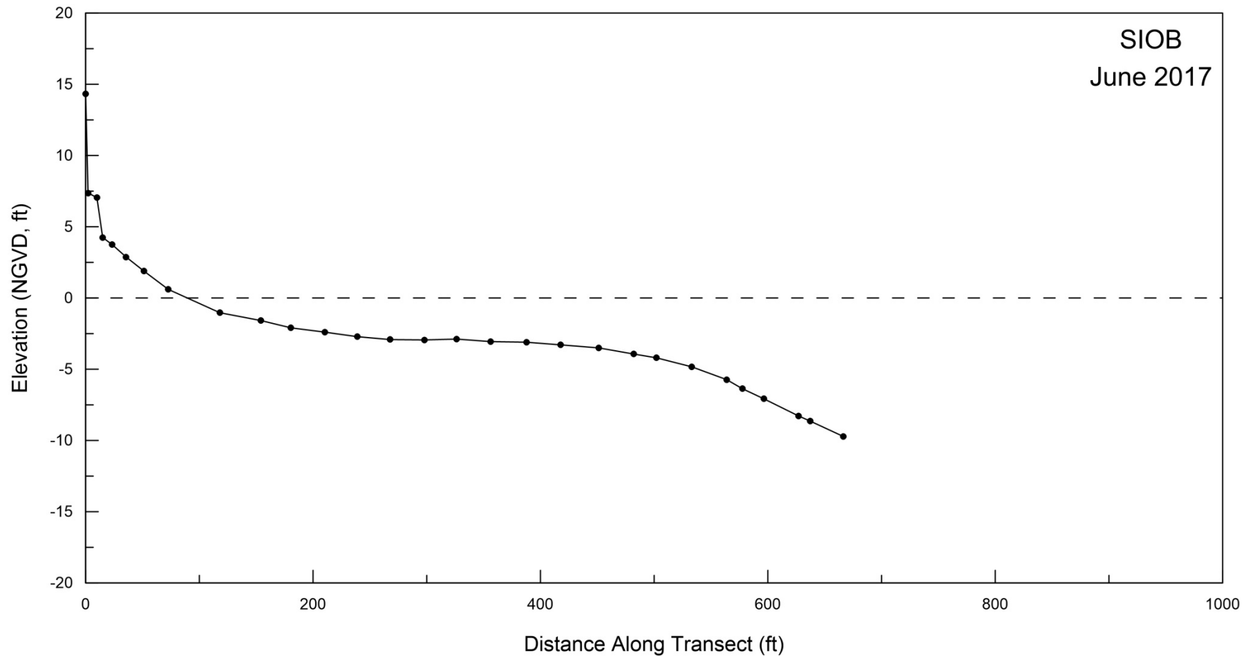
Figure A-6. Beach profile for SIOB surveyed on 20 June 2017.
