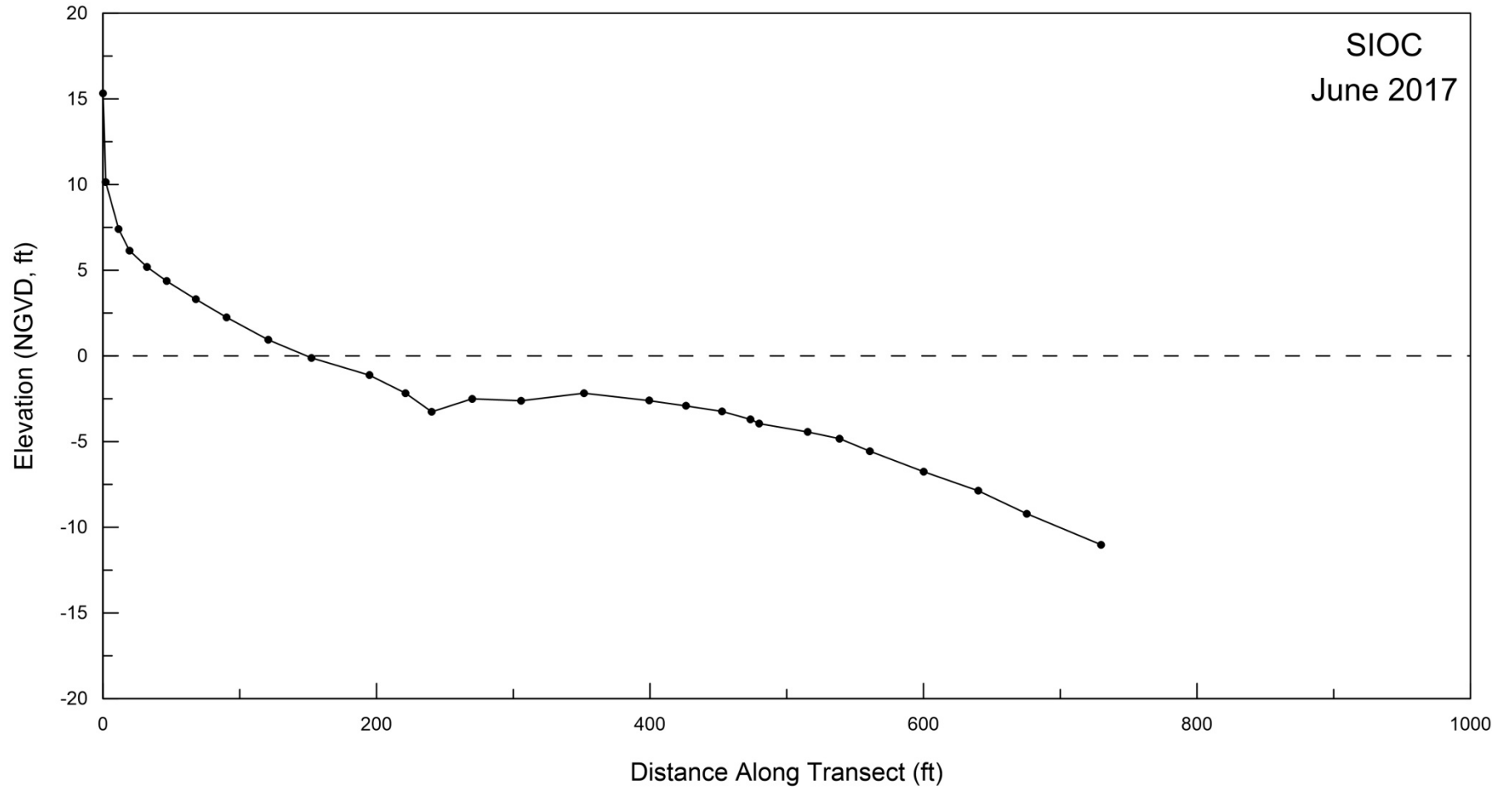
Figure A-7. Beach profile for SIOC surveyed on 20 June 2017.
