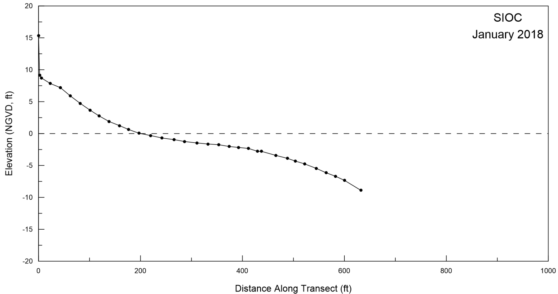
Figure A-7. Beach profile for SIOC surveyed on 08 January 2018.
