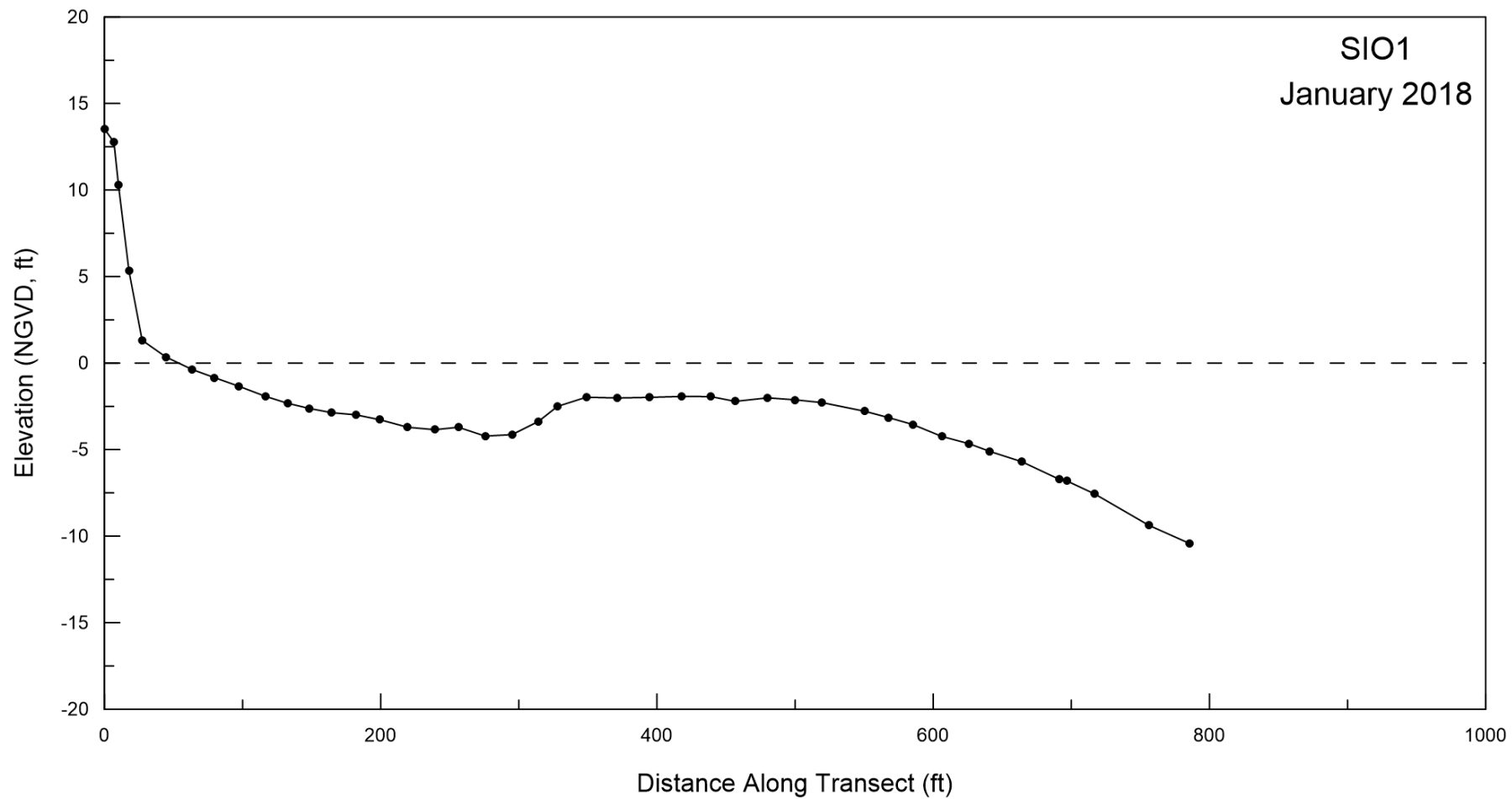
Figure A-1. Beach profile for SIO1 surveyed on 08 January 2018.
