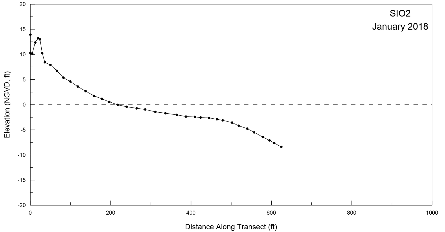
Figure A-2. Beach profile for SIO2 surveyed on 08 January 2018.
