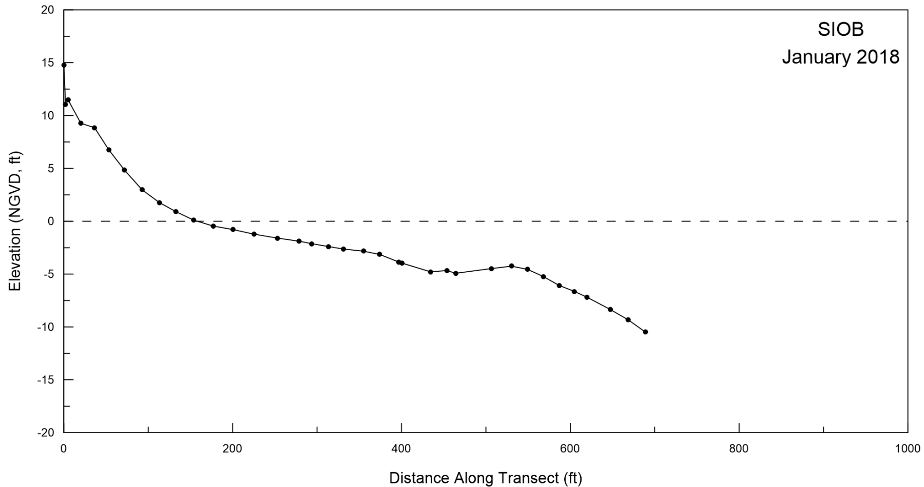
Figure A-6. Beach profile for SIOB surveyed on 08 January 2018.
