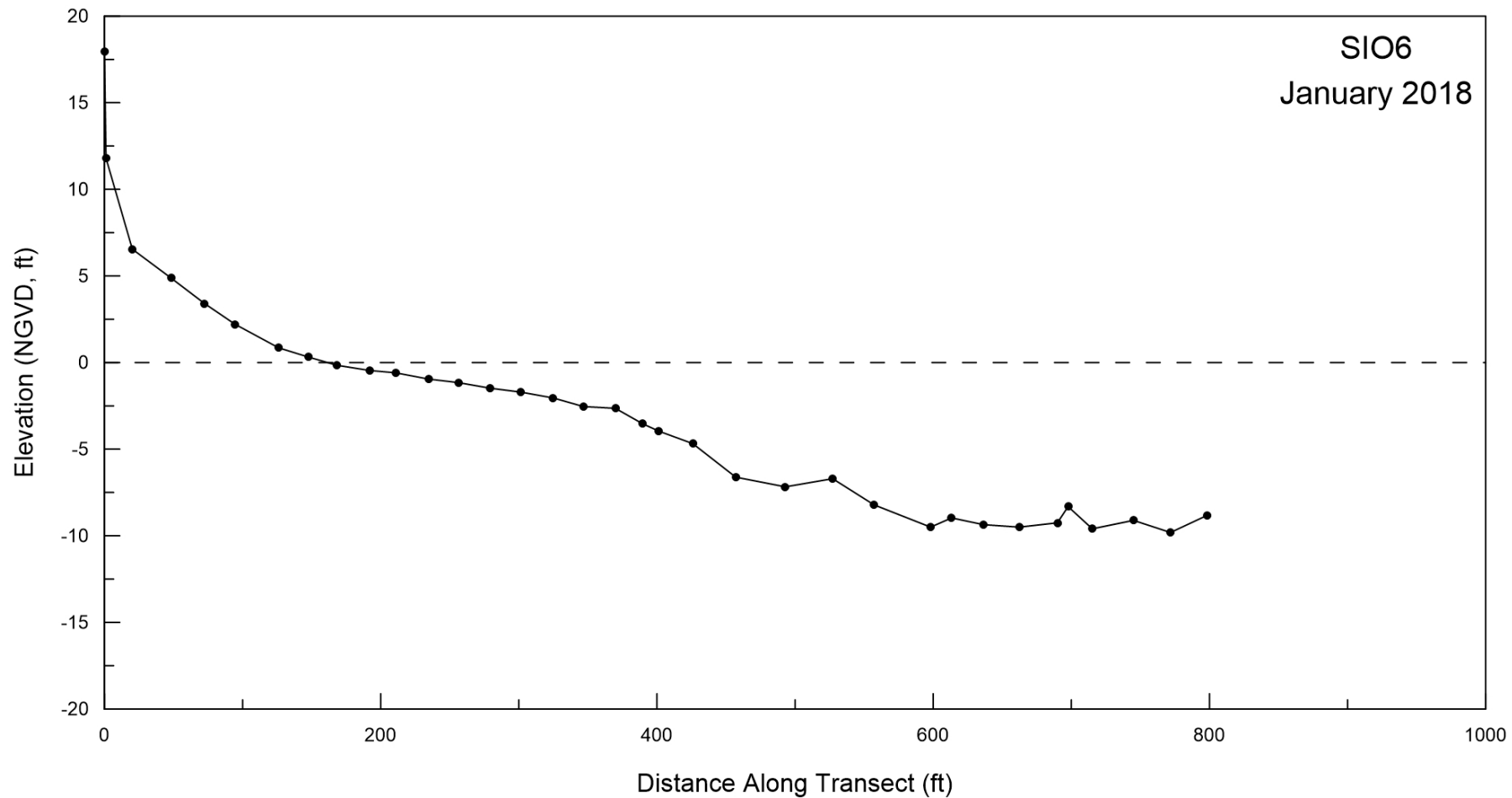
Figure A-4. Beach profile for SIO6 surveyed on 08 January 2018.
