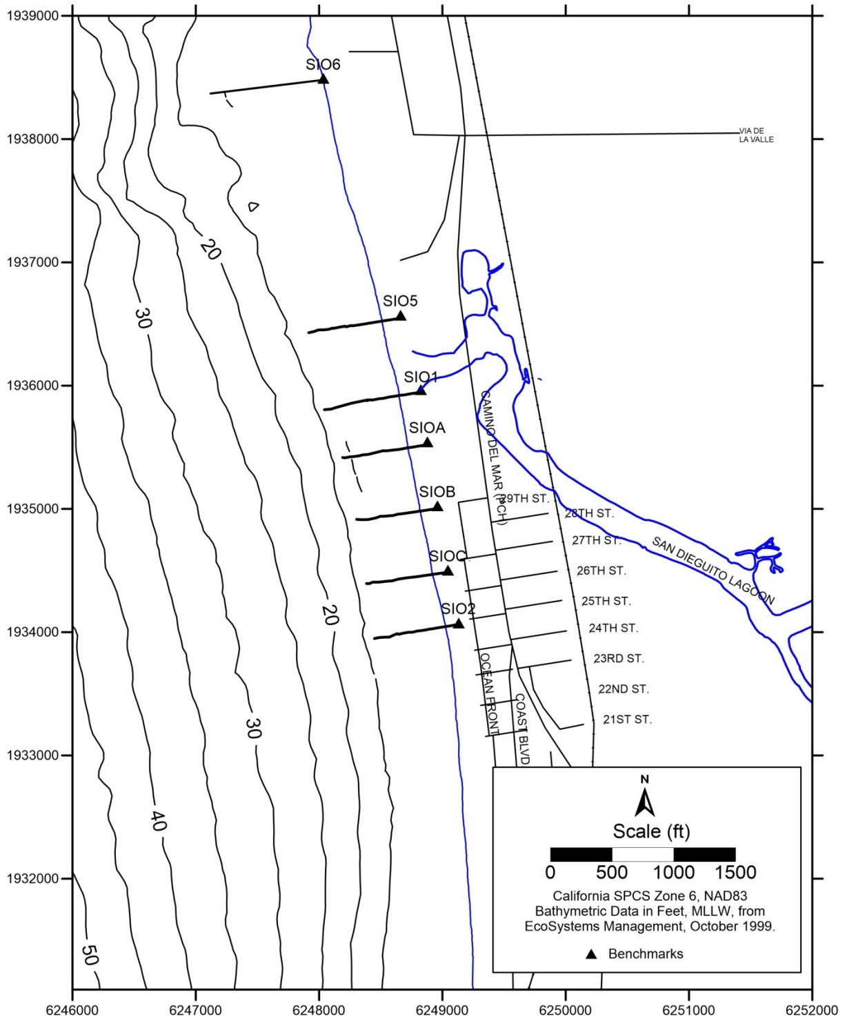
Figure 2. Beach profiles surveyed on 08 January 2018.
