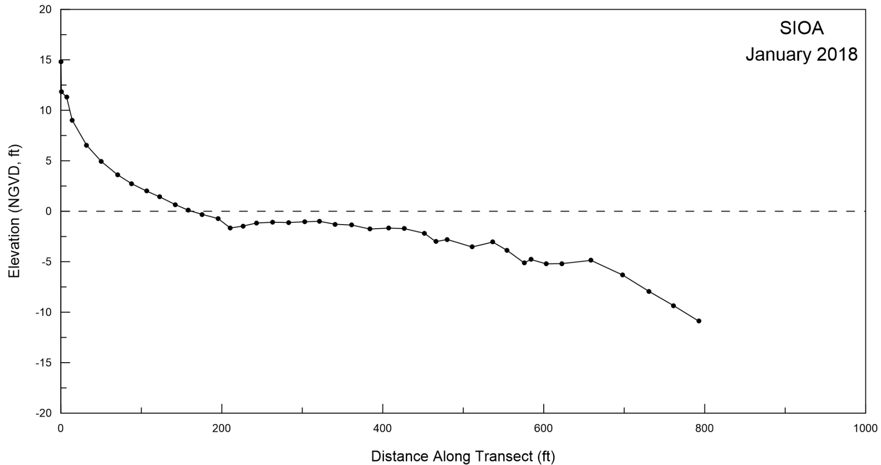
Figure A-5. Beach profile for SIOA surveyed on 08 January 2018.
