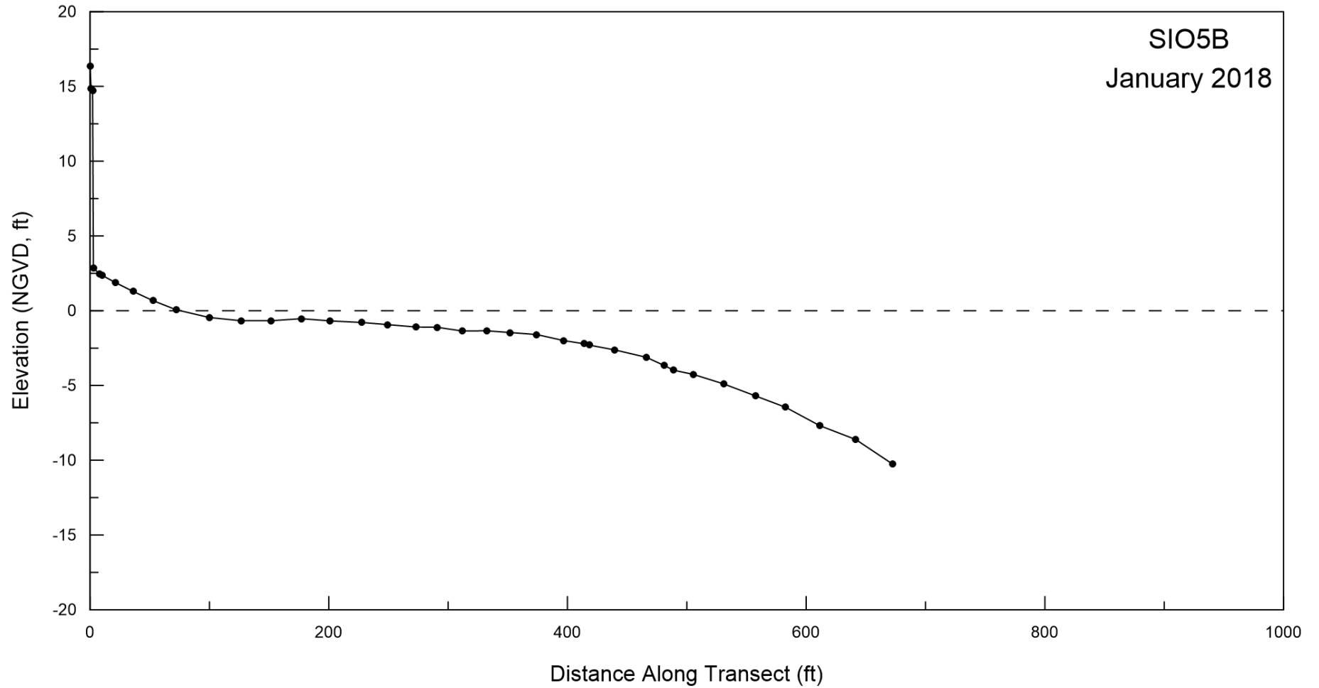
Figure A-3. Beach profile for SIO5B surveyed on 08 January 2018.
