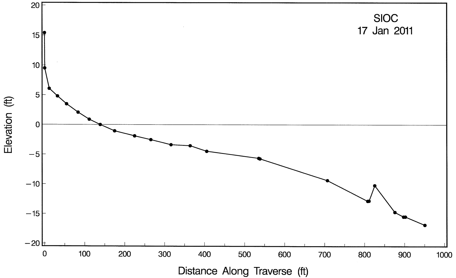
Figure A-7. Beach profile for SIOC taken on 17 January 2011.
