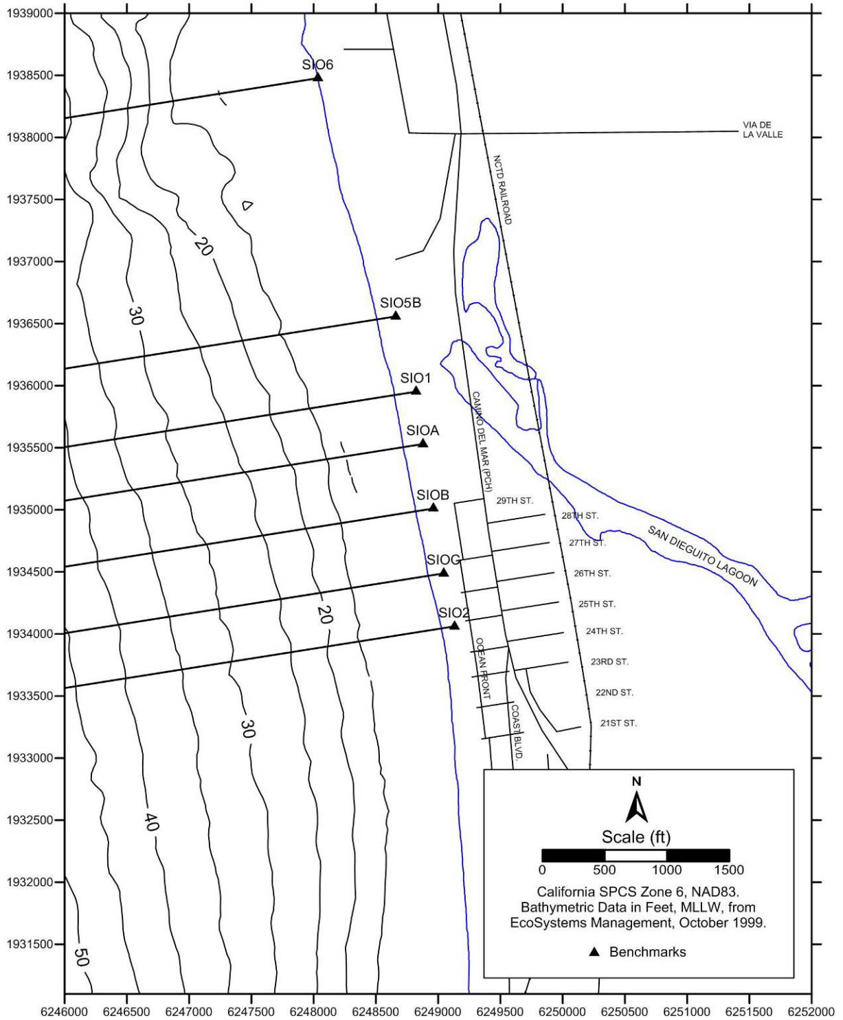
Figure 2. Beach profiles surveyed on 17 January 2011.
