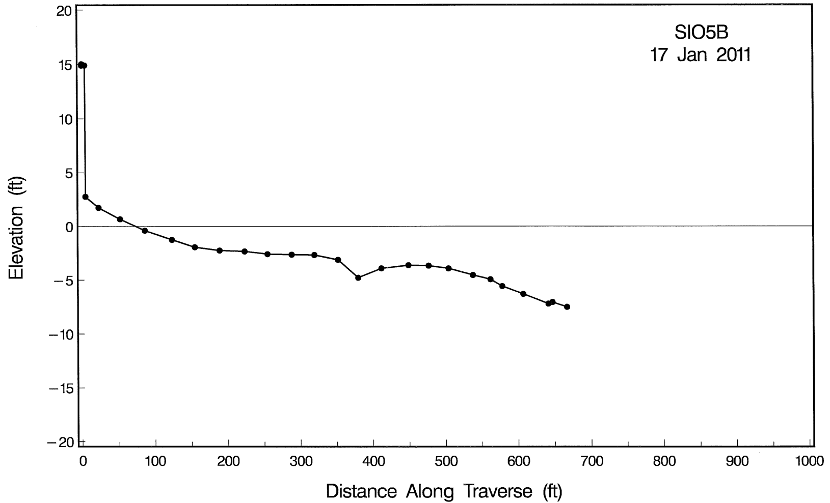
Figure A-3. Beach profile for SIO5B taken on 17 January 2011.
