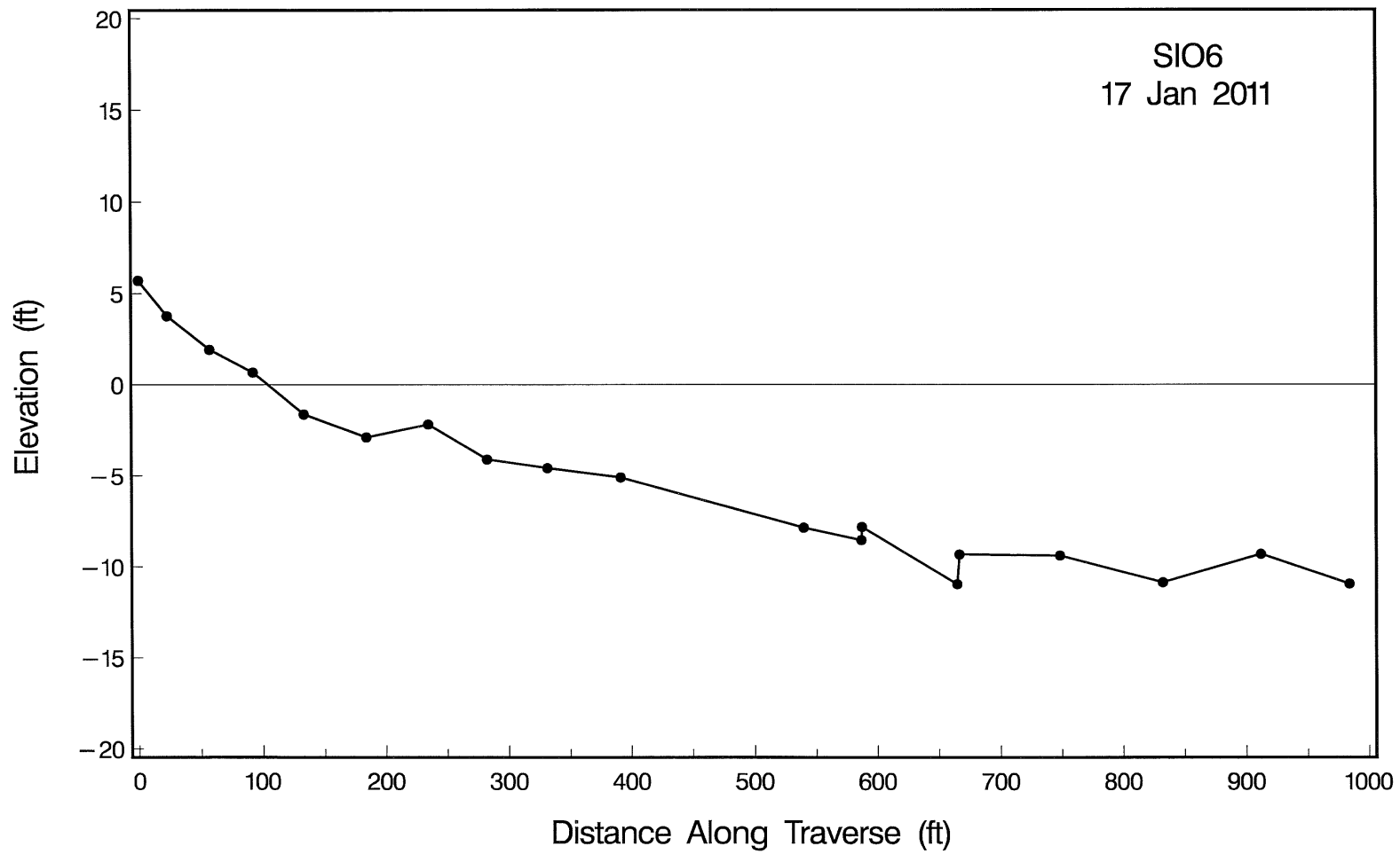
Figure A-4. Beach profile for SIO6 taken on 17 January 2011.
