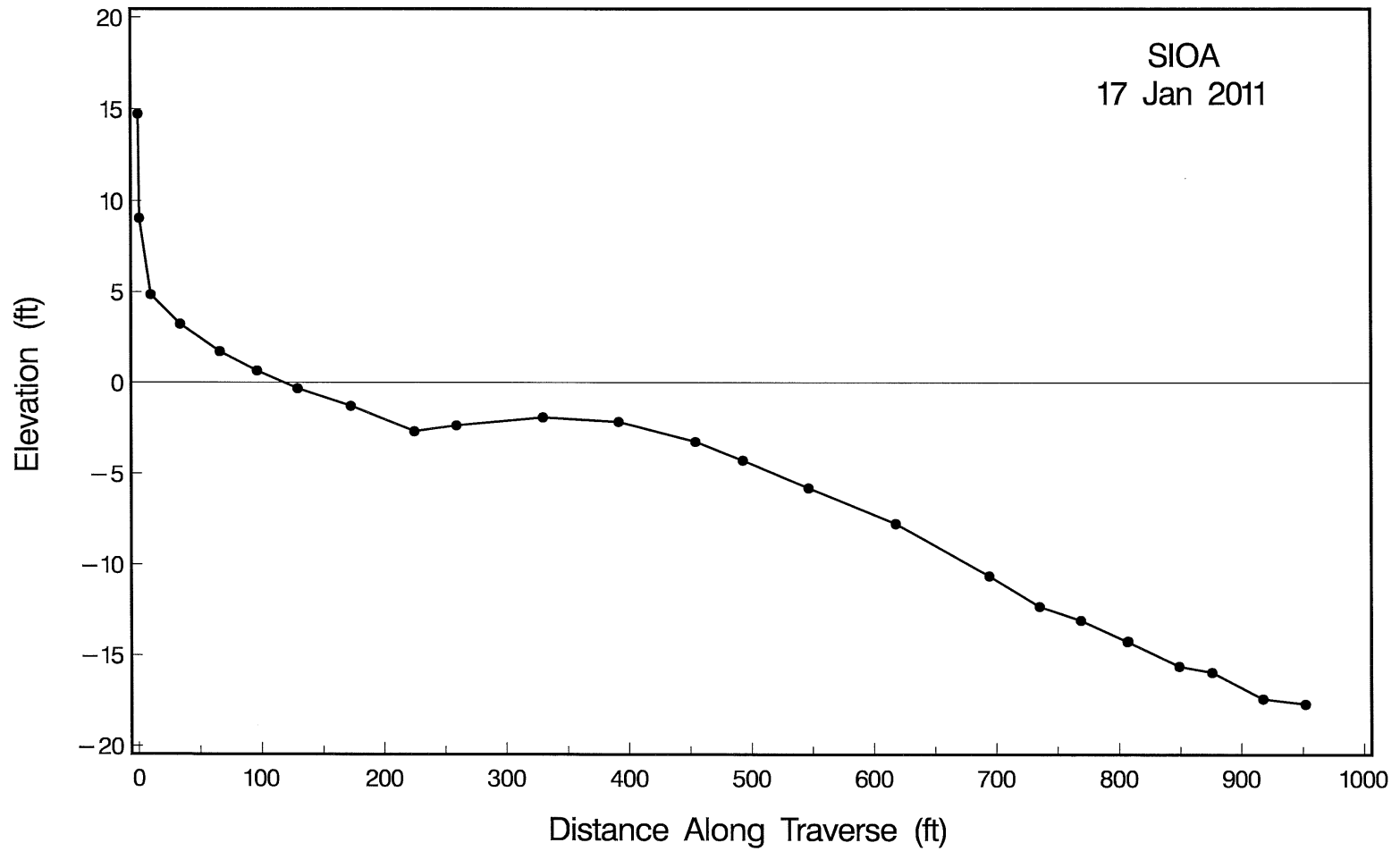
Figure A-5. Beach profile for SIOA taken on 17 January 2011.
