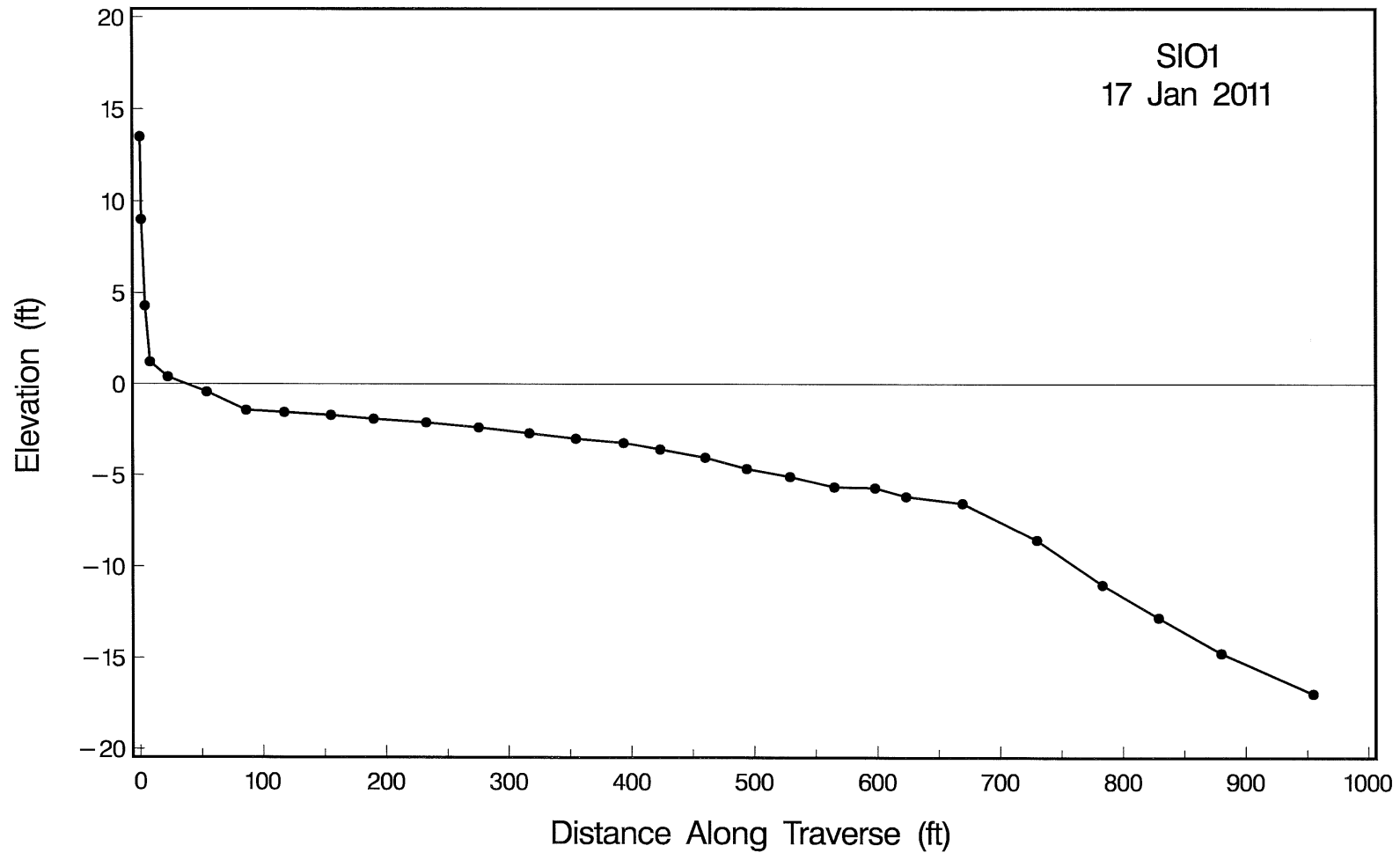
Figure A-1. Beach profile for SIO1 taken on 17 January 2011.
