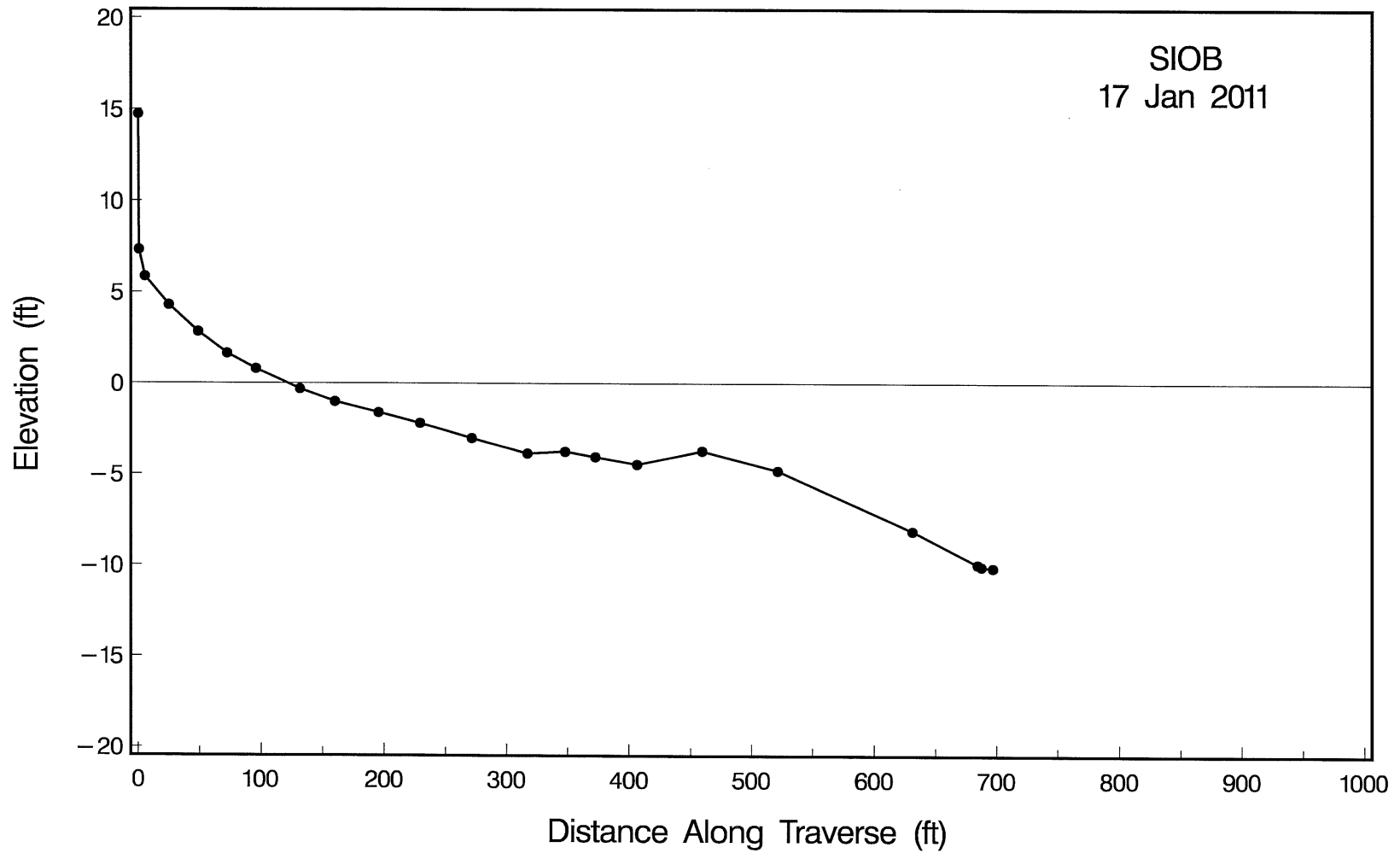
Figure A-6. Beach profile for SIOB taken on 17 January 2011.
