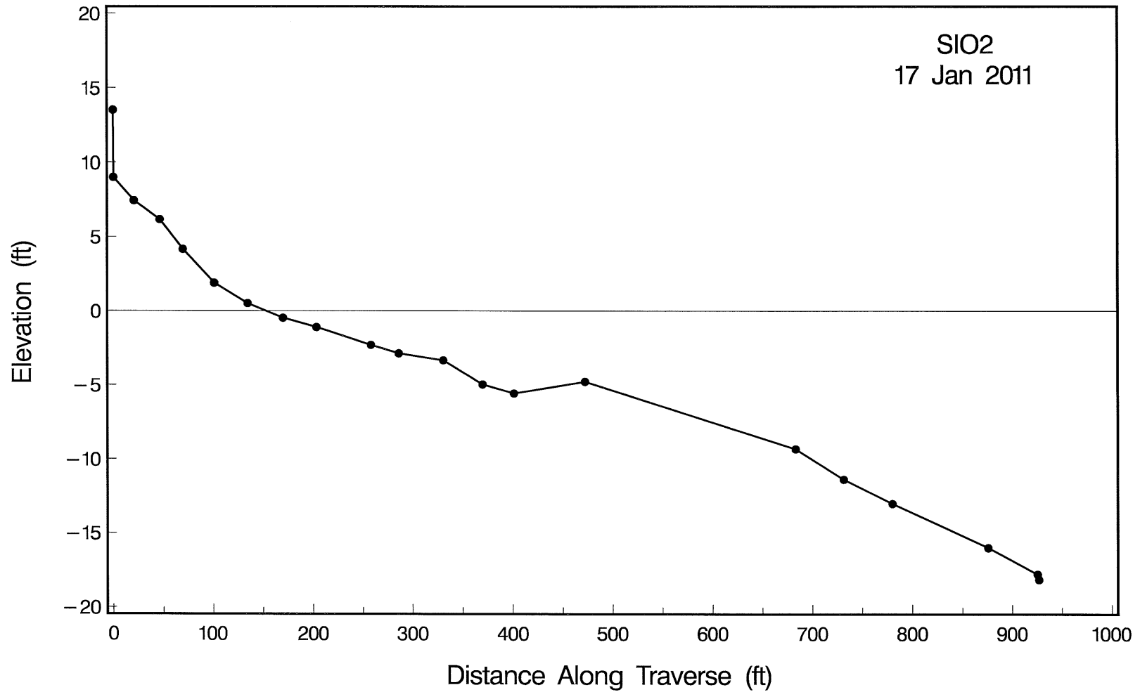
Figure A-2. Beach profile for SIO2 taken on 17 January 2011.
