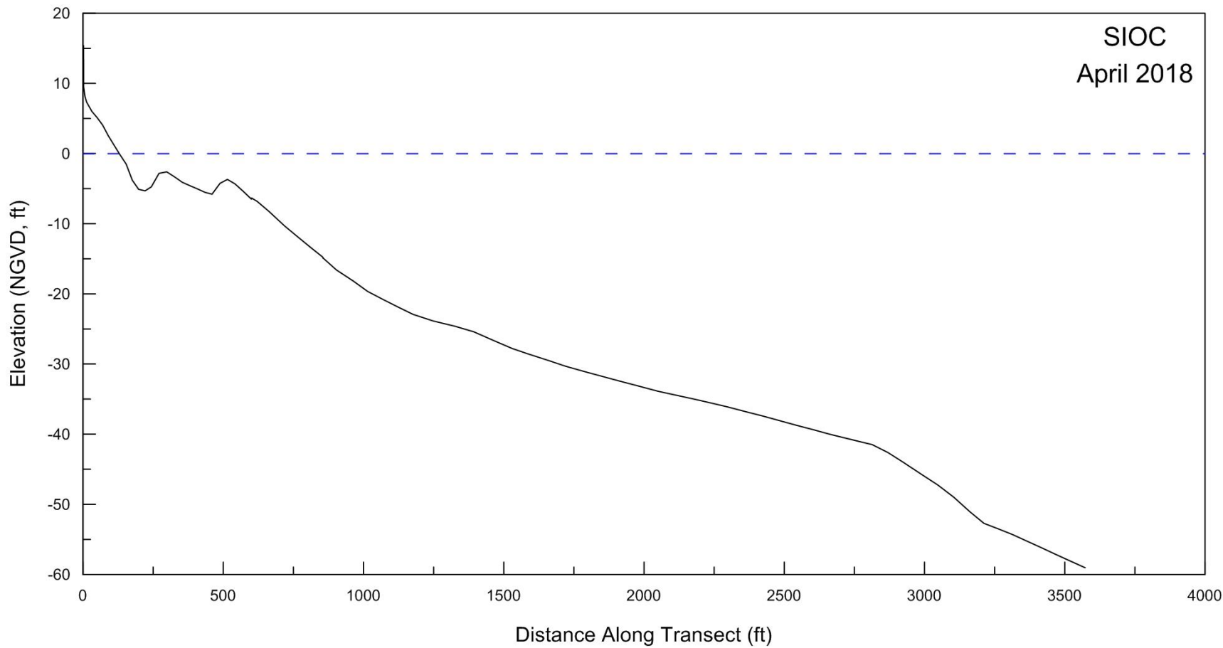
Figure A-7. Beach profile for SIOC surveyed on 25 April 2018.
