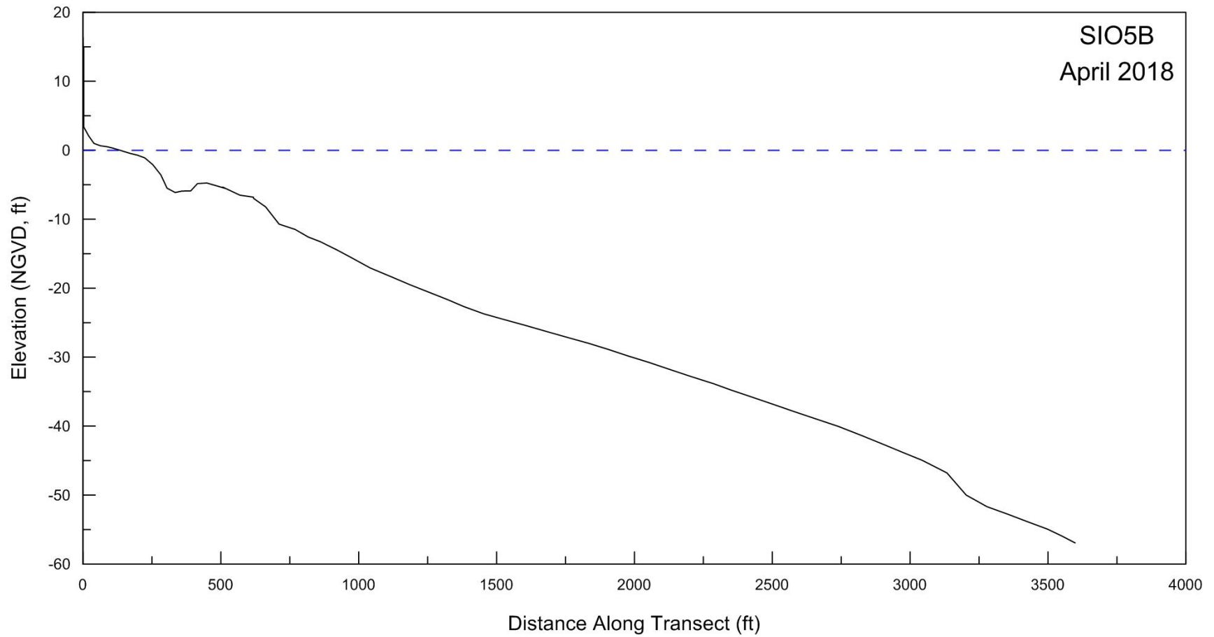
Figure A-3. Beach profile for SIO5B surveyed on 25 April 2018.
