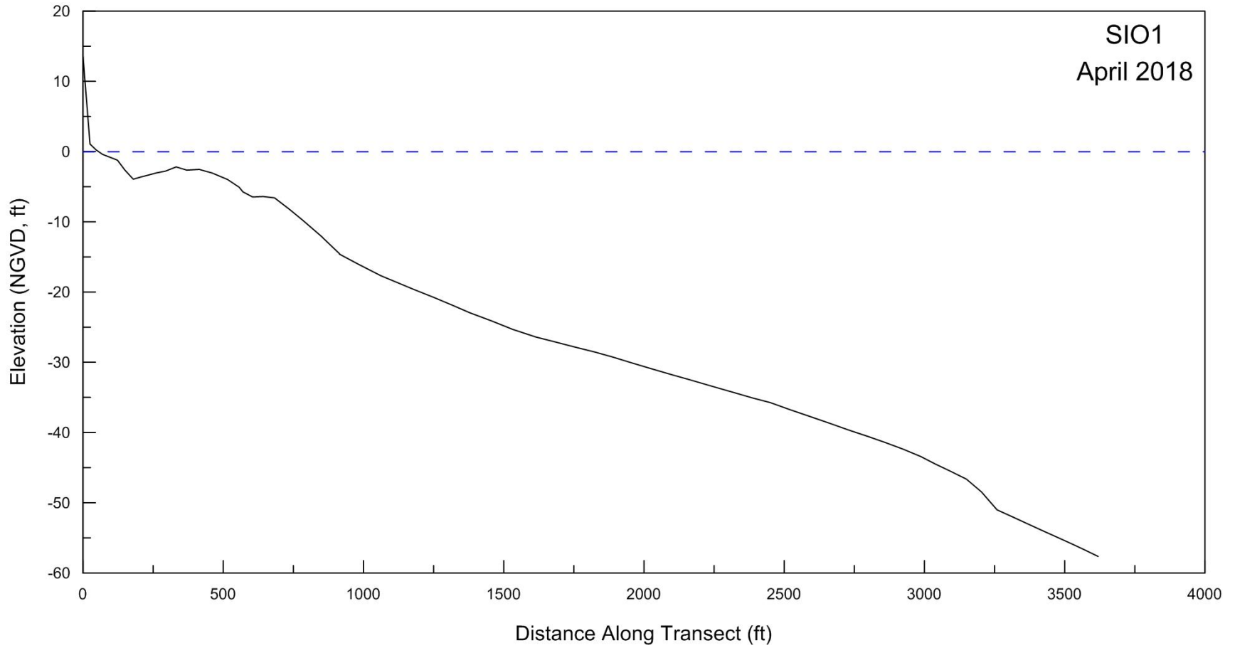
Figure A-1. Beach profile for SIO1 surveyed on 25 April 2018.
