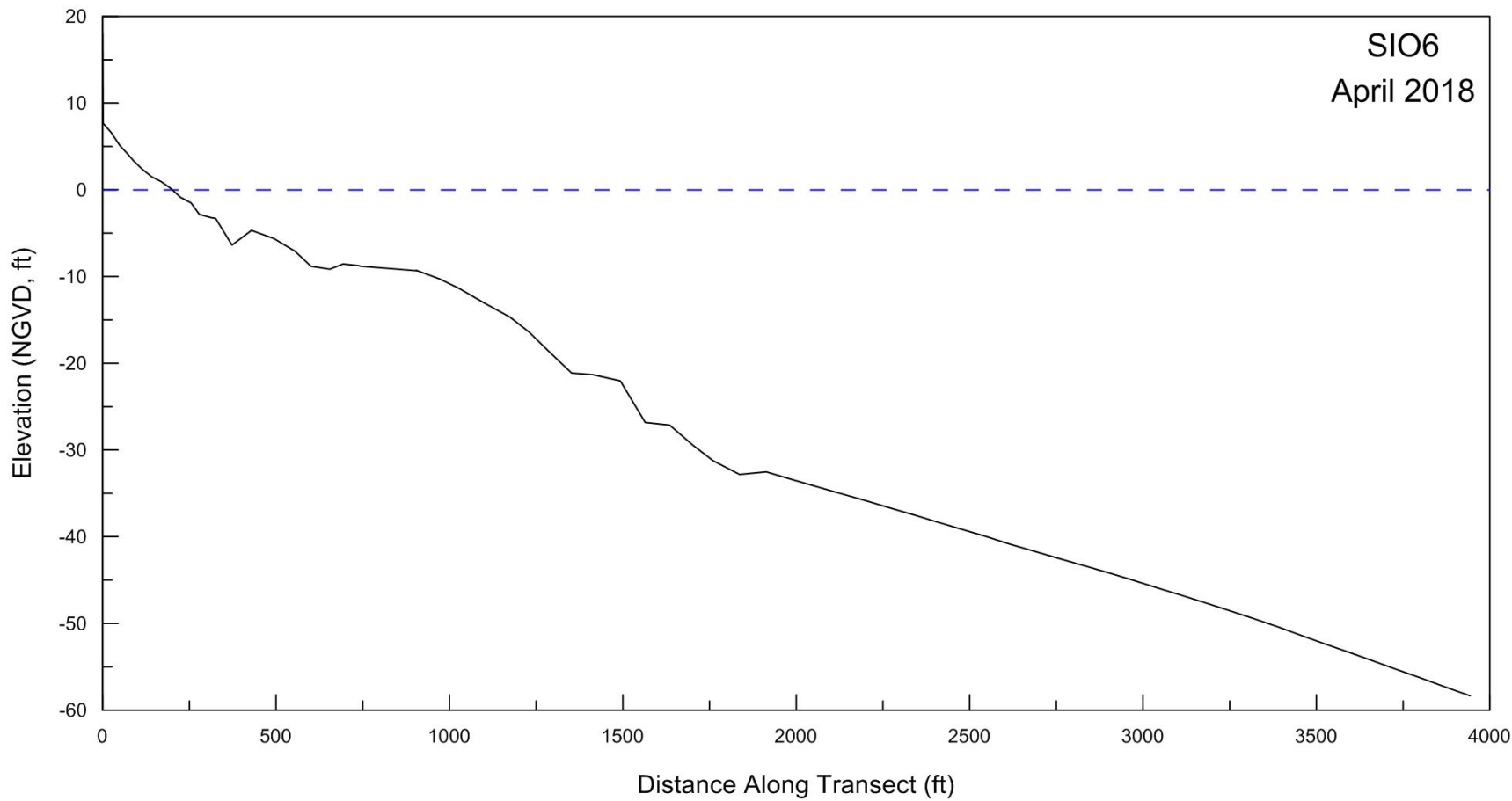
Figure A-4. Beach profile for SIO6 surveyed on 25 April 2018.
