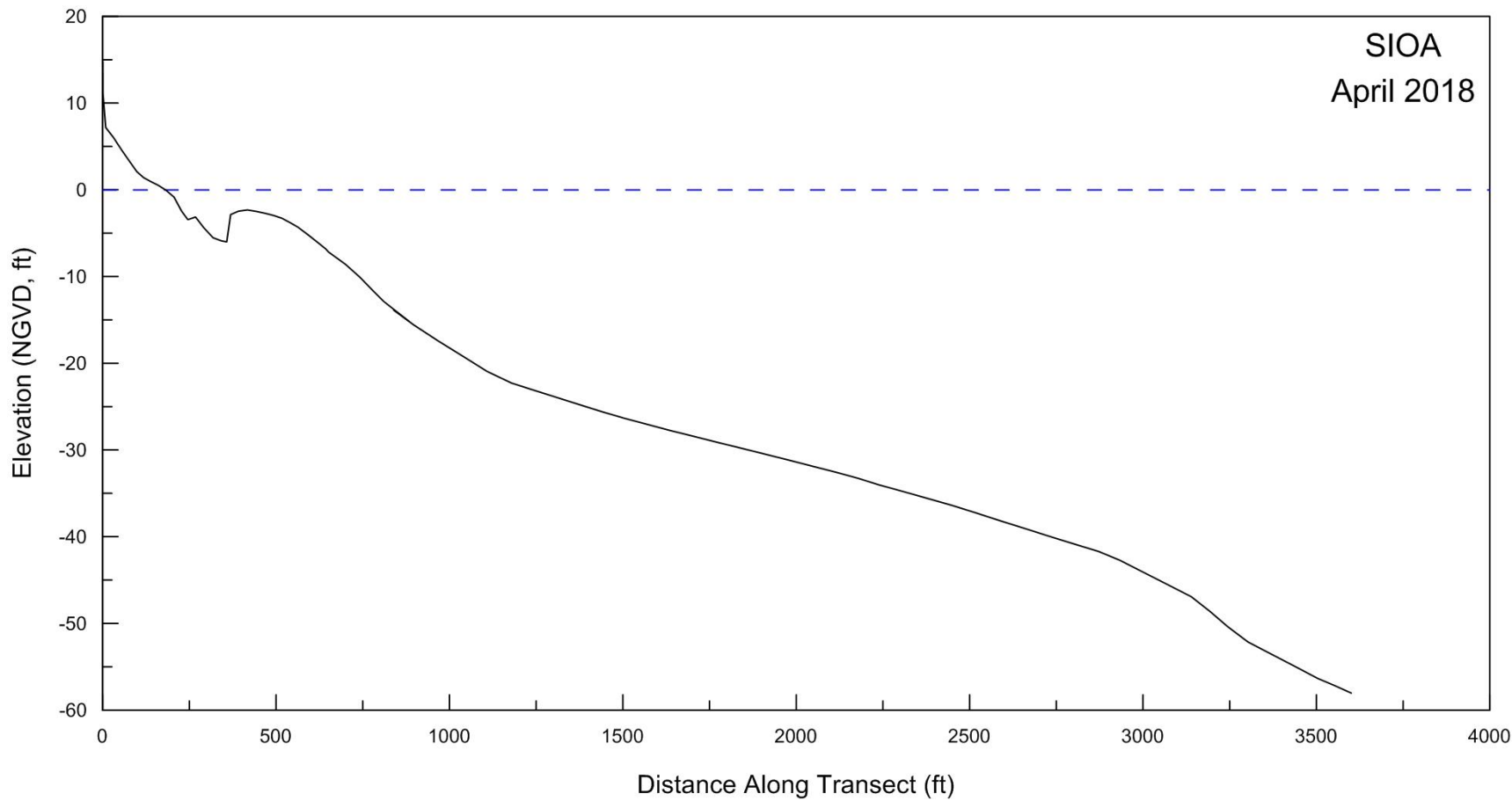
Figure A-5. Beach profile for SIOA surveyed on 25 April 2018.
