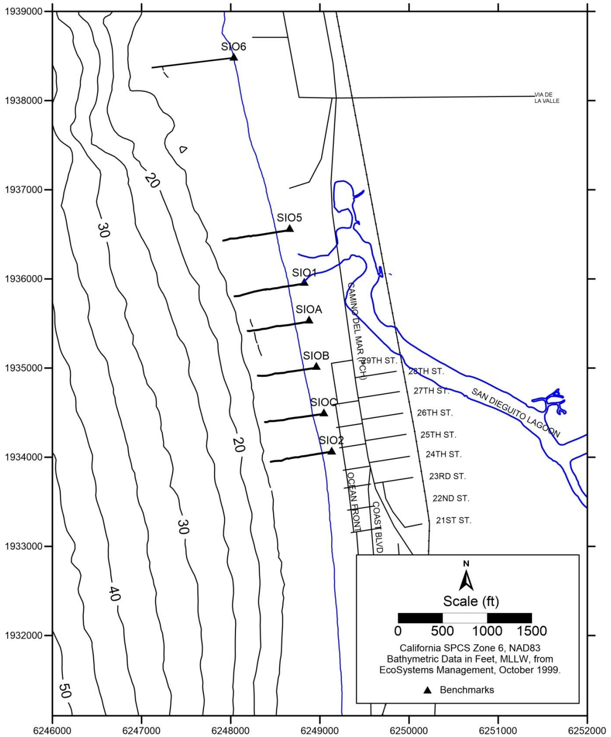
Figure 2. Beach profiles surveyed on 25 April 2018.
