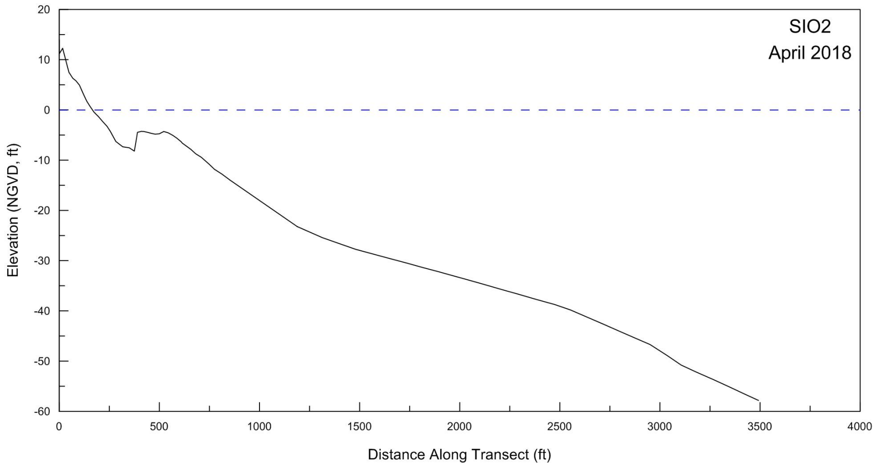
Figure A-2. Beach profile for SIO2 surveyed on 25 April 2018.
