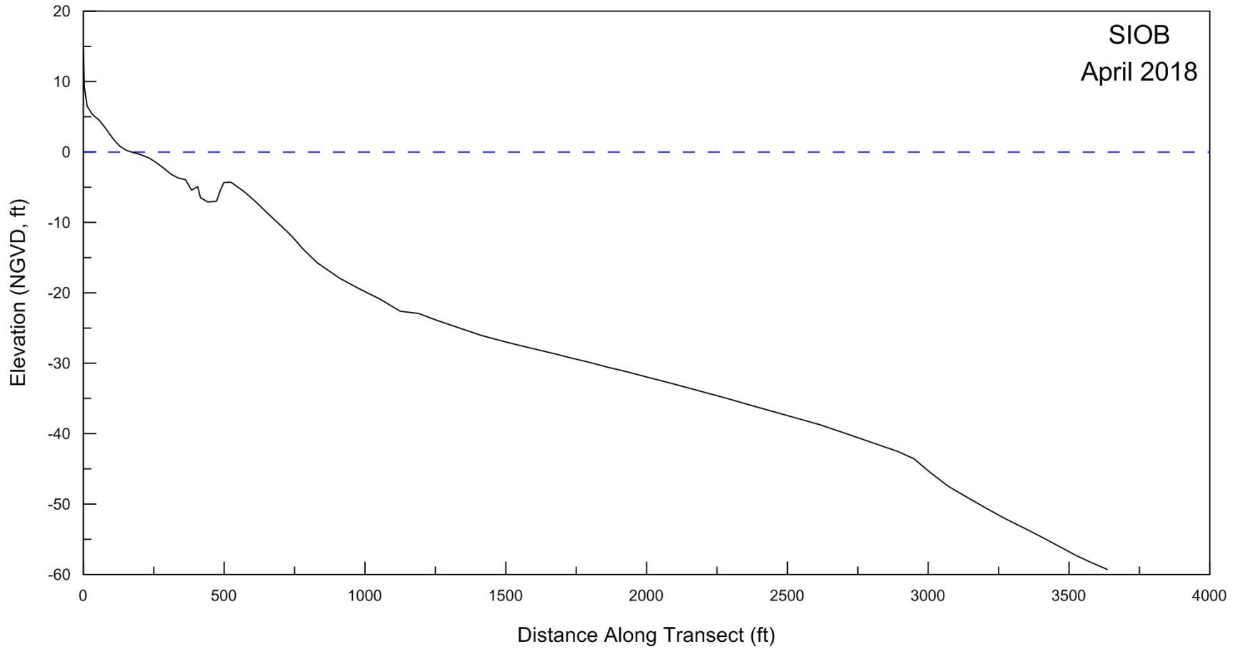
Figure A-6. Beach profile for SIOB surveyed on 25 April 2018.
