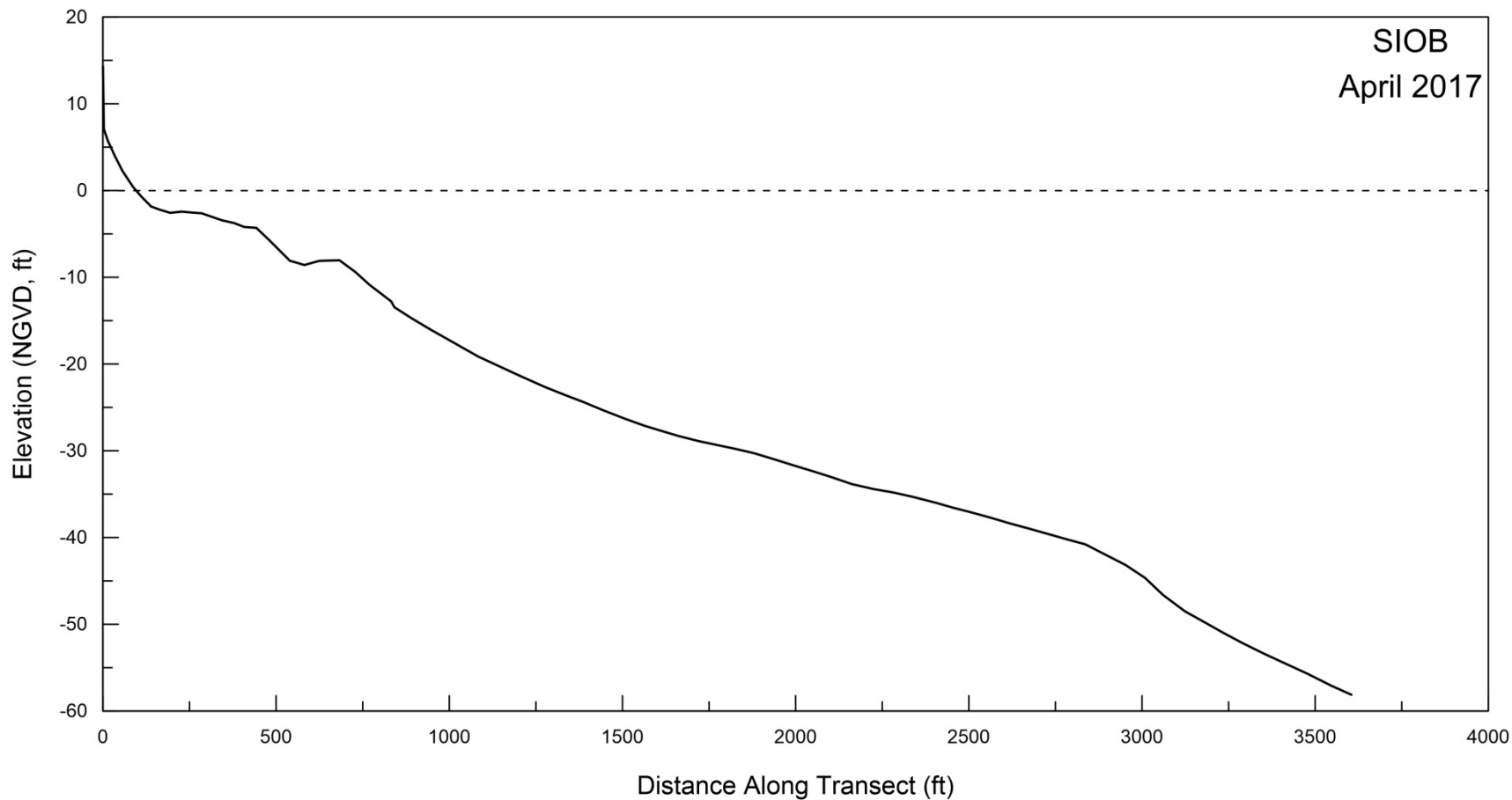
Figure A-6. Beach profile for SIOB surveyed on 05 April 2017.
