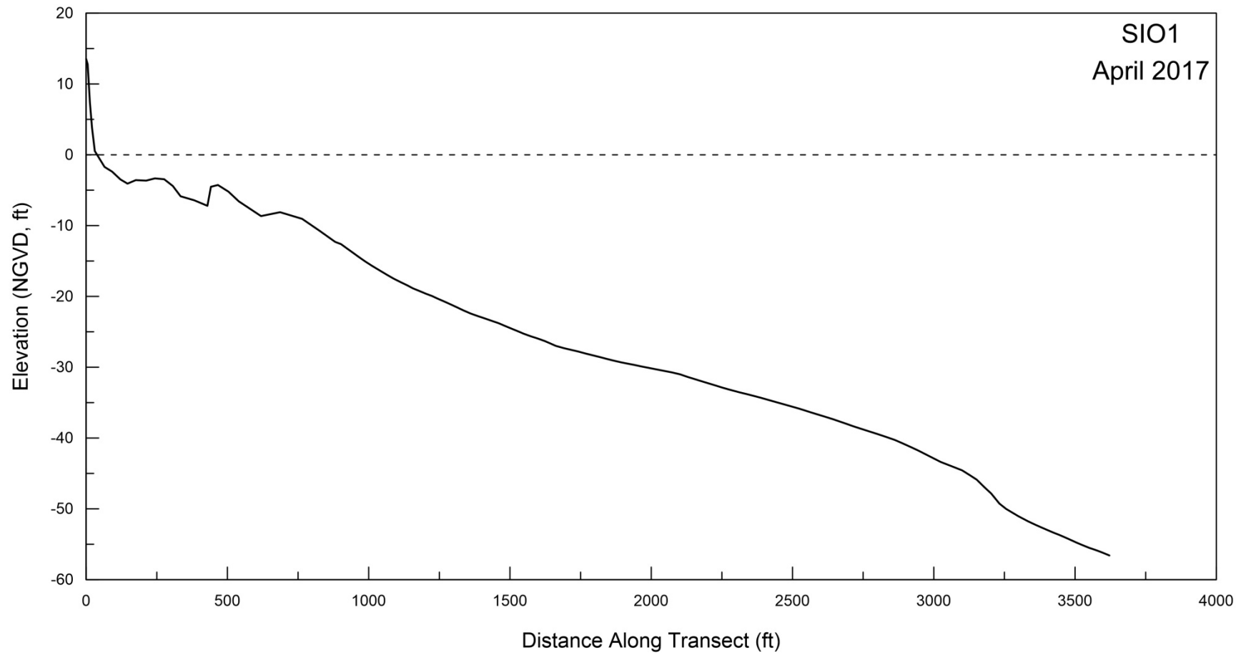
Figure A-1. Beach profile for SIO1 surveyed on 05 April 2017.
