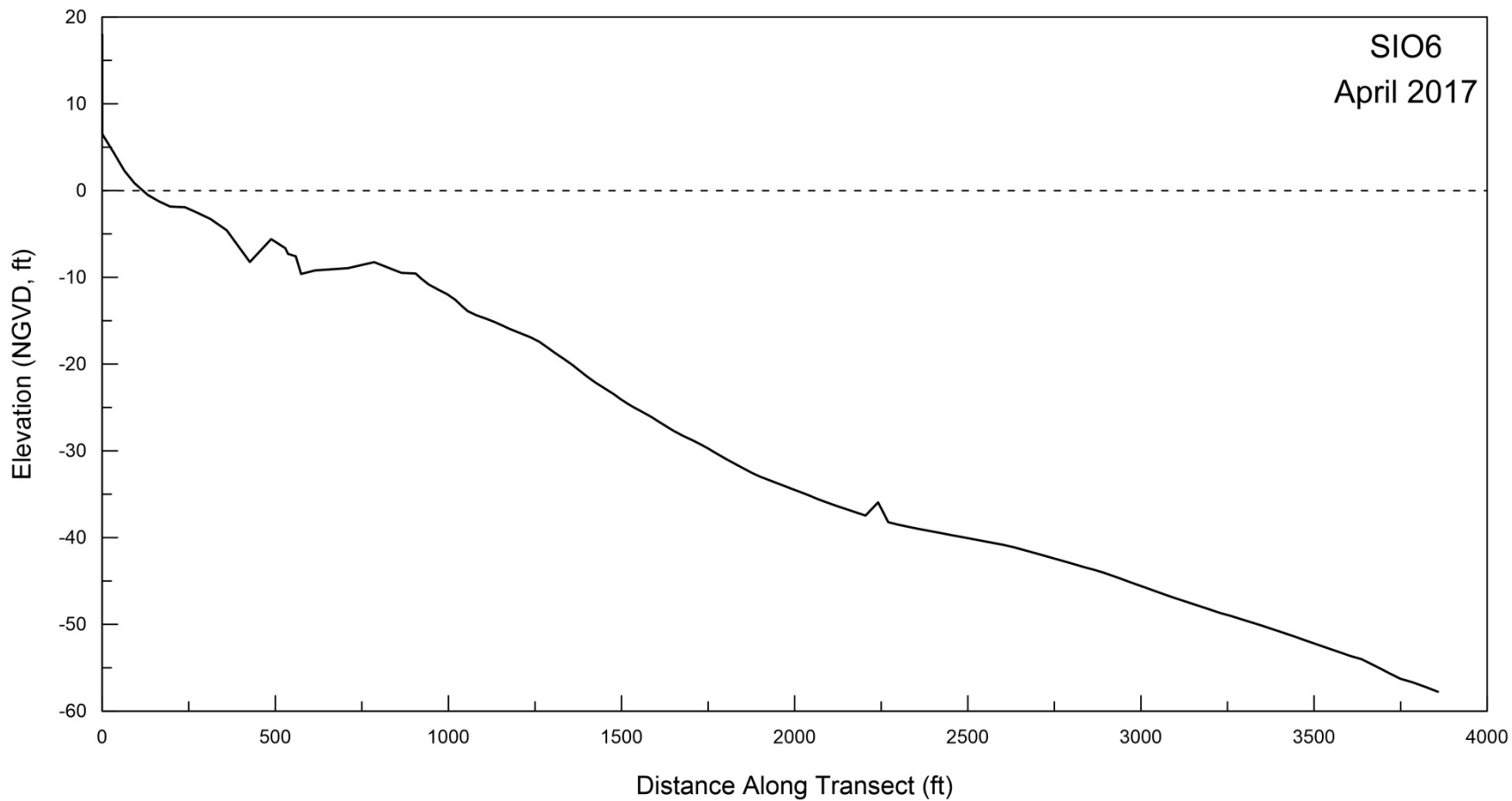
Figure A-4. Beach profile for SIO6 surveyed on 05 April 2017.
