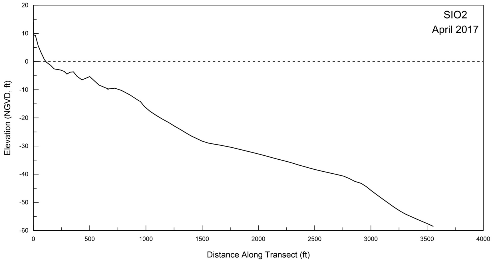
Figure A-2. Beach profile for SIO2 surveyed on 05 April 2017.
