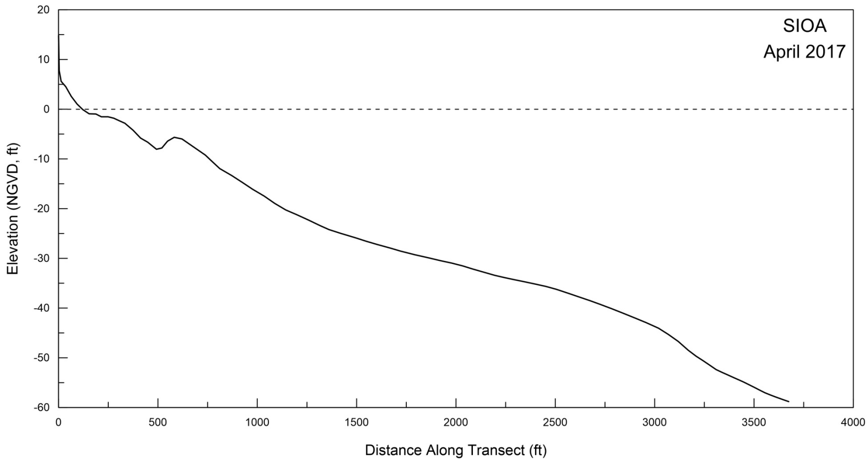
Figure A-5. Beach profile for SIOA surveyed on 05 April 2017.
