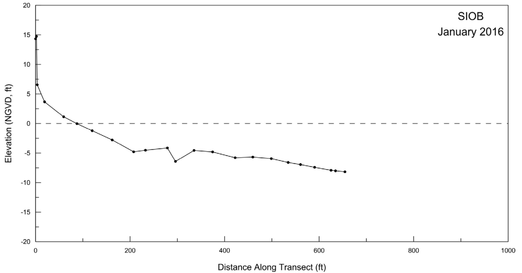
Figure A-6. Beach profile for SIOB surveyed on 21 January 2016.
