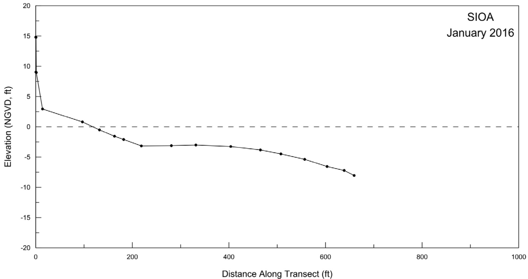
Figure A-5. Beach profile for SIOA surveyed on 21 January 2016.
