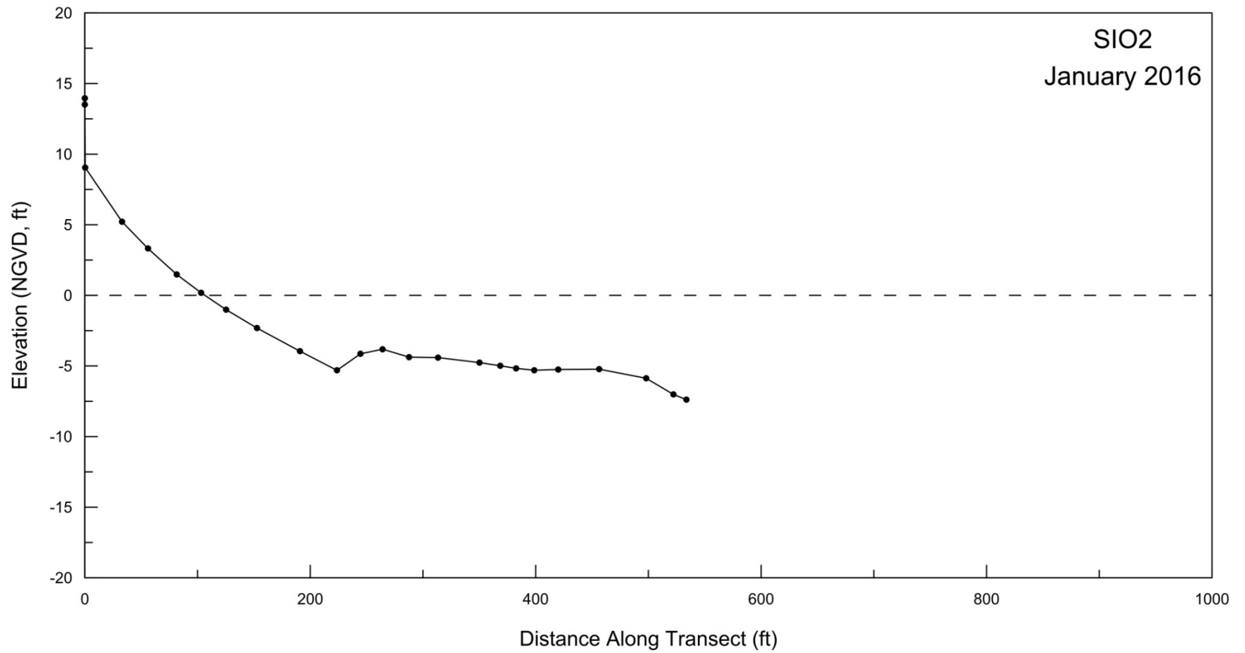
Figure A-2. Beach profile for SIO2 surveyed on 21 January 2016.
