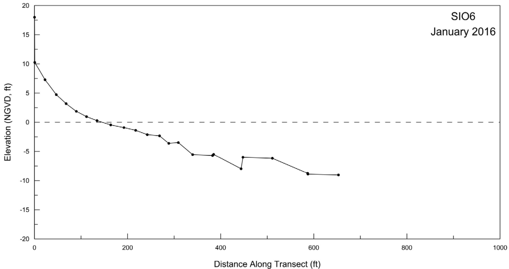
Figure A-4. Beach profile for SIO6 surveyed on 21 January 2016.
