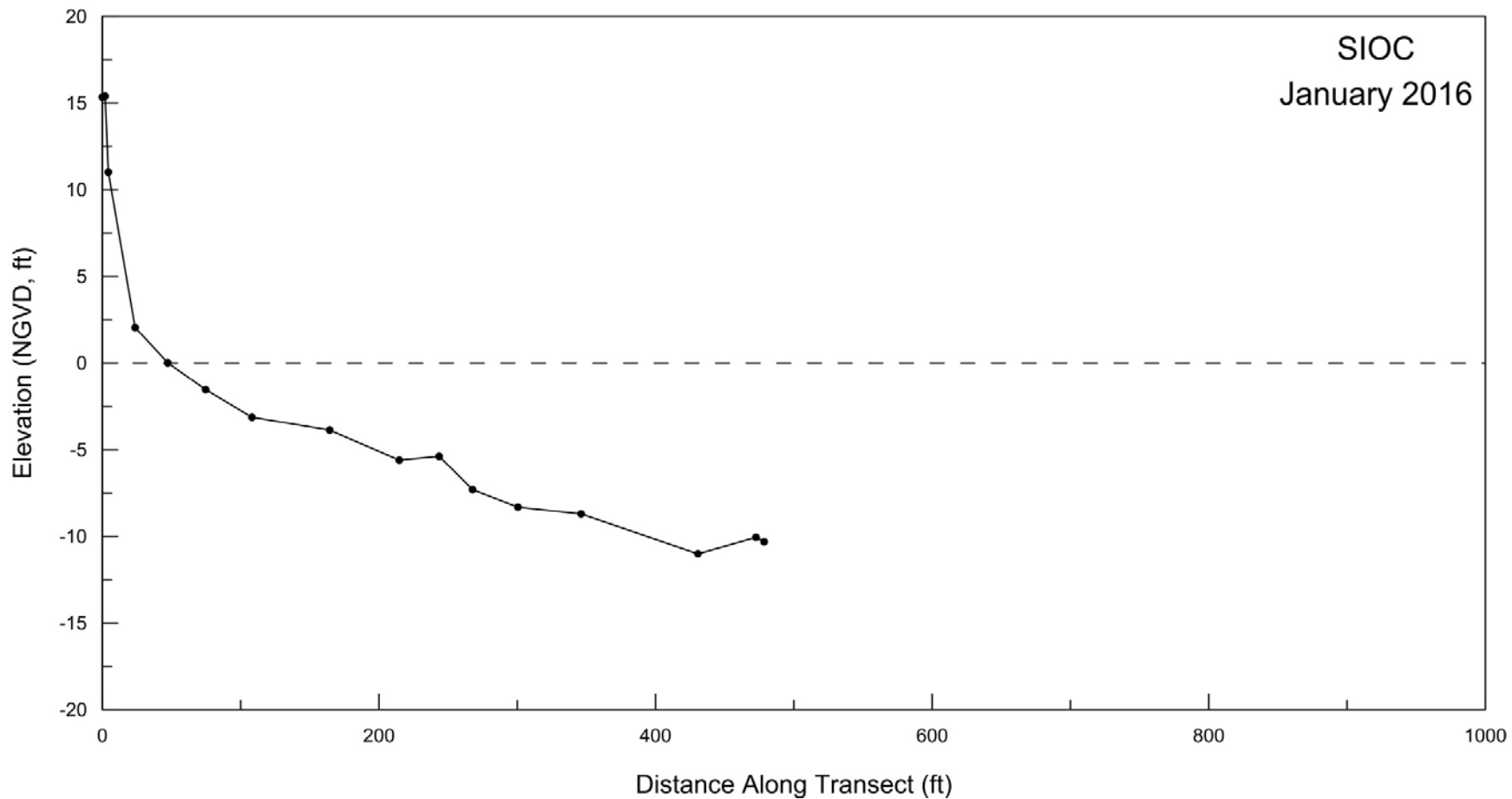
Figure A-7. Beach profile for SIOC surveyed on 21 January 2016.
