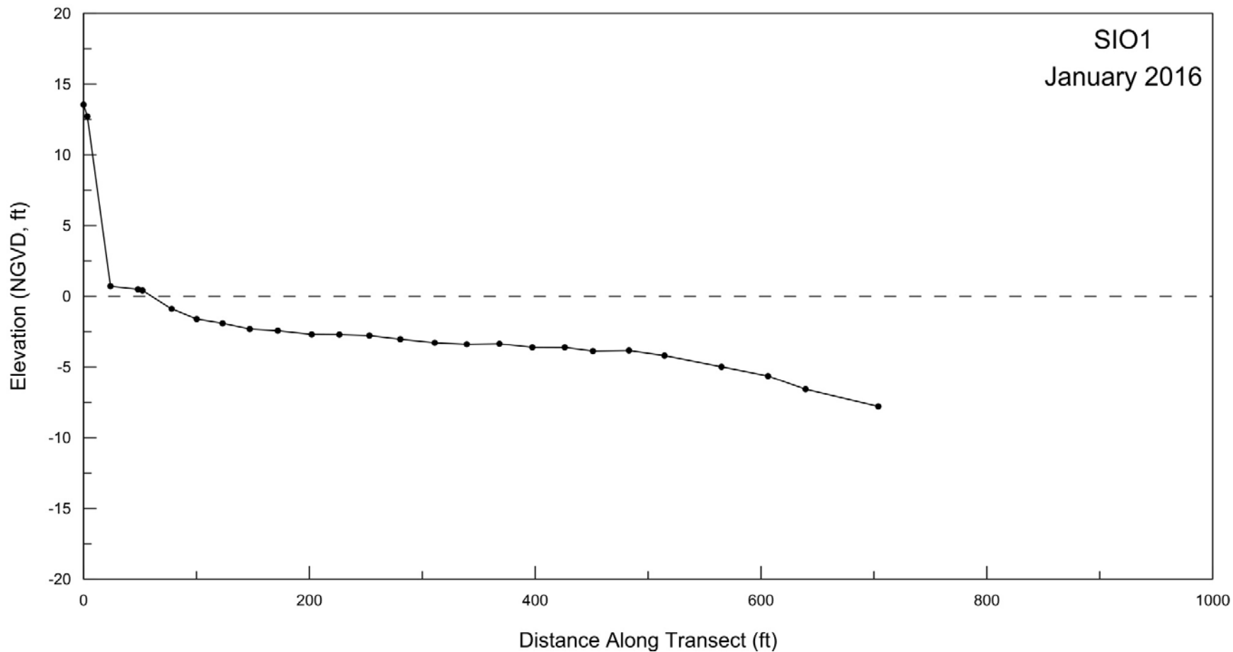
Figure A-1. Beach profile for SIO1 surveyed on 21 January 2016.
