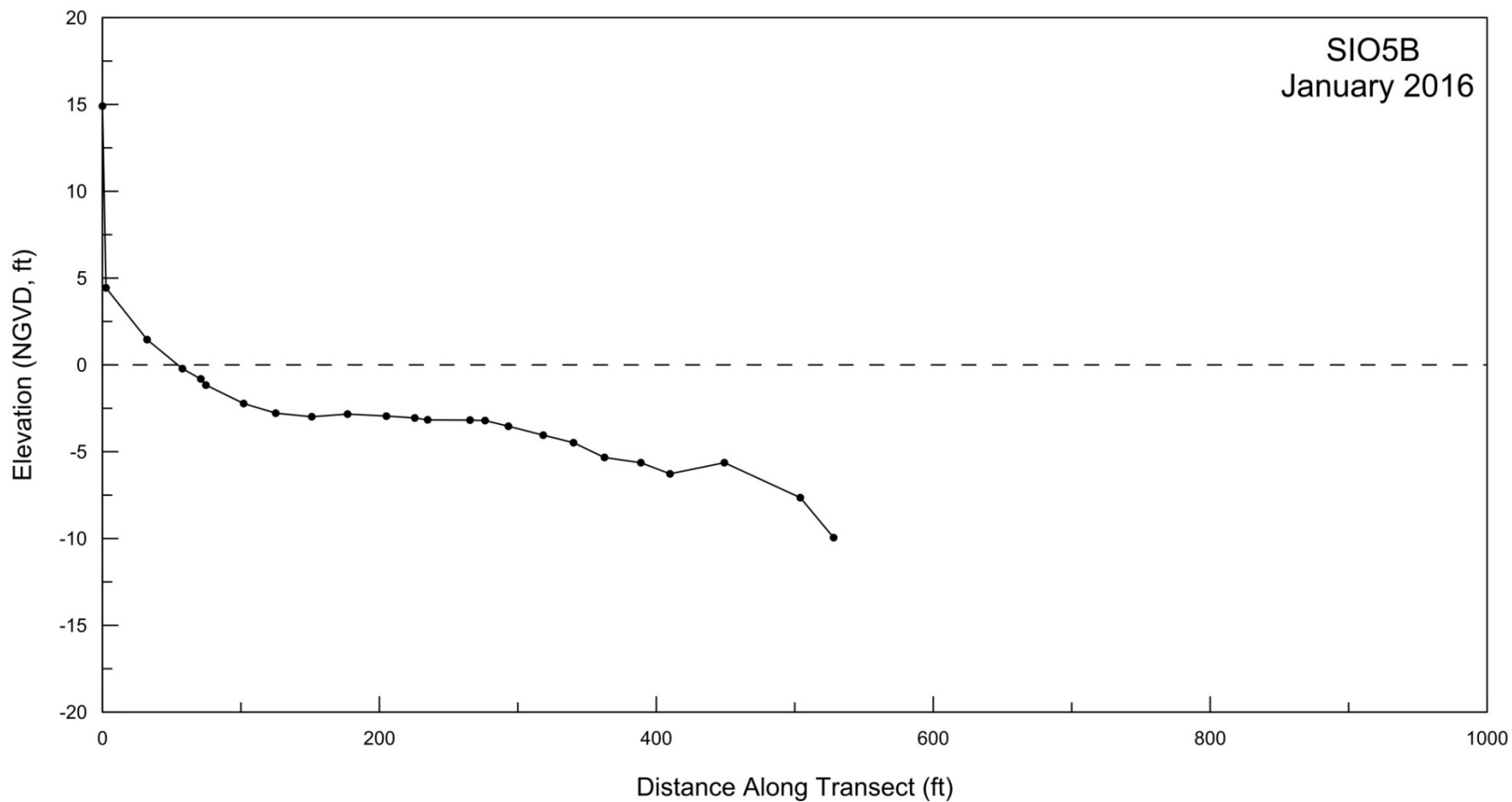
Figure A-3. Beach profile for SIO5B surveyed on 21 January 2016.
