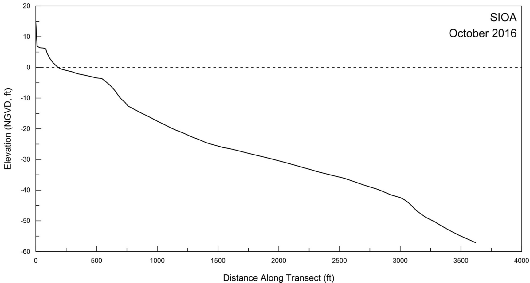
Figure A-5. Beach profile for SIOA surveyed on 06 October 2016.
