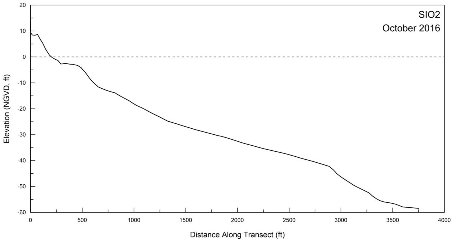
Figure A-2. Beach profile for SIO2 surveyed on 06 October 2016.
