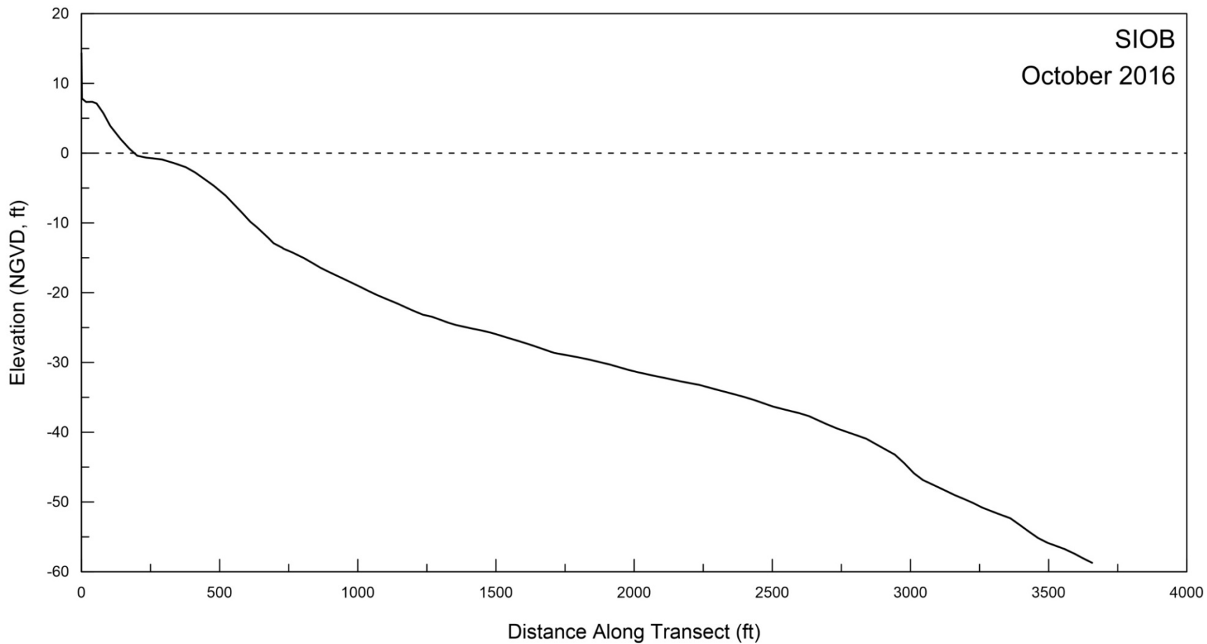
Figure A-6. Beach profile for SIOB surveyed on 06 October 2016.
