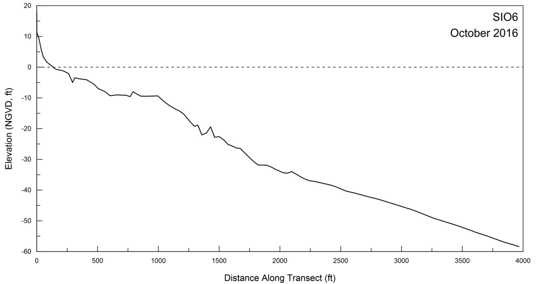
Figure A-4. Beach profile for SIO6 surveyed on 06 October 2016.
