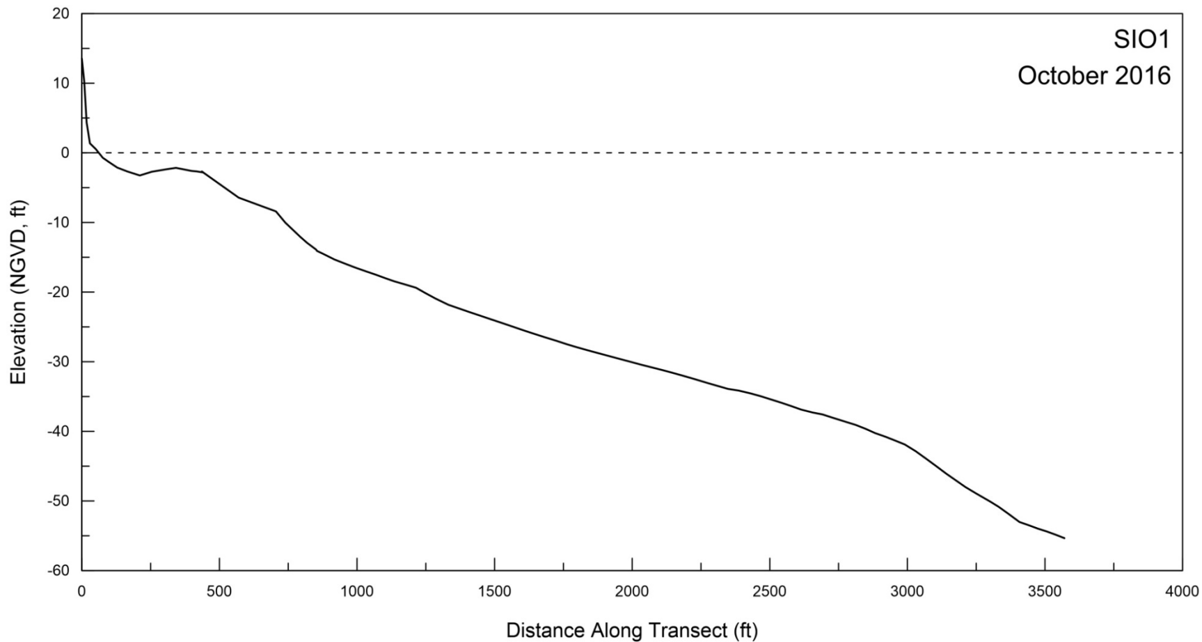
Figure A-1. Beach profile for SIO1 surveyed on 06 October 2016.
