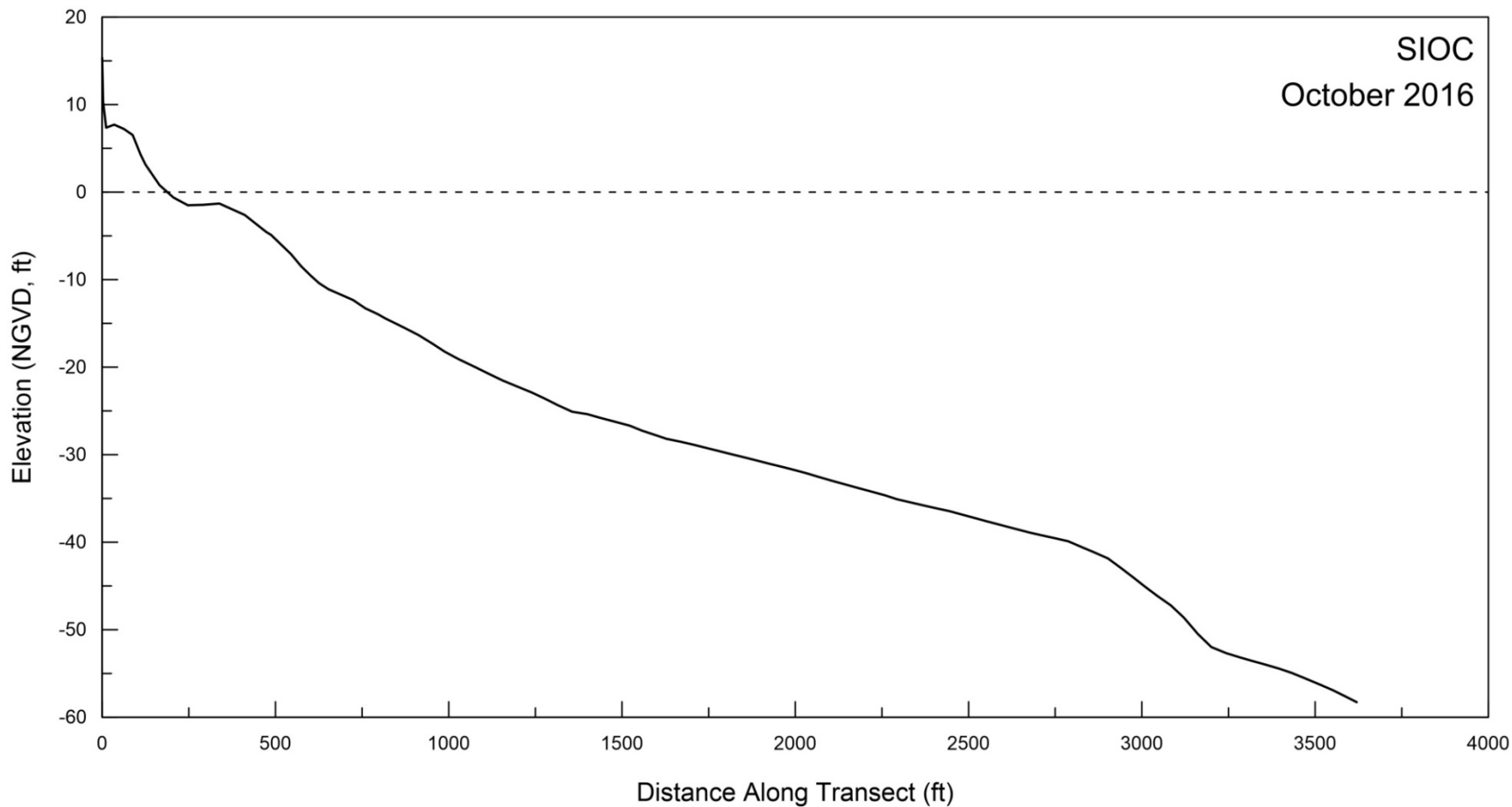
Figure A-7. Beach profile for SIOC surveyed on 06 October 2016.
