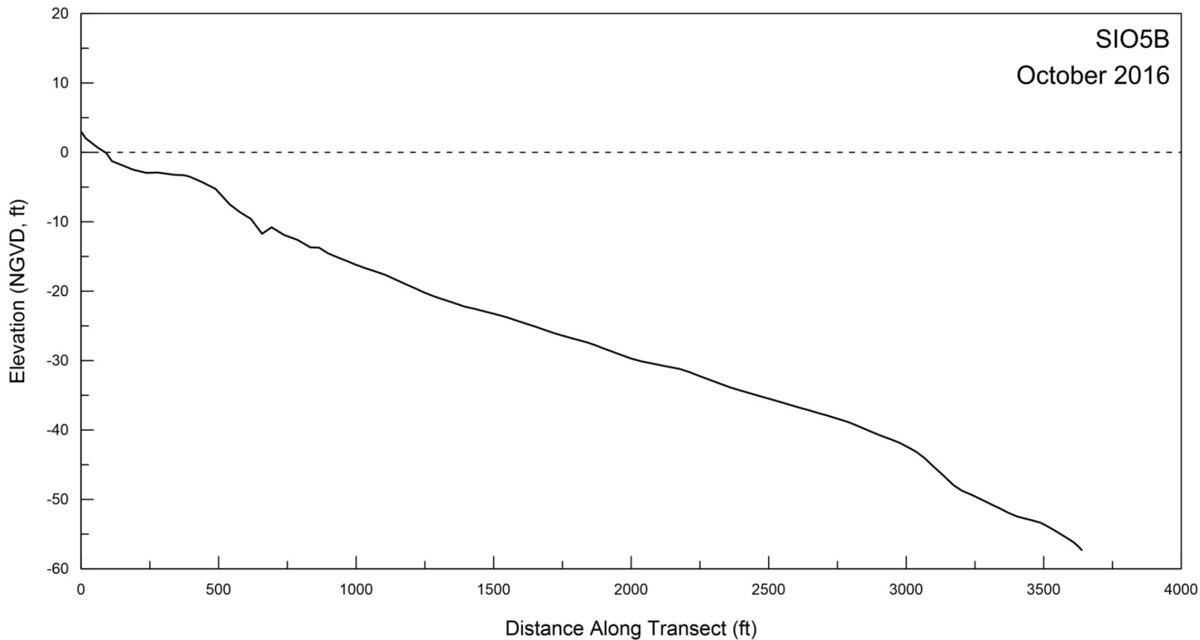
Figure A-3. Beach profile for SIO5B surveyed on 06 October 2016.
