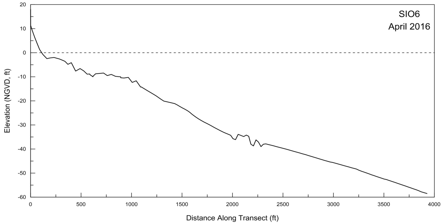
Figure A-4. Beach profile for SIO6 surveyed on 05 April 2016.
