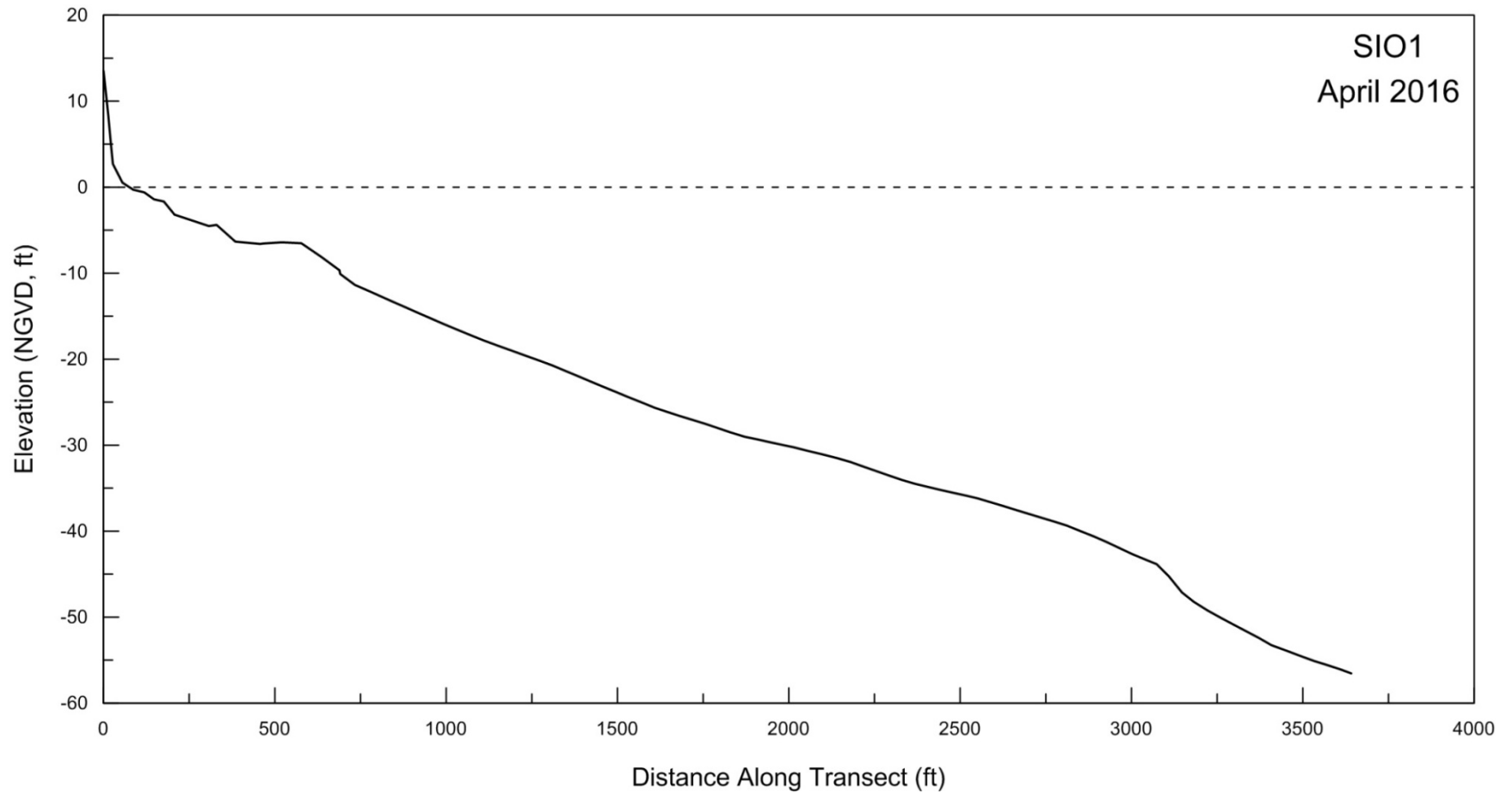
Figure A-1. Beach profile for SIO1 surveyed on 05 April 2016.
