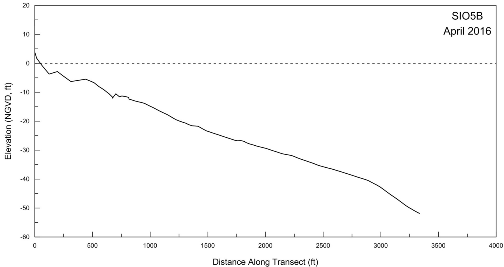
Figure A-3. Beach profile for SIO5B surveyed on 05 April 2016.
