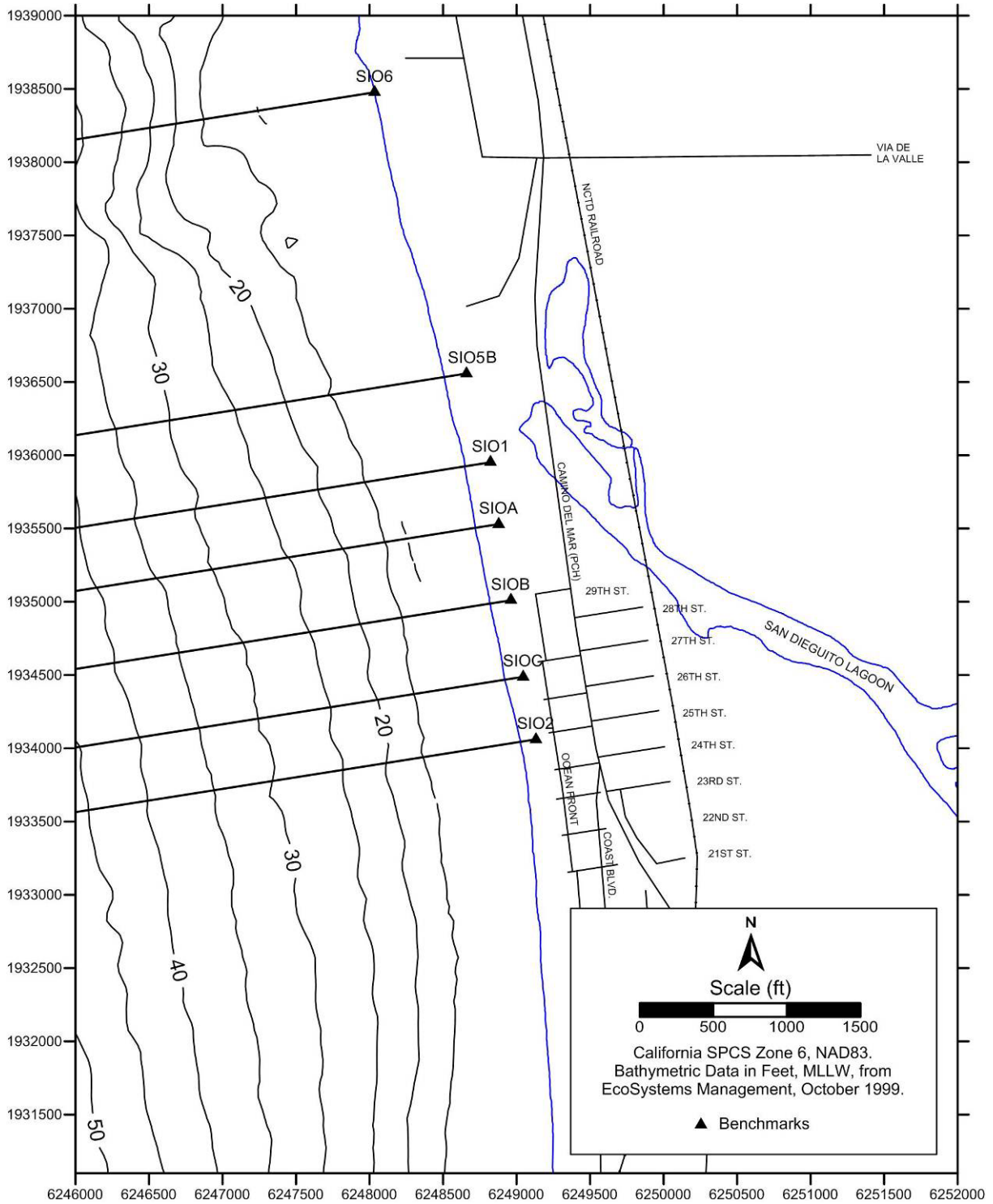
Figure 2. Beach profiles surveyed on 05 April 2016.
