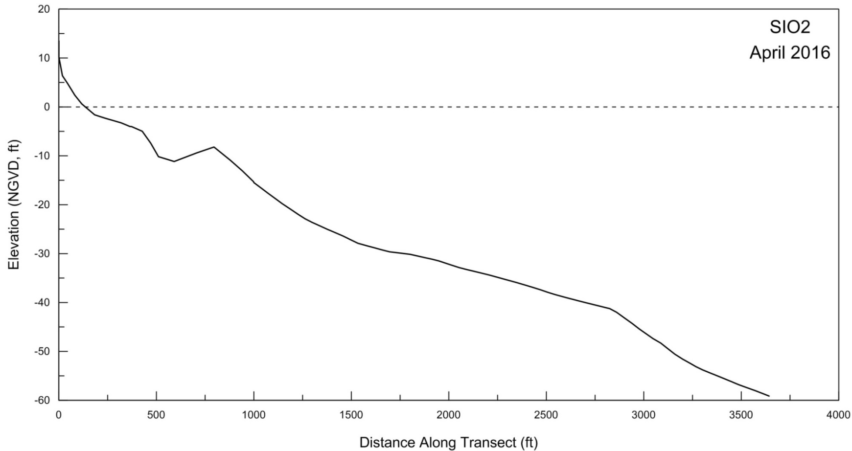
Figure A-2. Beach profile for SIO2 surveyed on 05 April 2016.
