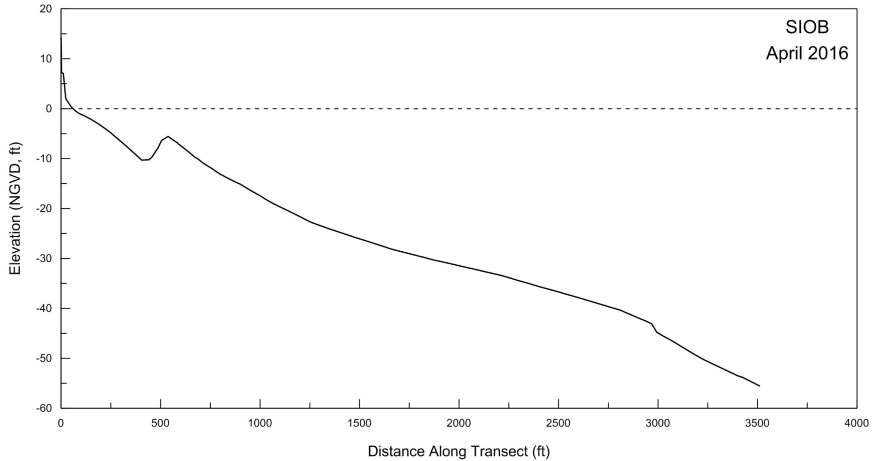
Figure A-6. Beach profile for SIOB surveyed on 05 April 2016.
