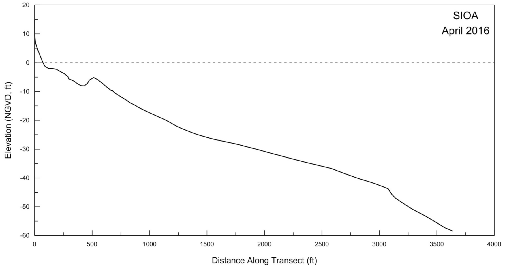
Figure A-5. Beach profile for SIOA surveyed on 05 April 2016.
