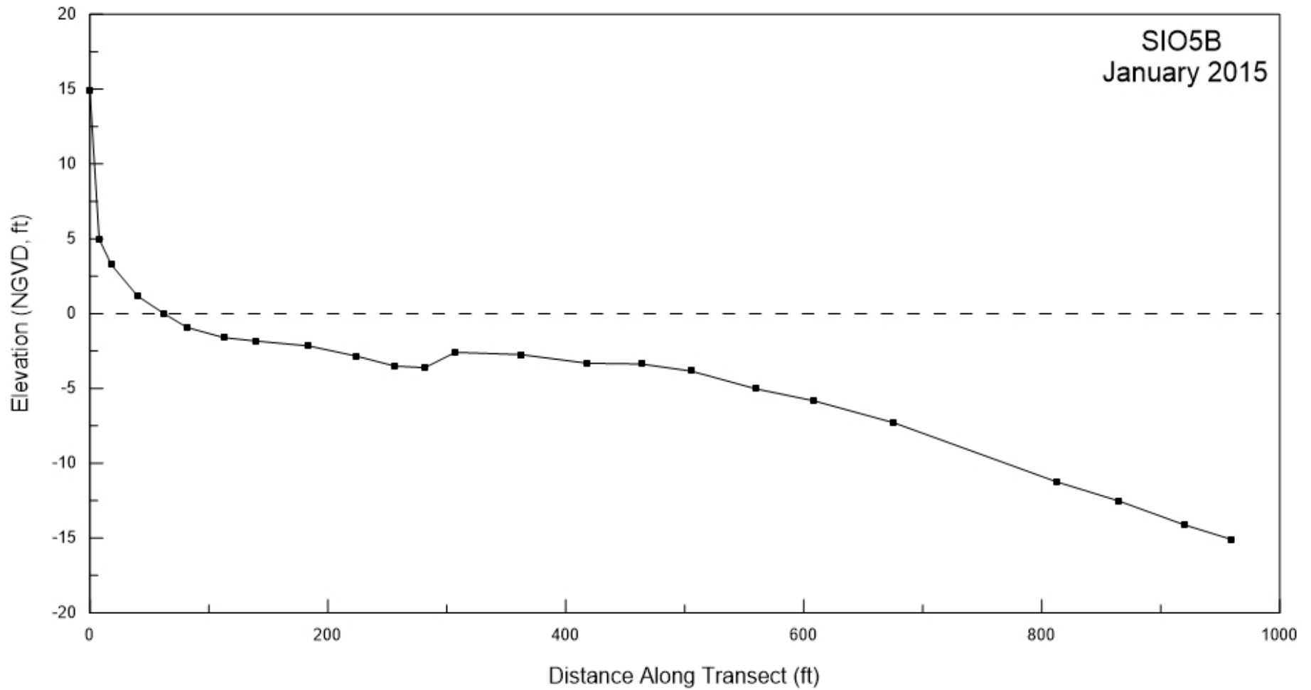
Figure A-3. Beach profile for SIO5B surveyed on 14 January 2015.
