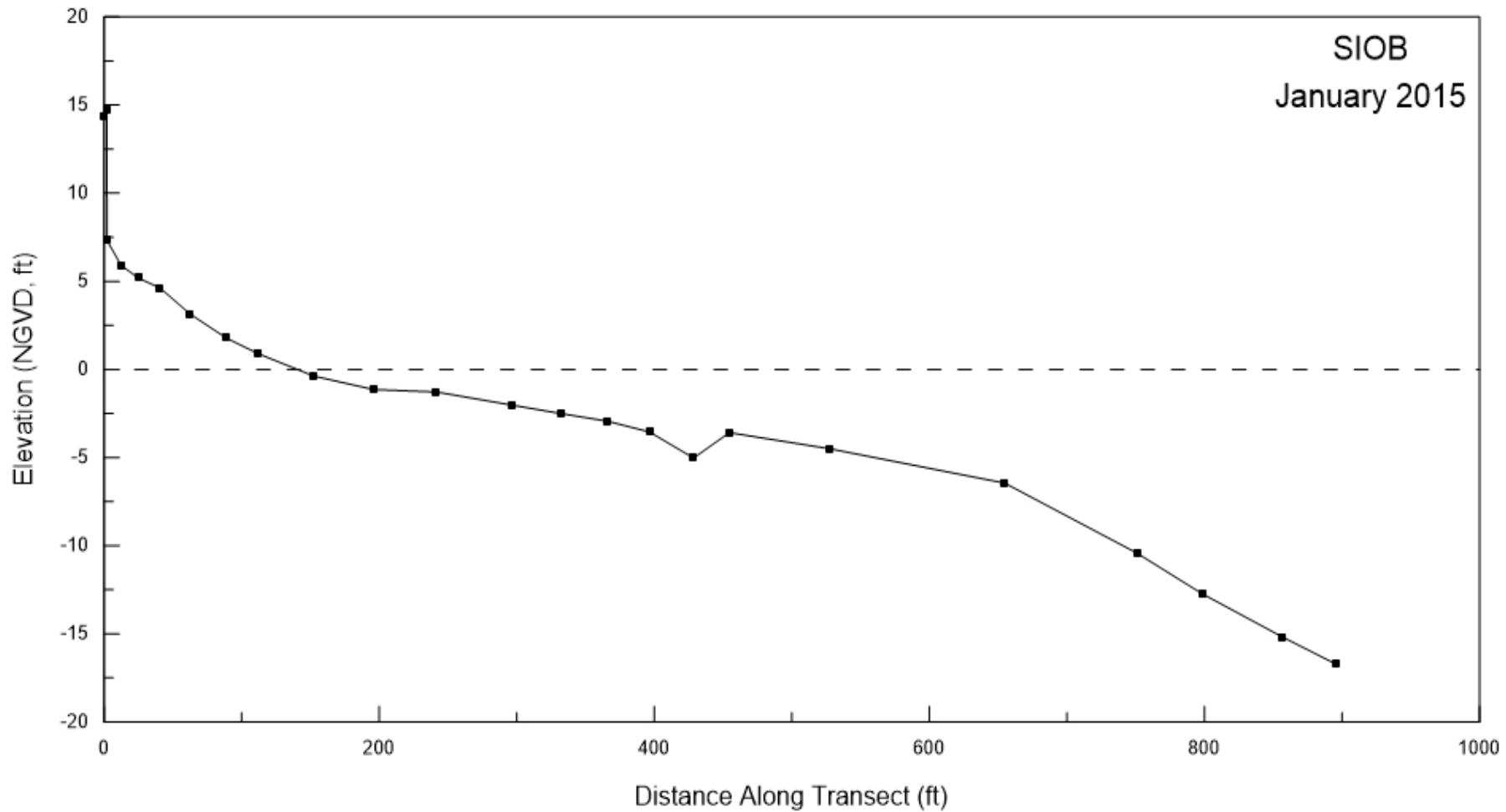
Figure A-6. Beach profile for SIOB surveyed on 14 January 2015.
