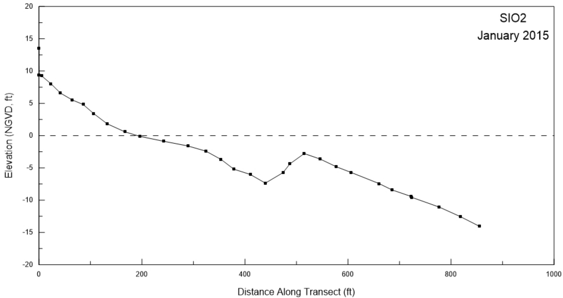
Figure A-2. Beach profile for SIO2 surveyed on 14 January 2015.
