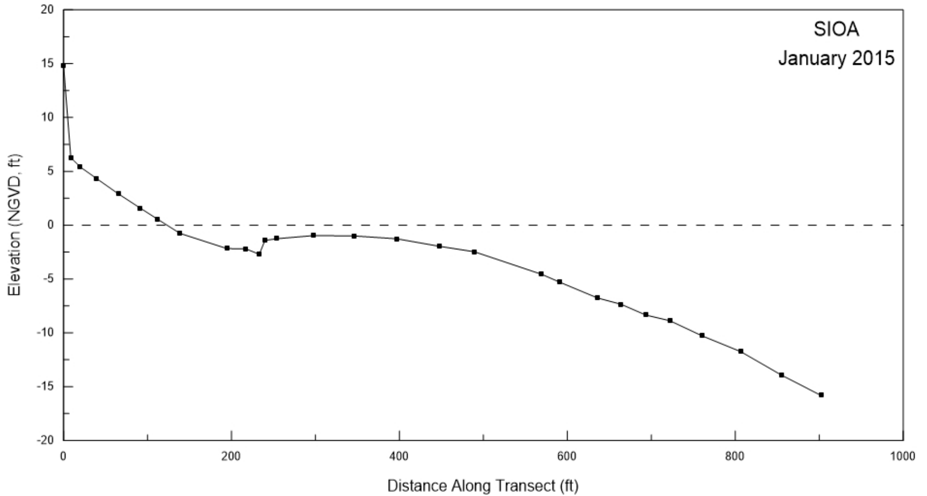
Figure A-5. Beach profile for SIOA surveyed on 14 January 2015.
