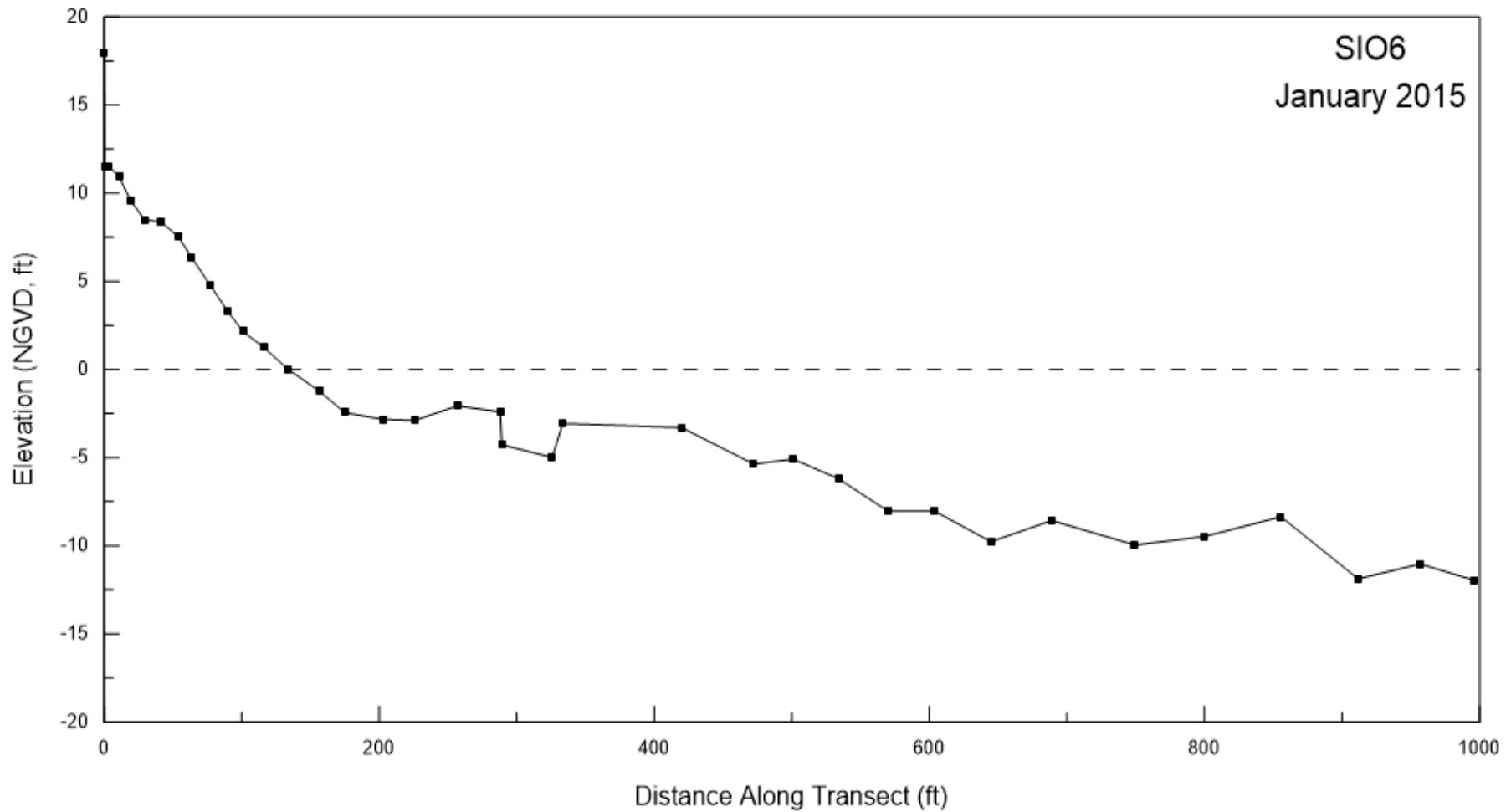
Figure A-4. Beach profile for SIO6 surveyed on 14 January 2015.
