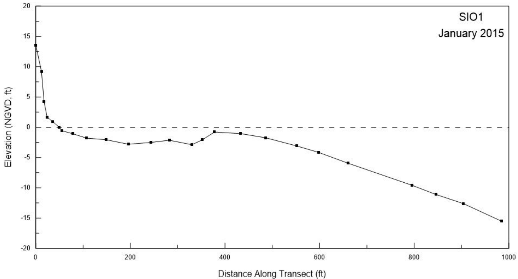
Figure A-1. Beach profile for SIO1 surveyed on 14 January 2015.
