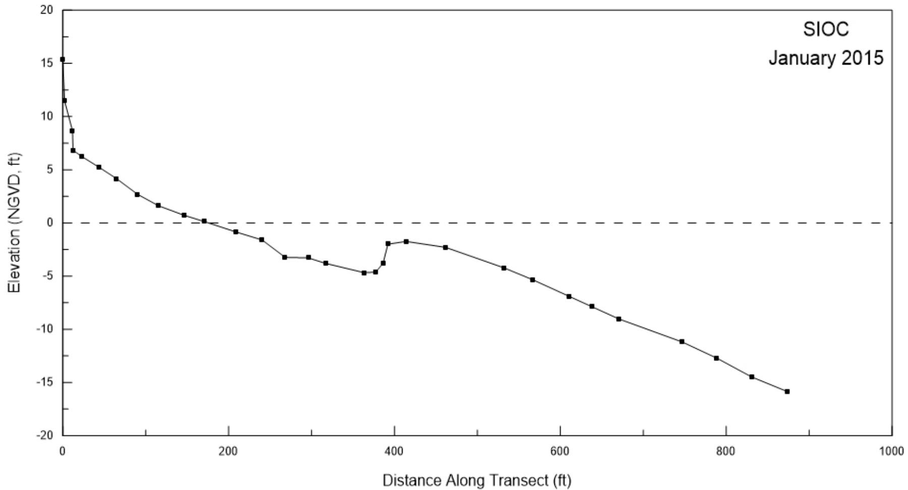
Figure A-7. Beach profile for SIOC surveyed on 14 January 2015.
