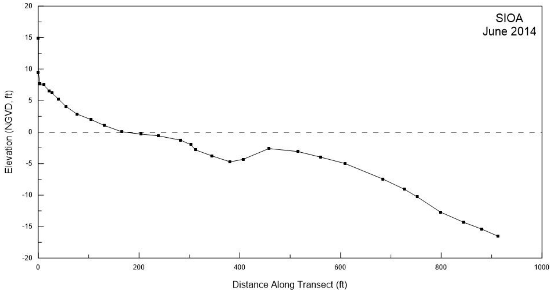
Figure A-5. Beach profile for SIOA surveyed in June 2014.
