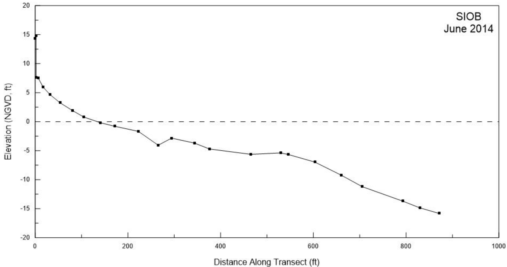
Figure A-6. Beach profile for SIOB surveyed in June 2014.
