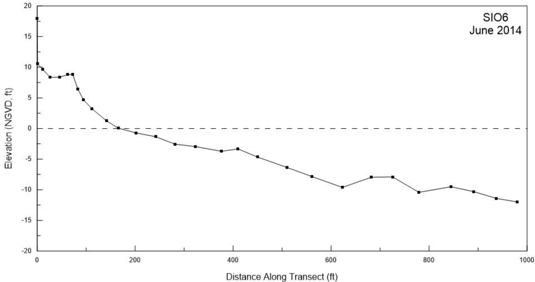
Figure A-4. Beach profile for SIO6 surveyed in June 2014.
