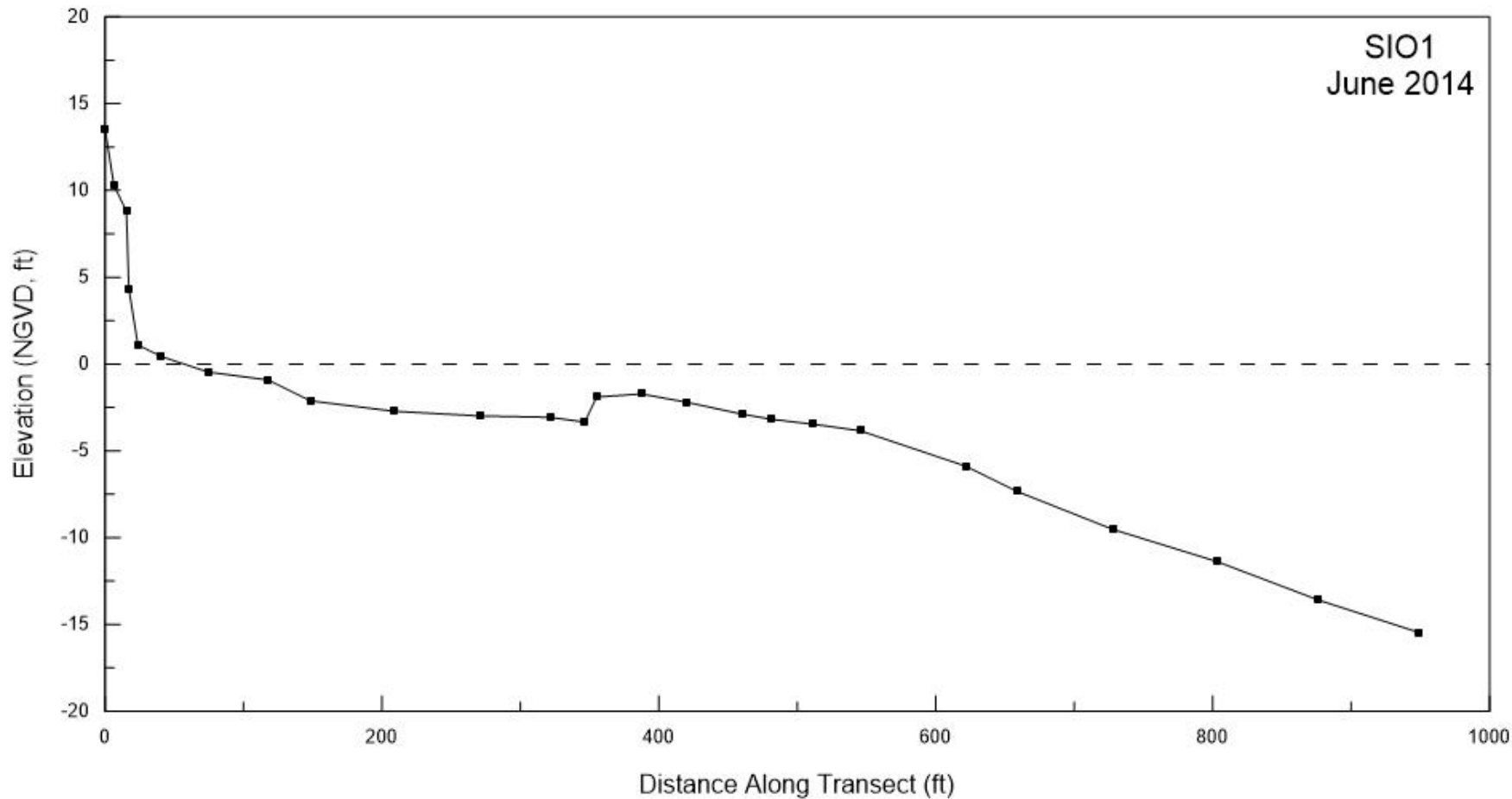
Figure A-1. Beach profile for SIO1 surveyed in June 2014.
