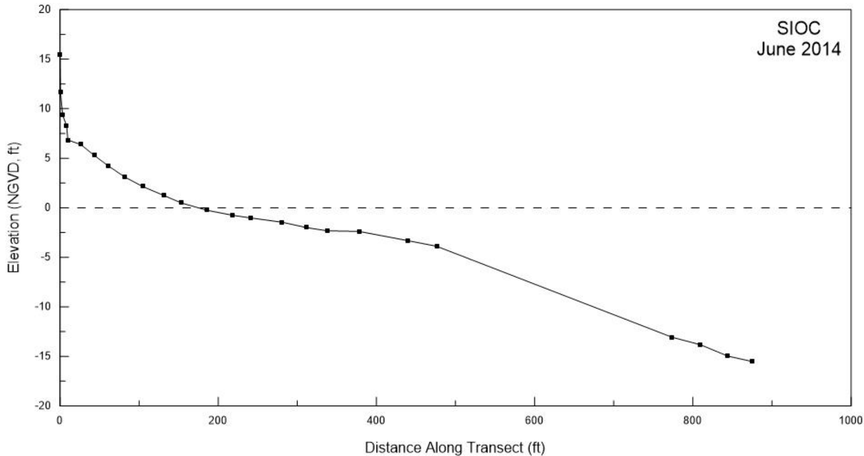
Figure A-7. Beach profile for SIOC surveyed in June 2014.
