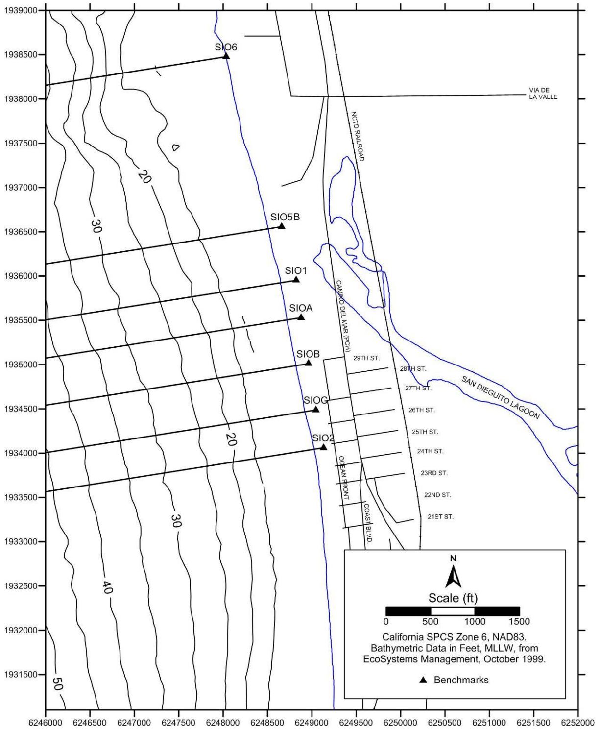
Figure 2. Beach profiles surveyed on 24 June 2014.
