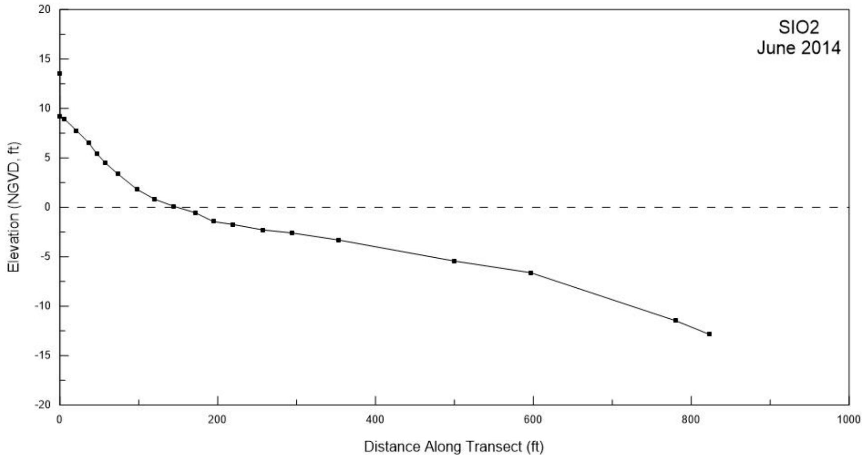
Figure A-2. Beach profile for SIO2 surveyed in June 2014.
