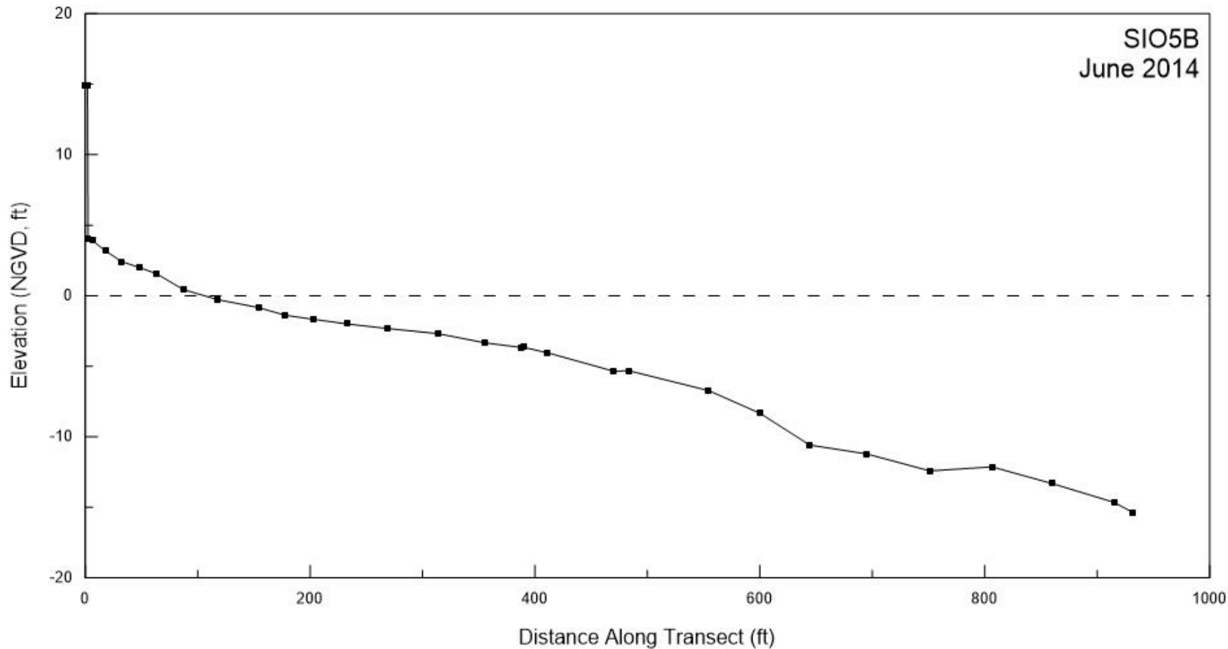
Figure A-3. Beach profile for SIO5B surveyed in June 2014.
