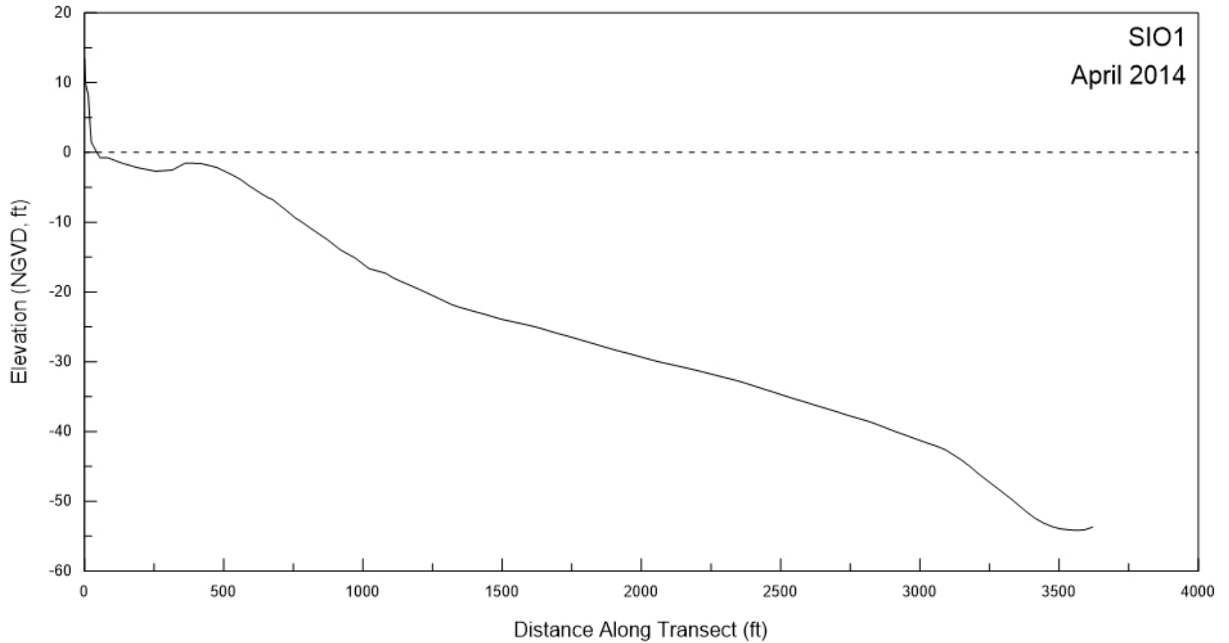
Figure A-1. Beach profile for SIO1 surveyed in April 2014.
