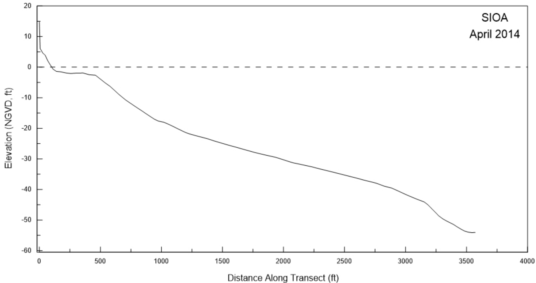
Figure A-5. Beach profile for SIOA surveyed in April 2014.
