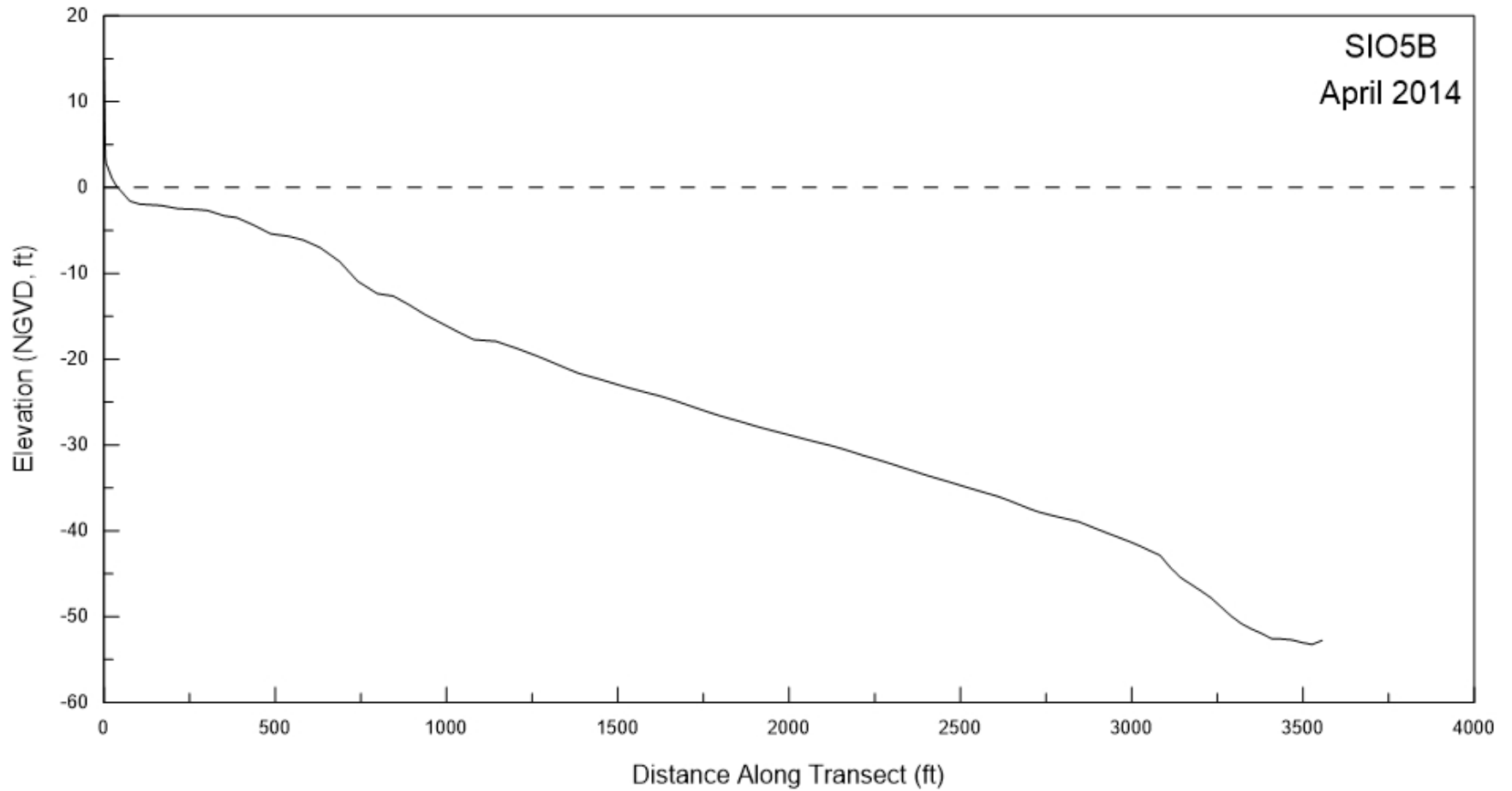
Figure A-3. Beach profile for SIO5B surveyed in April 2014.
