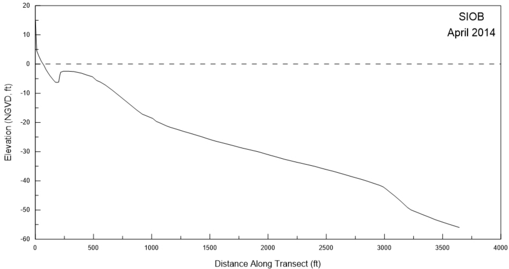
Figure A-6. Beach profile for SIOB surveyed in April 2014.
