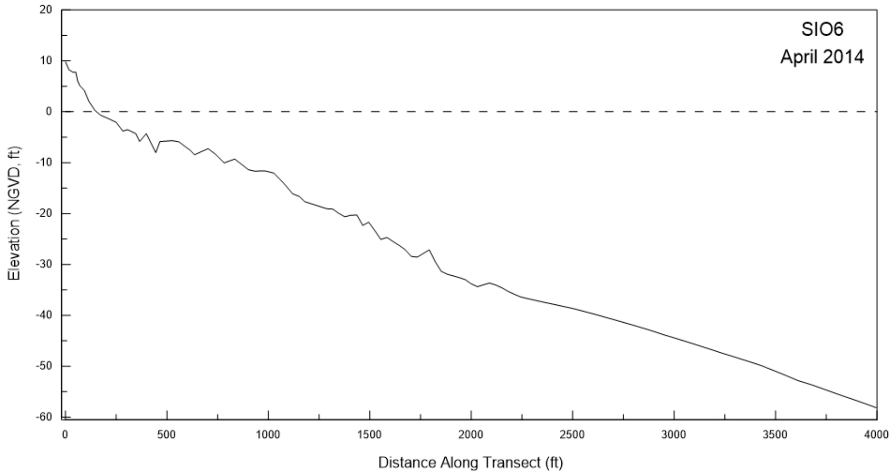
Figure A-4. Beach profile for SIO6 surveyed in April 2014.
