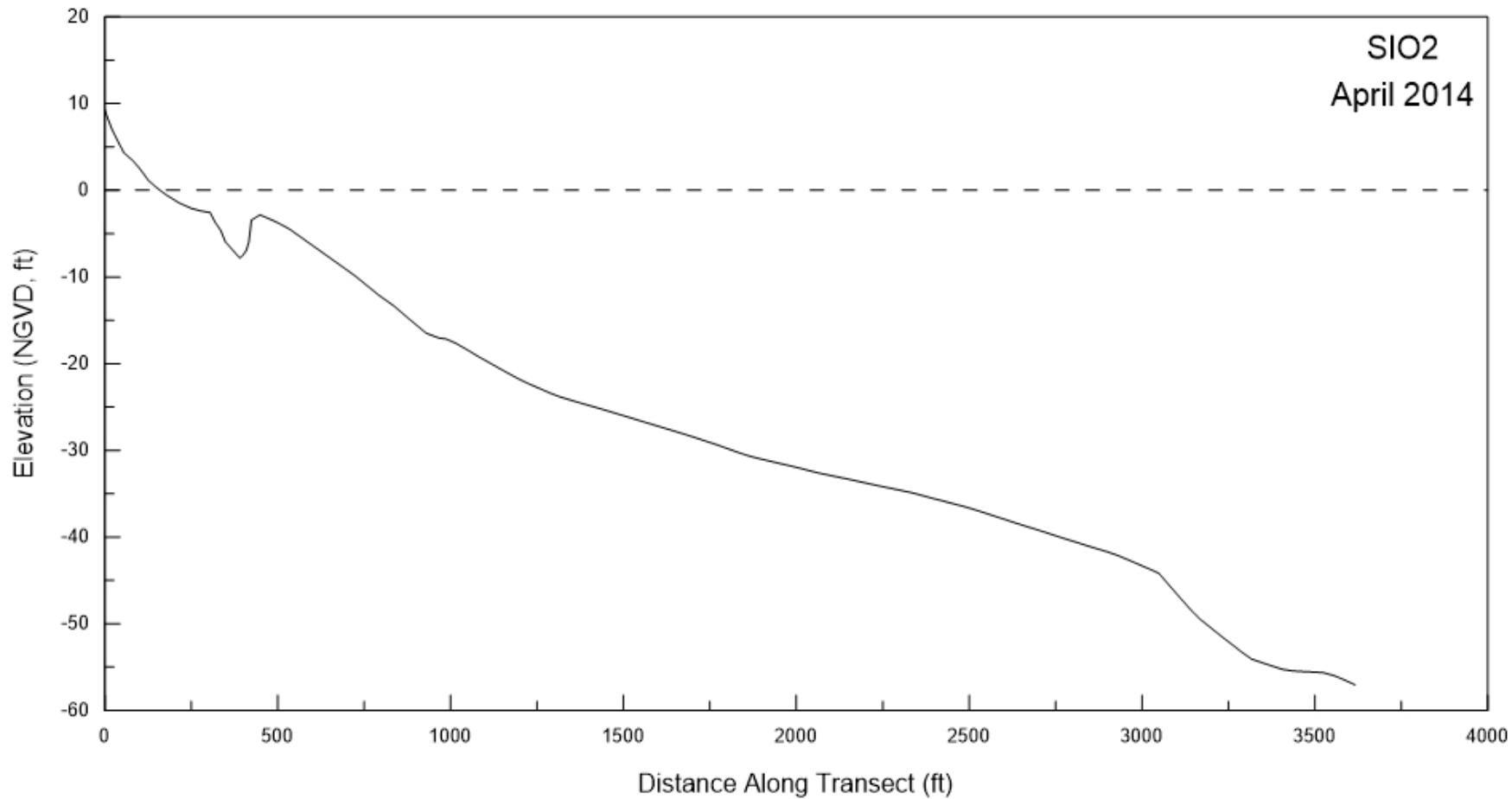
Figure A-2. Beach profile for SIO2 surveyed in April 2014.
