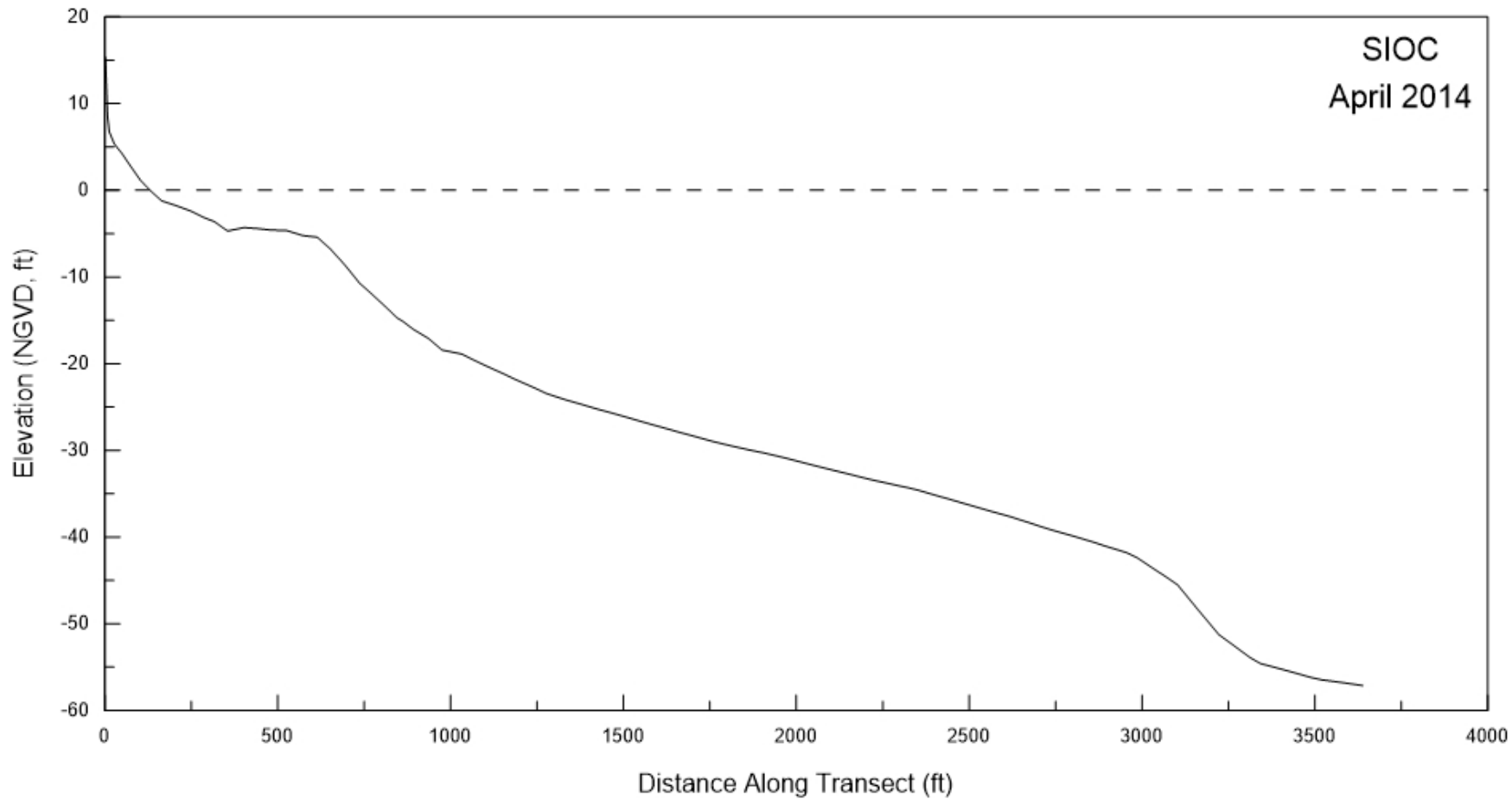
Figure A-7. Beach profile for SIOC surveyed in April 2014.
