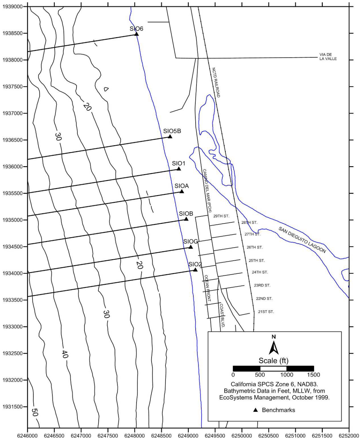
Figure 2. Beach profiles surveyed on 05 November 2014.
