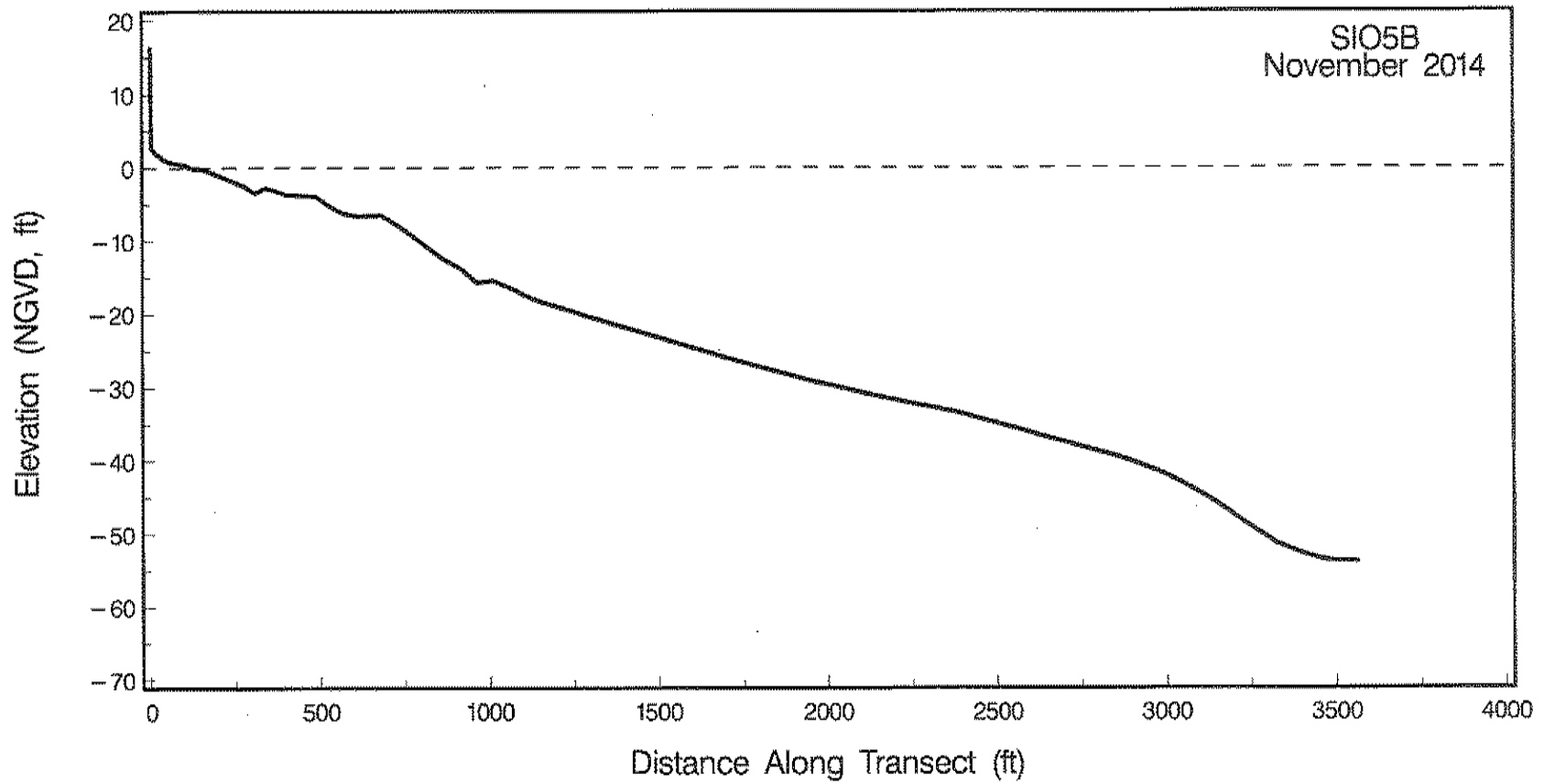
Figure A-3. Beach profile for SIO5B surveyed in November 2014.
