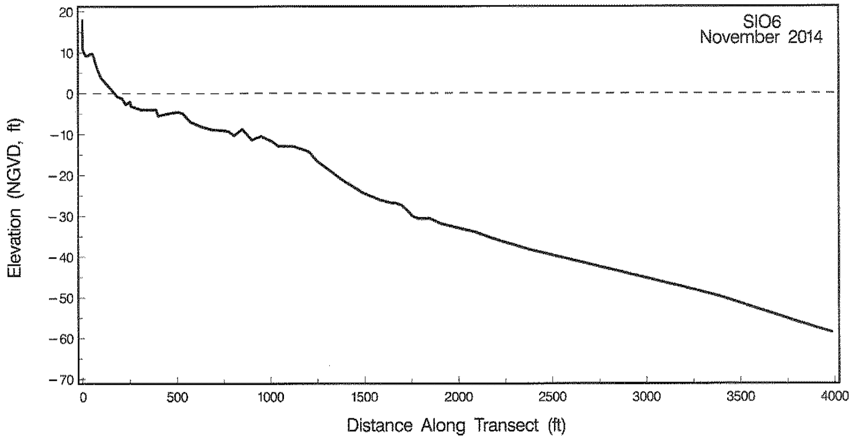
Figure A-4. Beach profile for SIO6 surveyed in November 2014.
