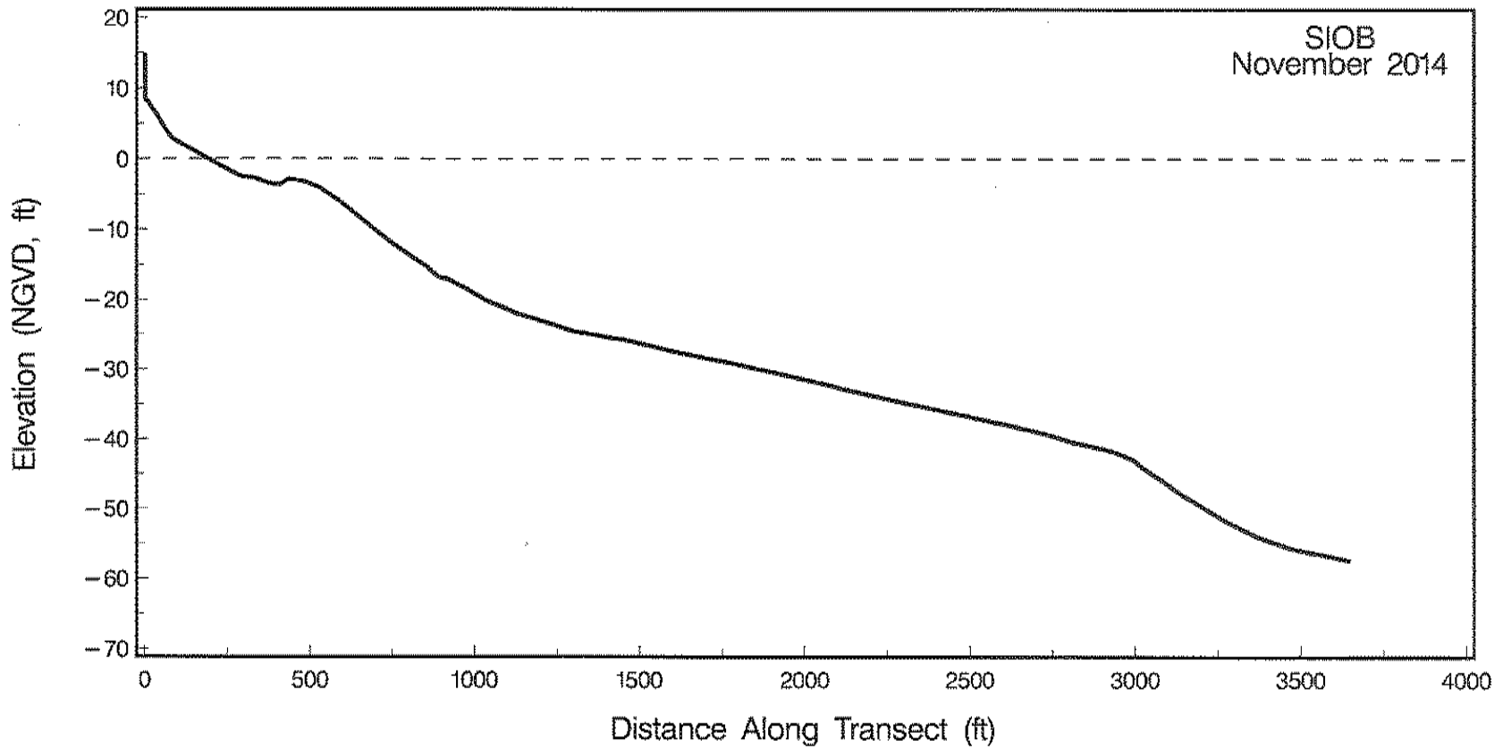
Figure A-6. Beach profile for SIOB surveyed in November 2014.
