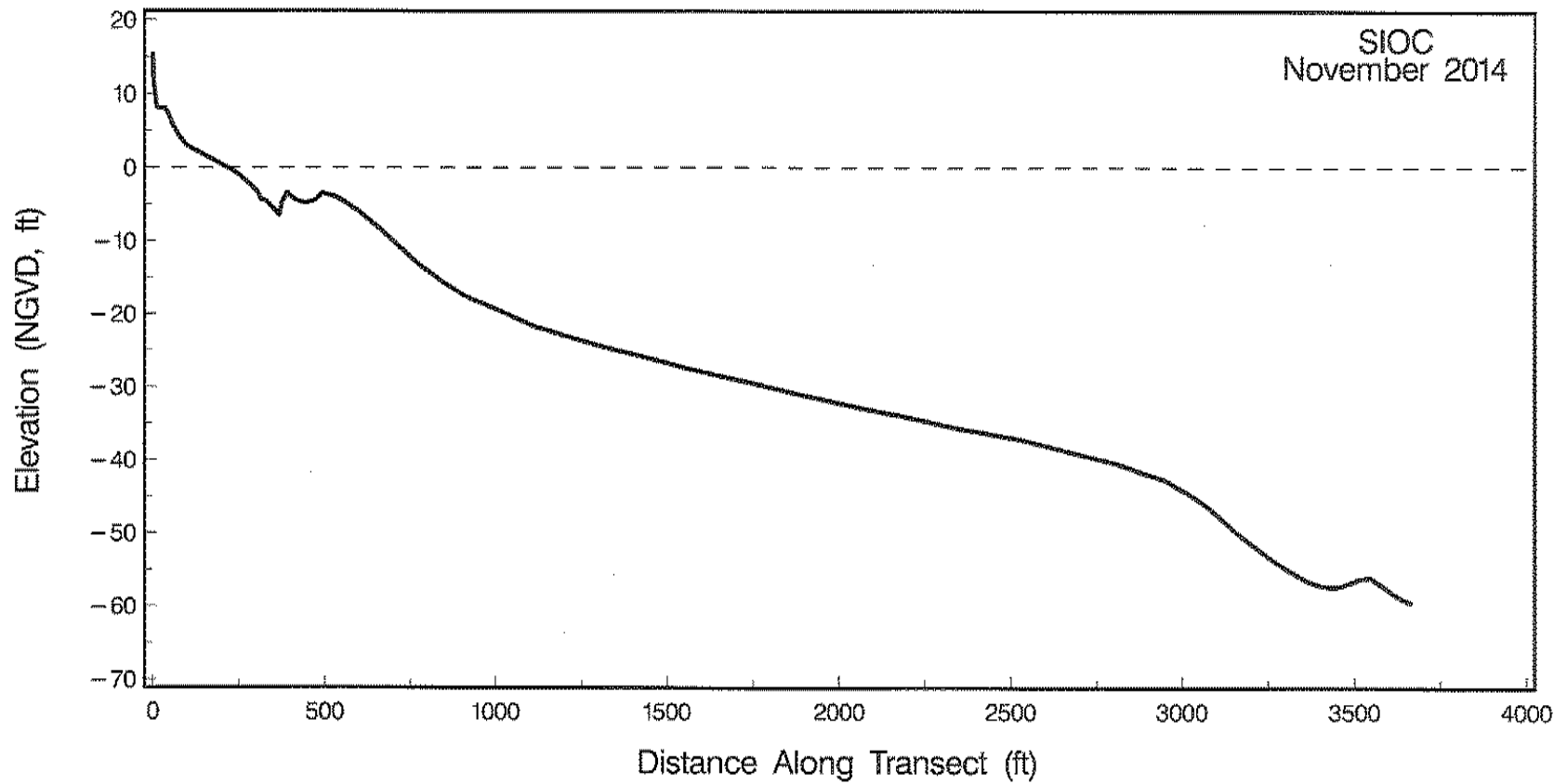
Figure A-7. Beach profile for SIOC surveyed in November 2014.
