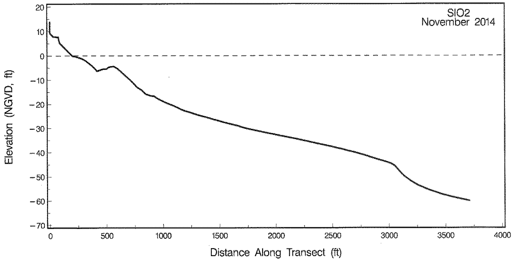
Figure A-2. Beach profile for SIO2 surveyed in November 2014.
