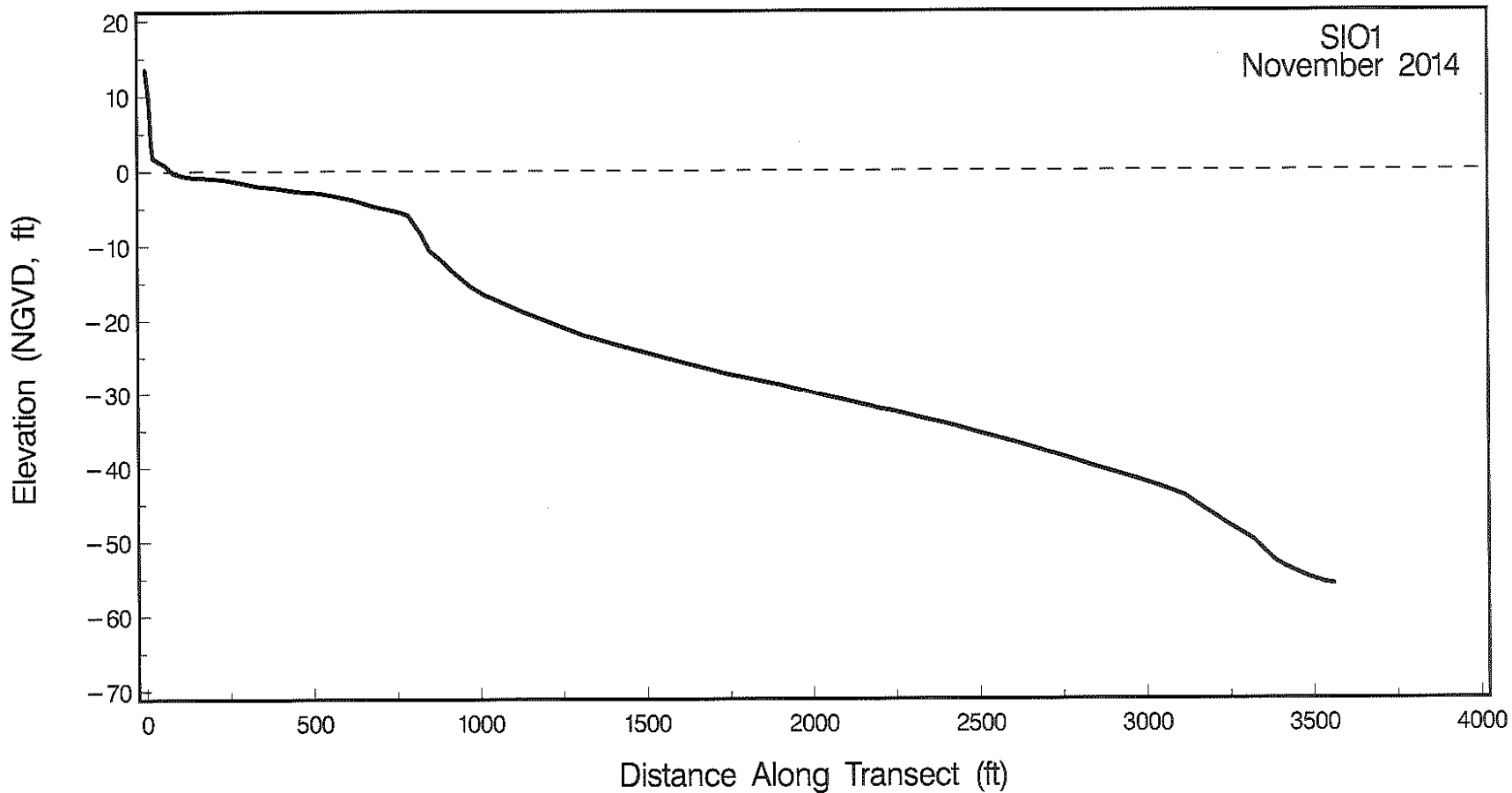
Figure A-1. Beach profile for SIO1 surveyed in November 2014.
