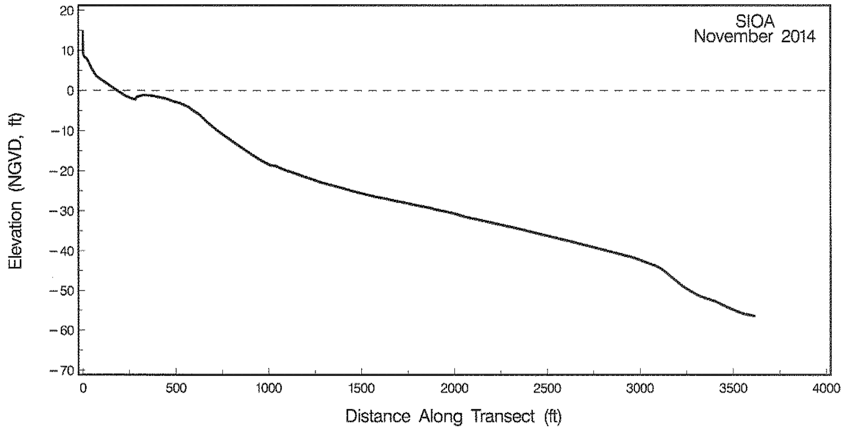
Figure A-5. Beach profile for SIOA surveyed in November 2014.
