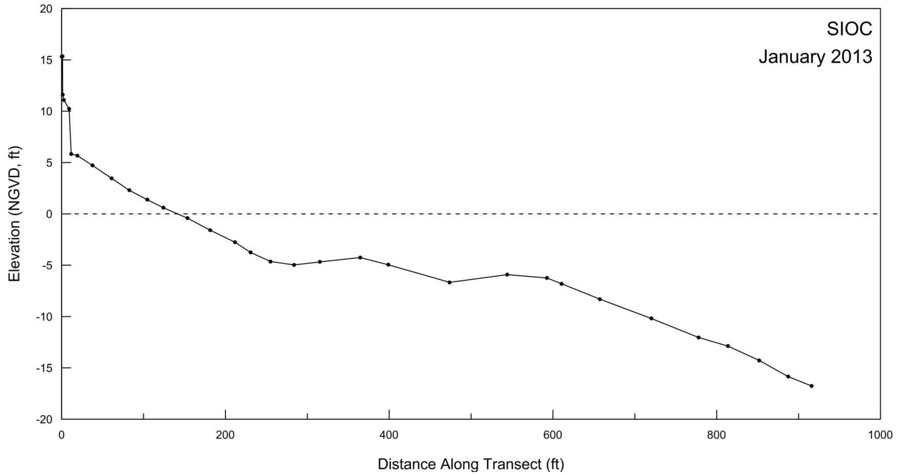
Figure A-7. Beach profile for SIOC surveyed on 23 January 2013.
