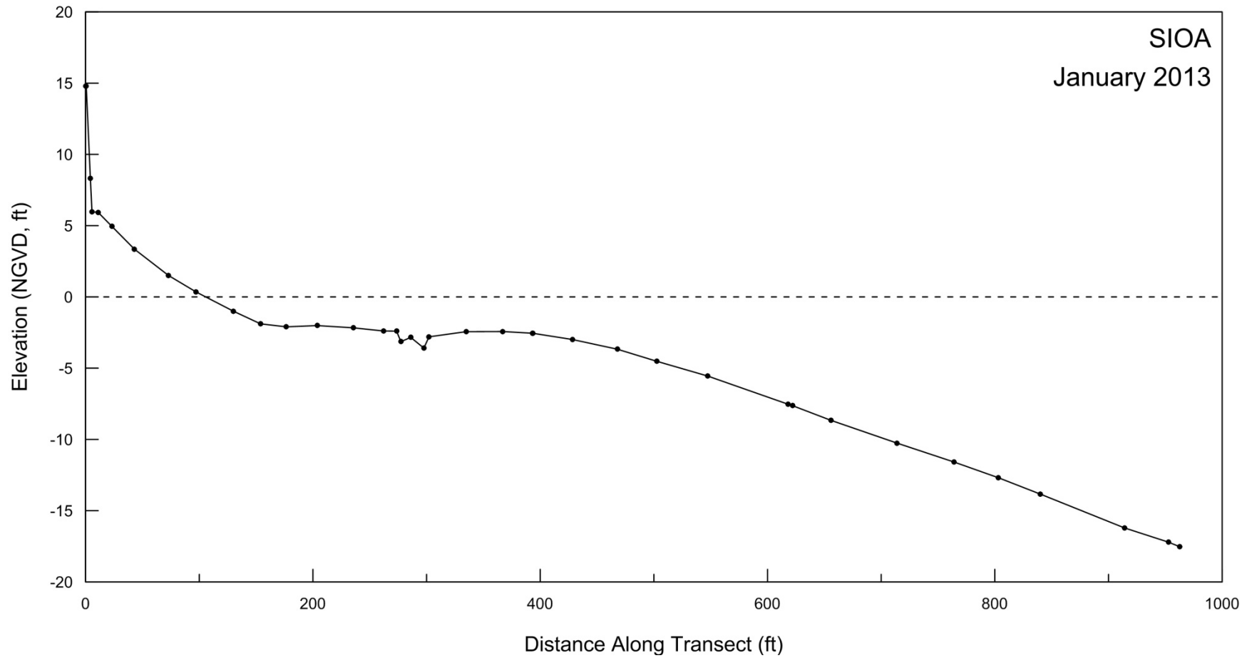
Figure A-5. Beach profile for SIOA surveyed on 23 January 2013.
