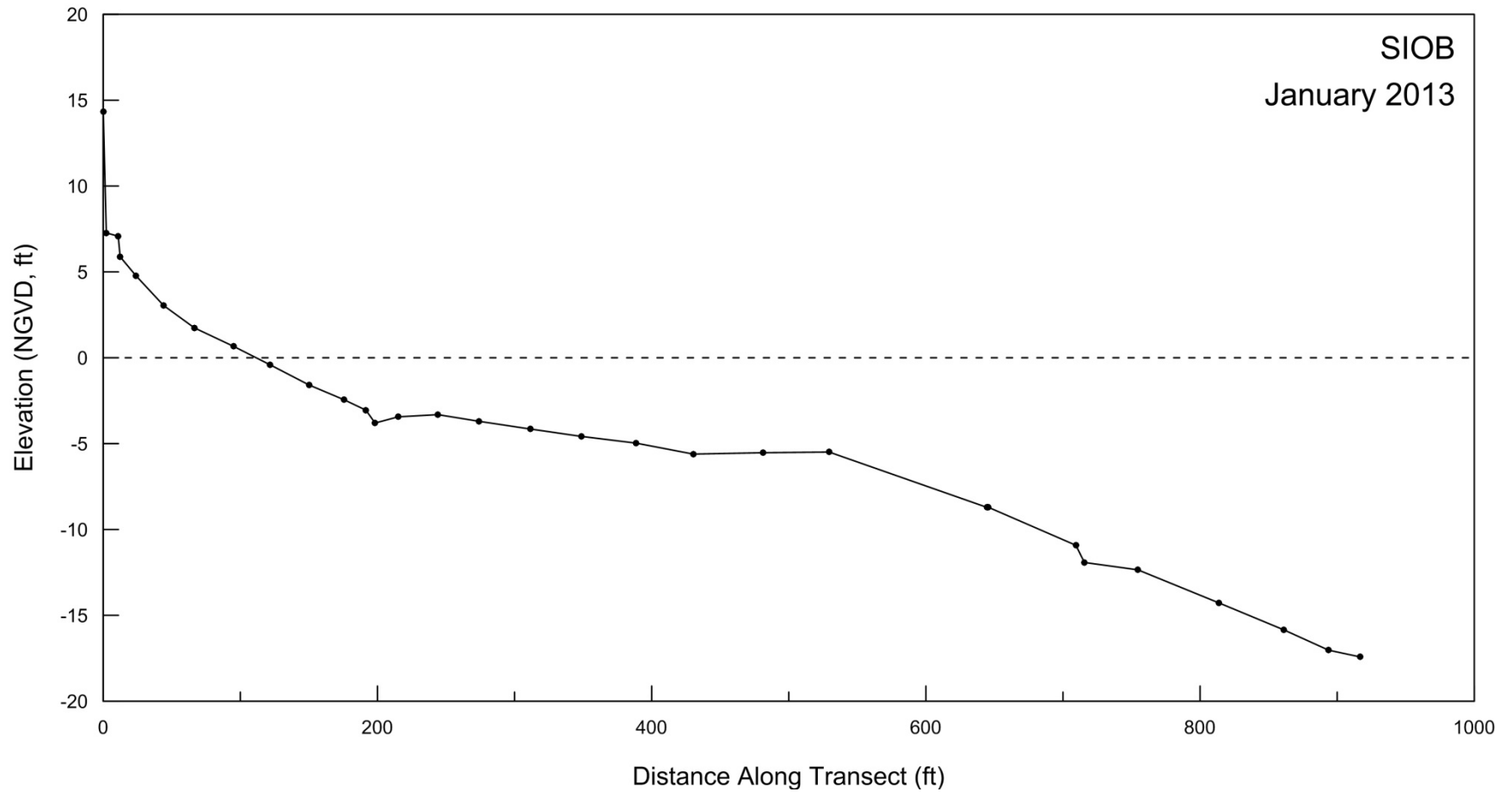
Figure A-6. Beach profile for SIOB surveyed on 23 January 2013.
