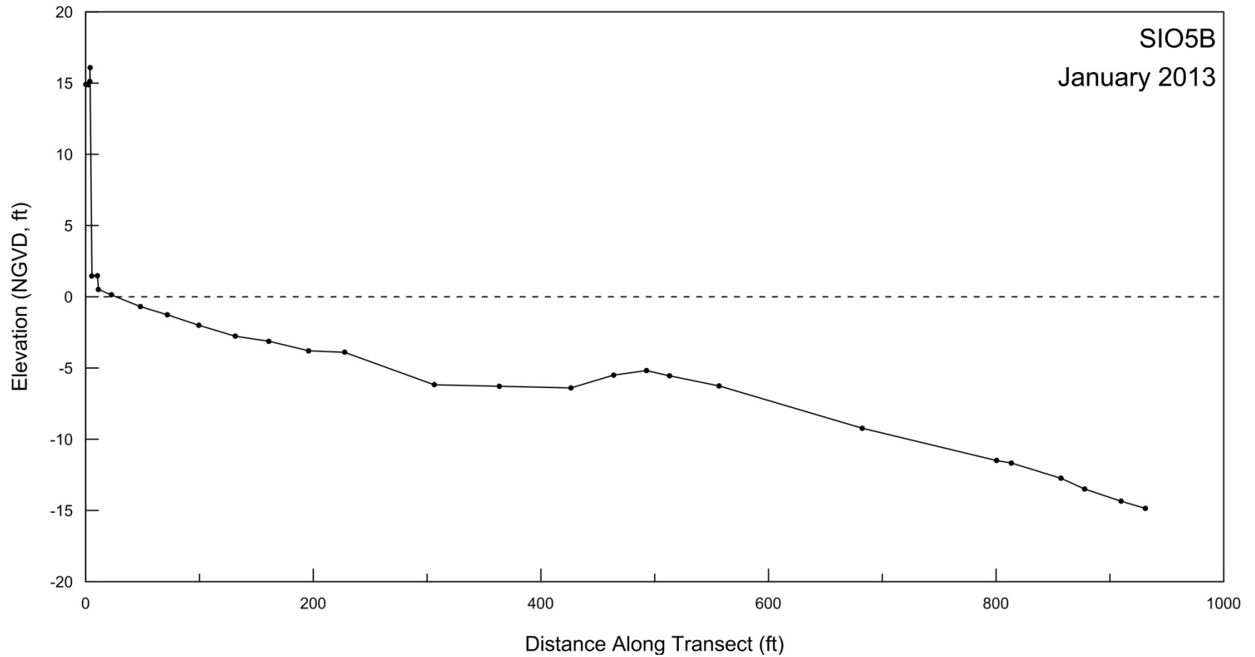
Figure A-3. Beach profile for SIO5B surveyed on 23 January 2013.
