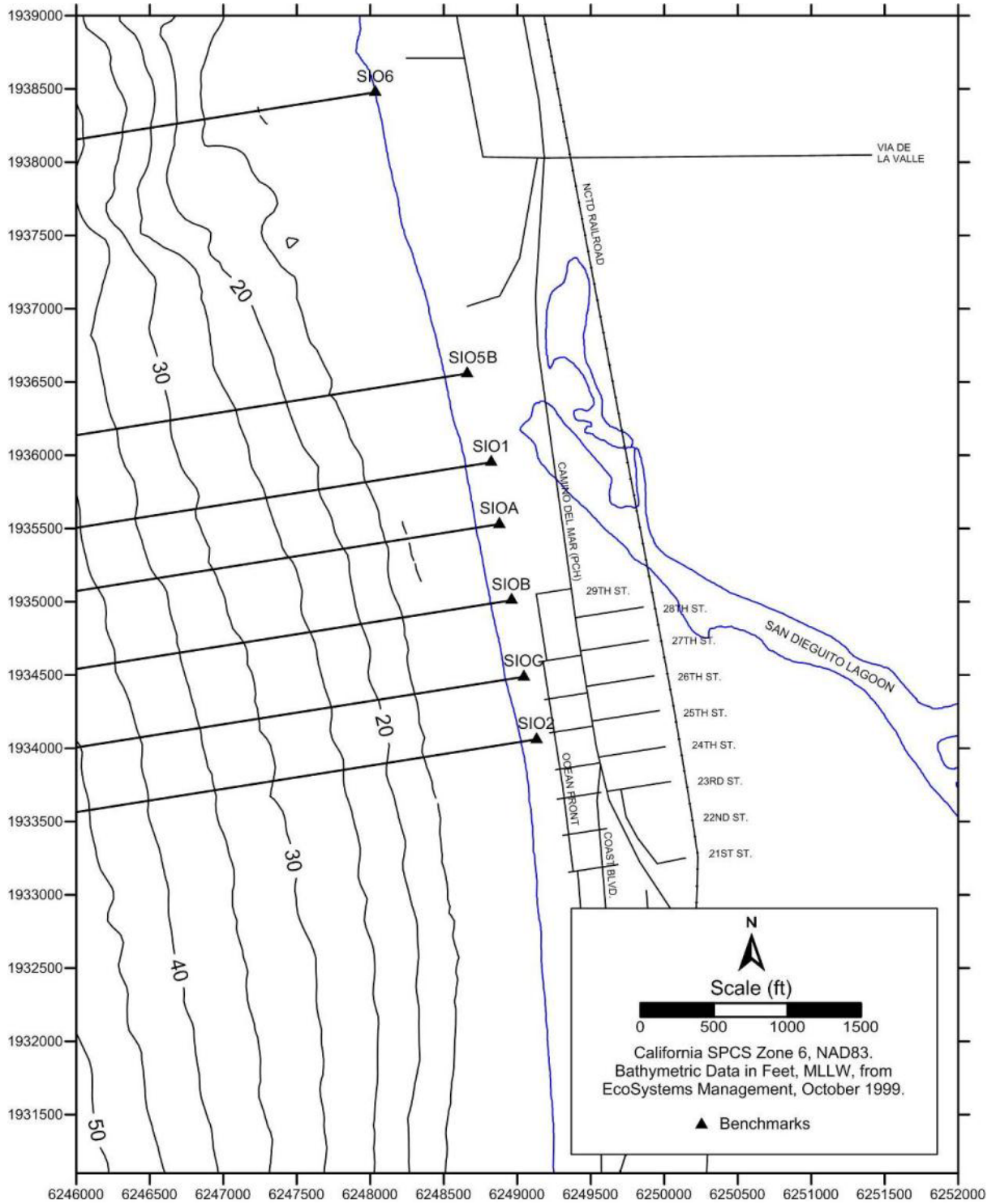
Figure 2. Beach profiles surveyed on 23 January 2013.
