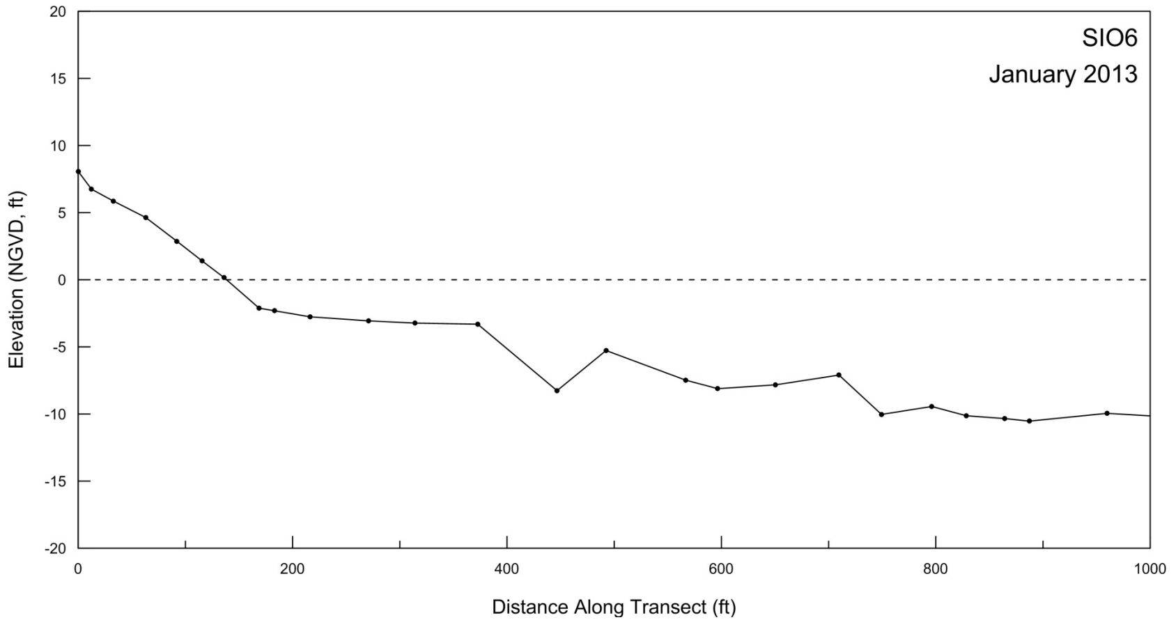
Figure A-4. Beach profile for SIO6 surveyed on 23 January 2013.
