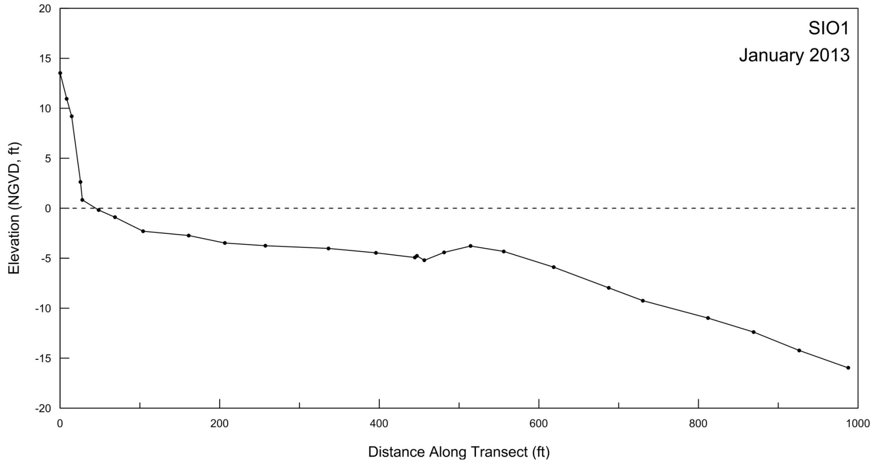
Figure A-1. Beach profile for SIO1 surveyed on 23 January 2013.
