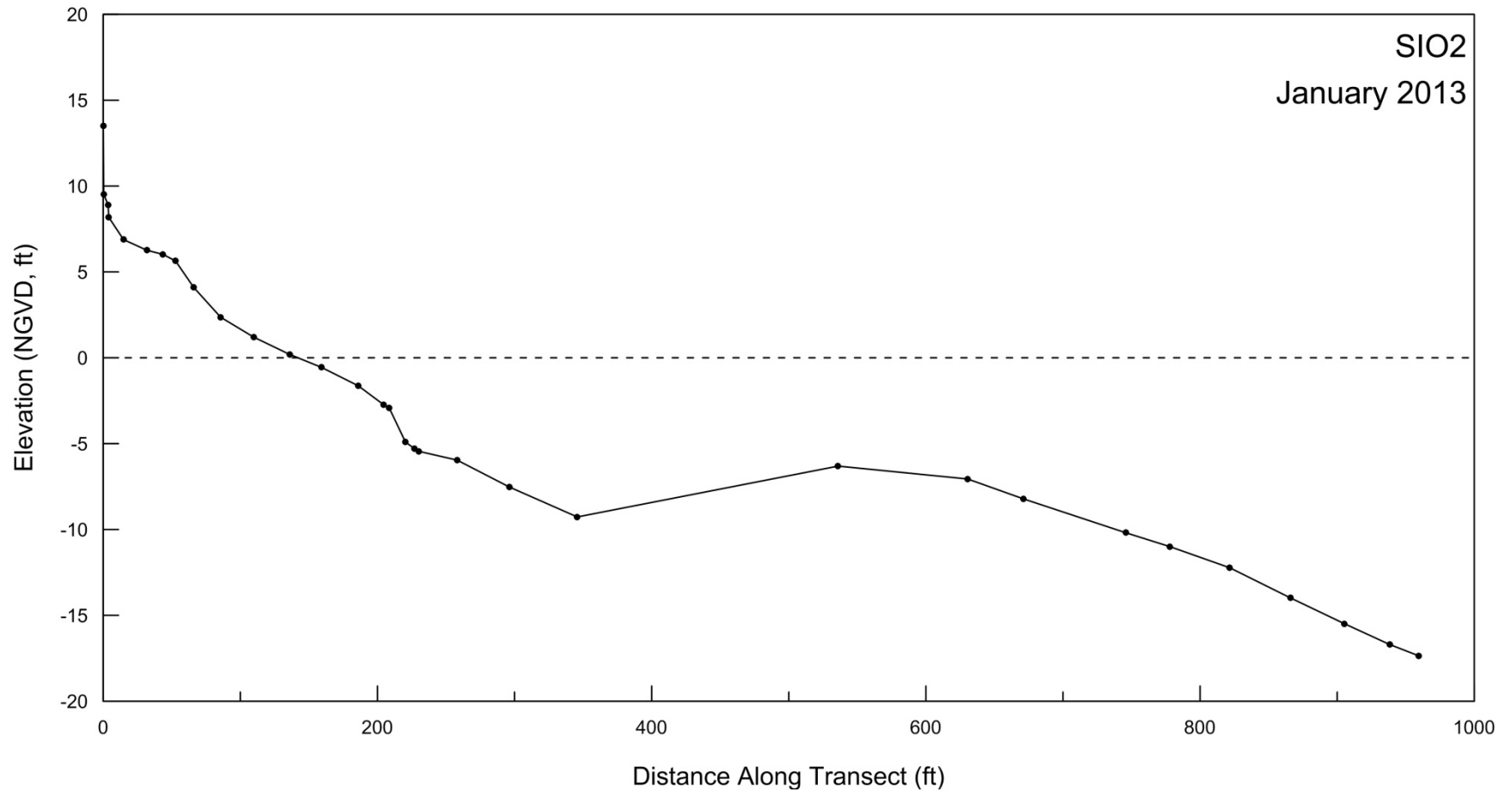
Figure A-2. Beach profile for SIO2 surveyed on 23 January 2013.
