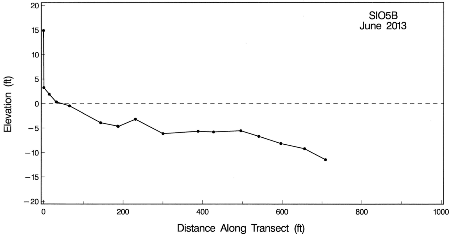
Figure A-3. Beach profile for SIO5B surveyed in June 2013.
