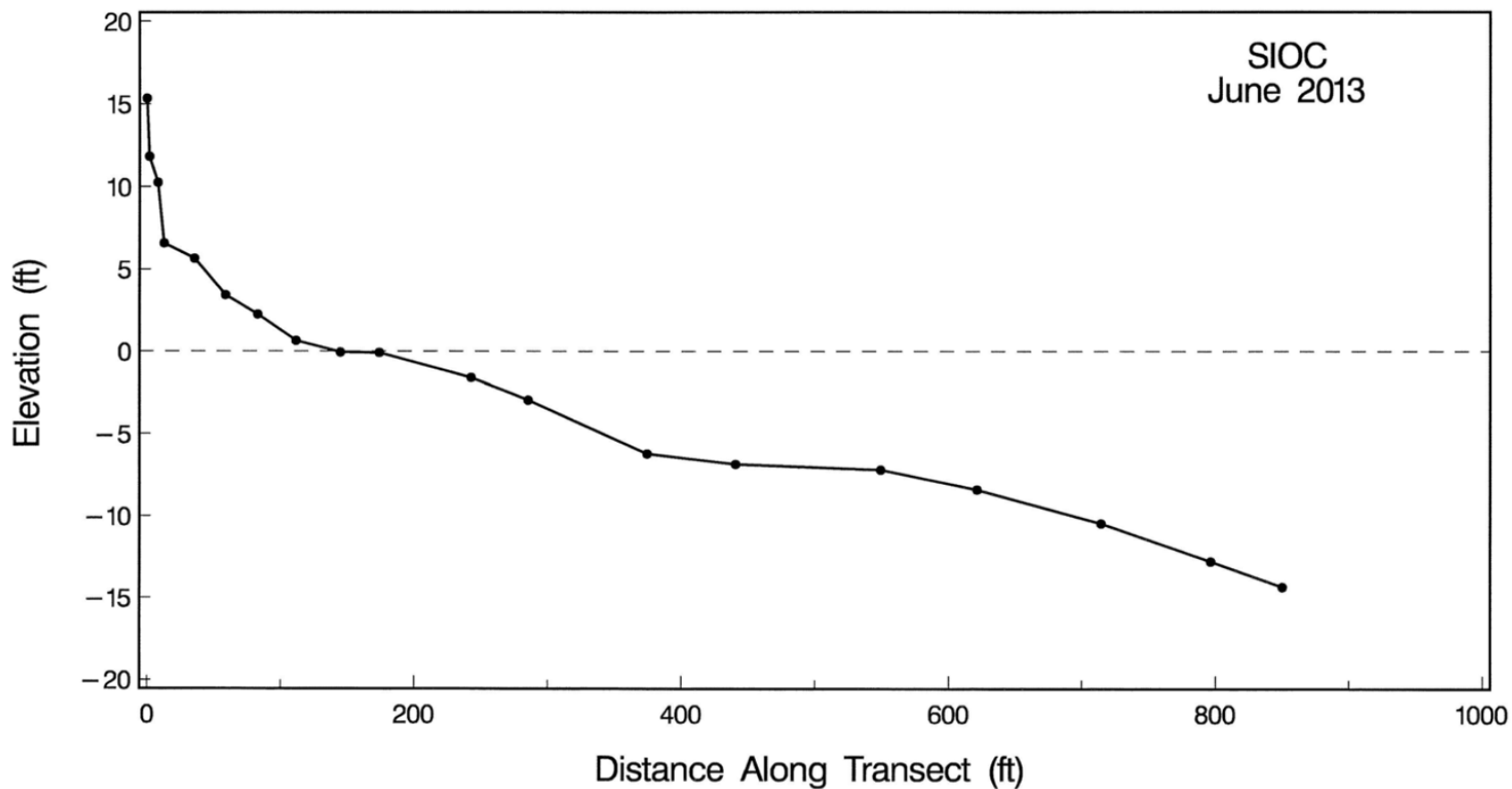
Figure A-7. Beach profile for SIOC surveyed in June 2013.
