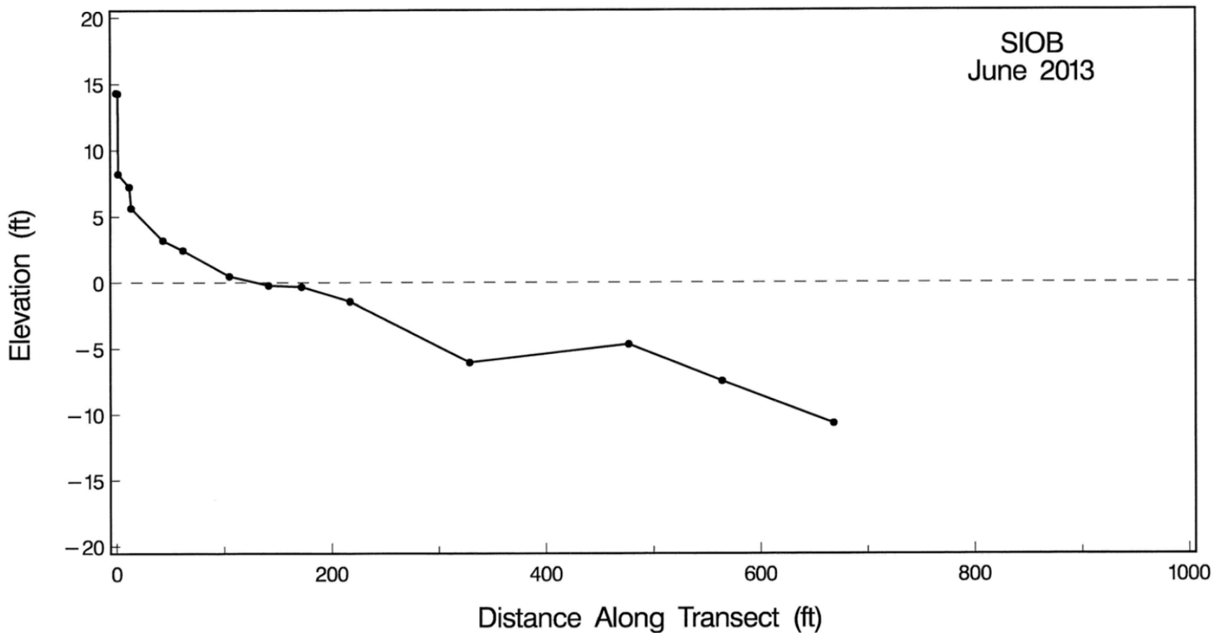
Figure A-6. Beach profile for SIOB surveyed in June 2013.
