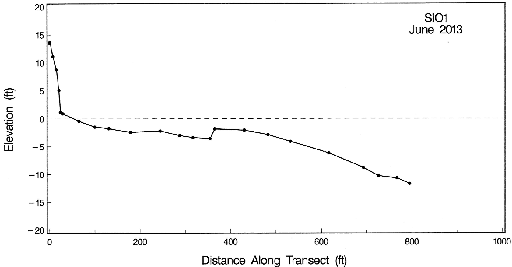
Figure A-1. Beach profile for SIO1 surveyed in June 2013.
