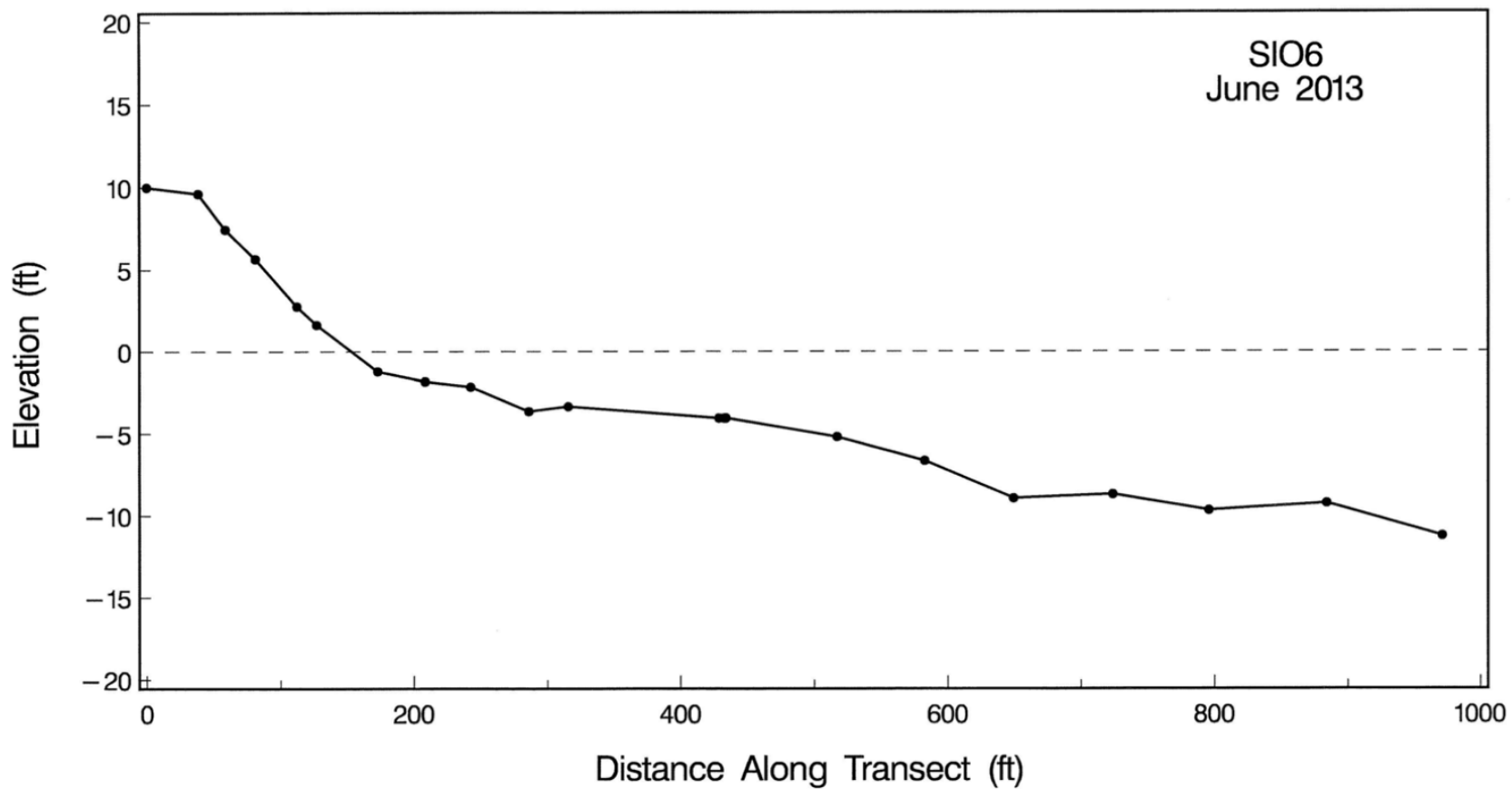
Figure A-4. Beach profile for SIO6 surveyed in June 2013.
