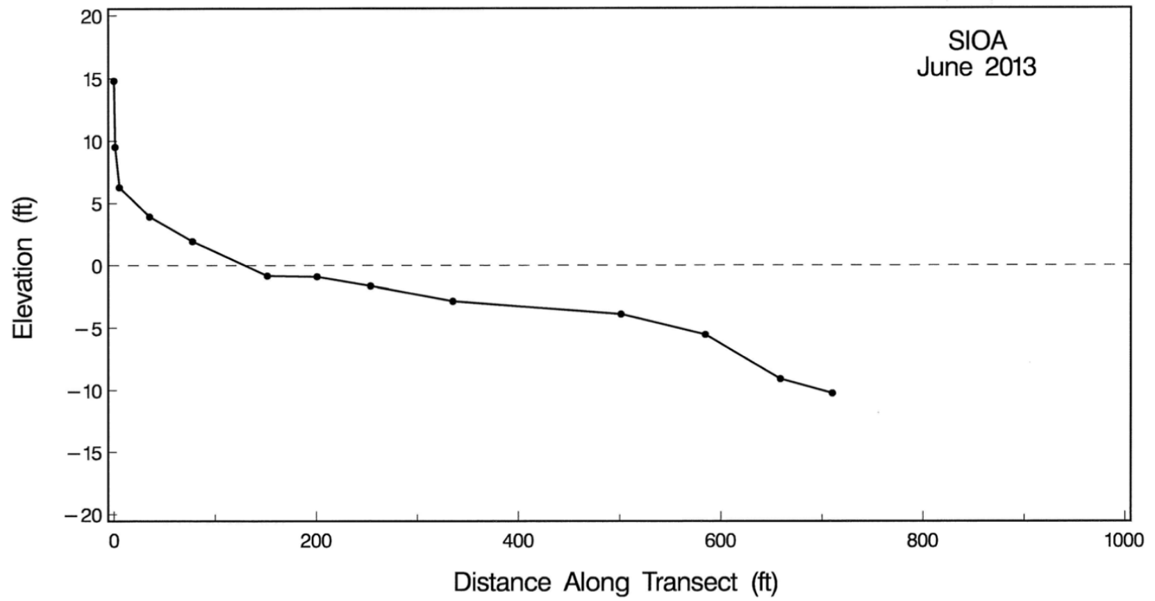
Figure A-5. Beach profile for SIOA surveyed in June 2013.
