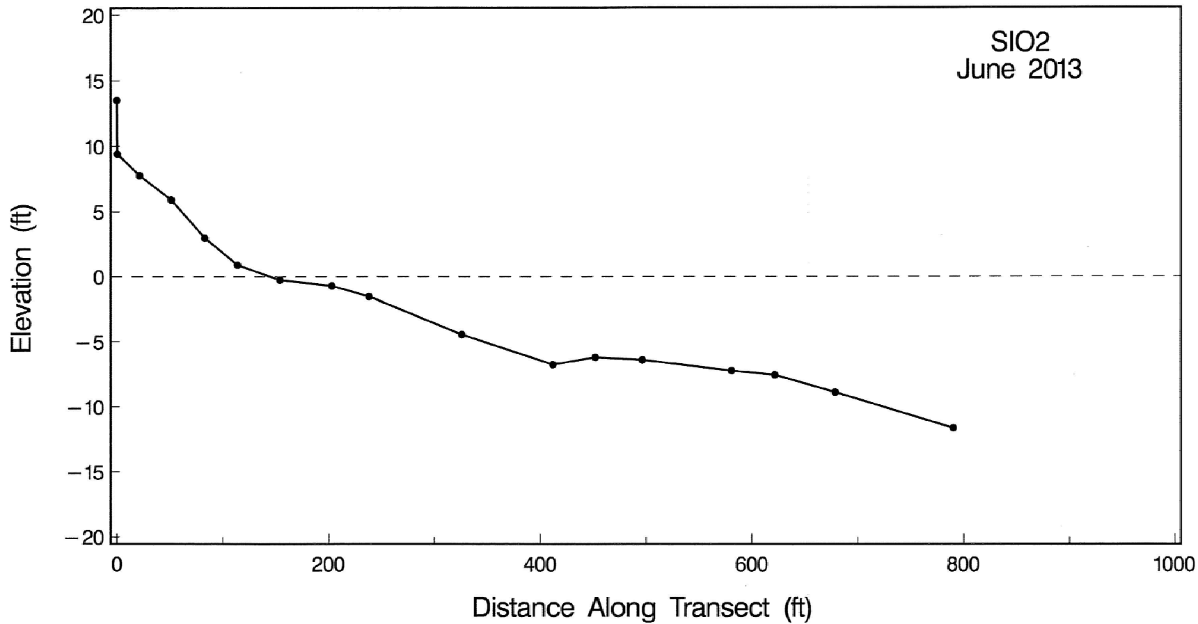
Figure A-2. Beach profile for SIO2 surveyed in June 2013.
